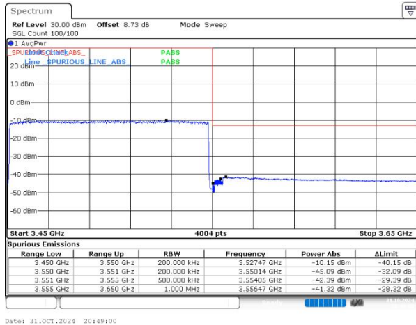
n77(3450-3550) SCS=30kHz DFT_QPSK BW=100MHz HighChannel=633334 RB=270@0
