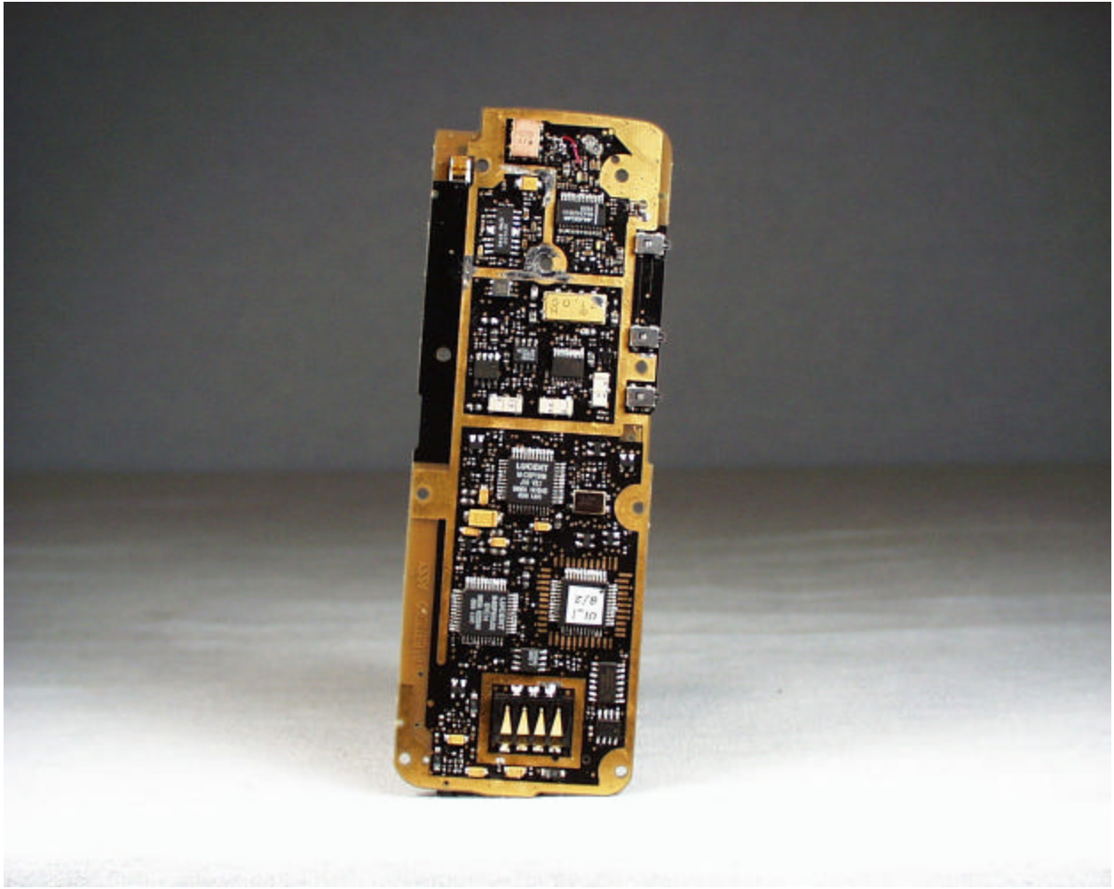
Opposite Side of PCB without Shield Installed (Handset)
