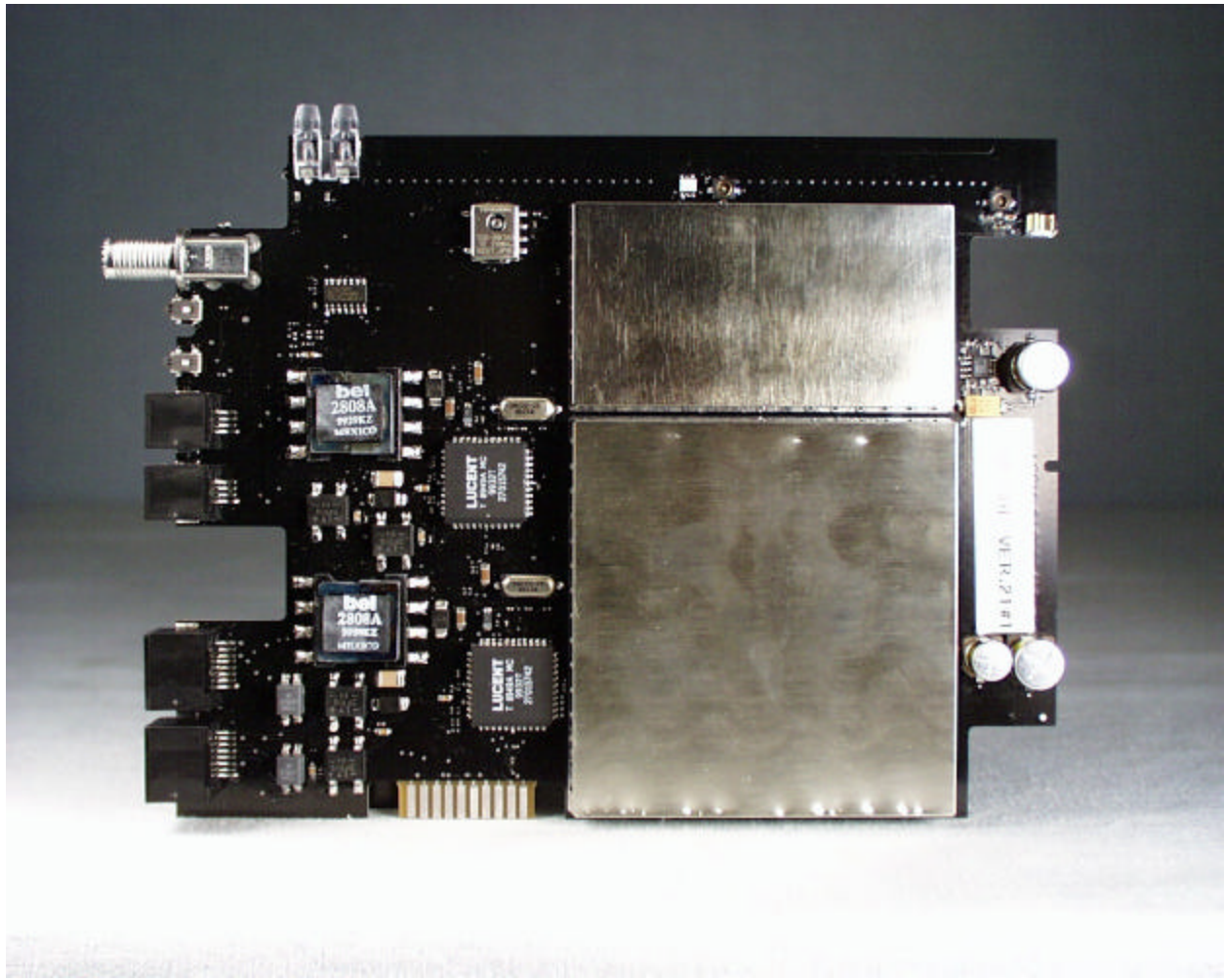
Component Side of DCM with Shields Installed PCB (Base)
