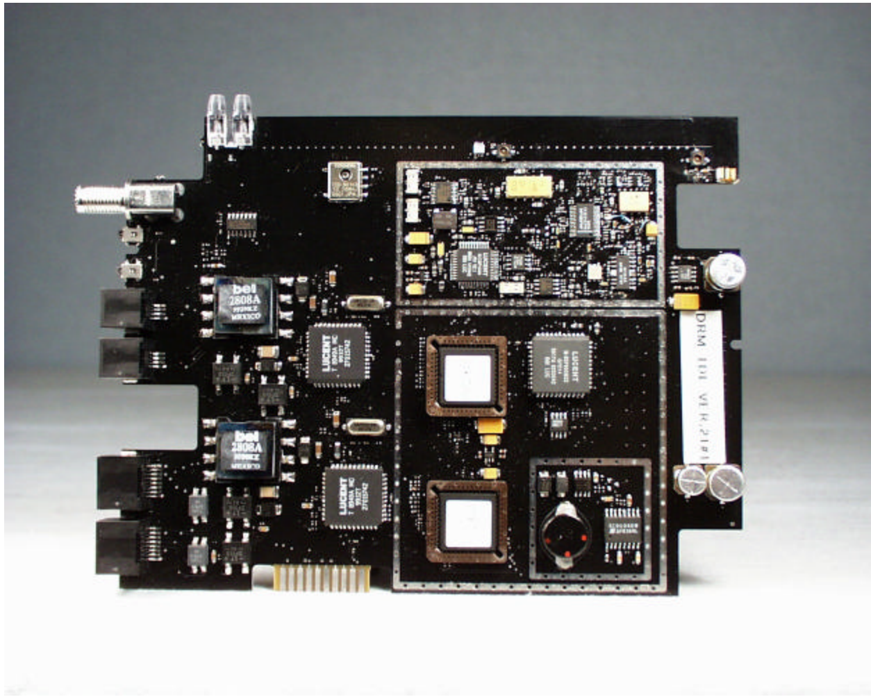
Component Side of DCM PCB without Shields Installed (Base)
