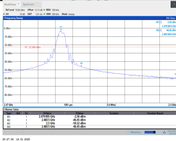
SRD_Ant1_High_2480
