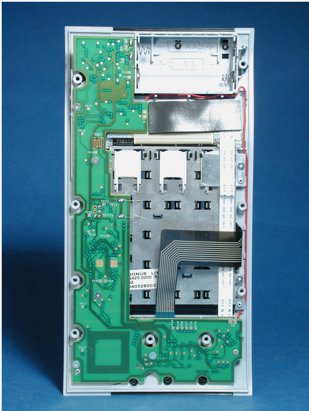
Photograph 1: Y-RX43 internal view
