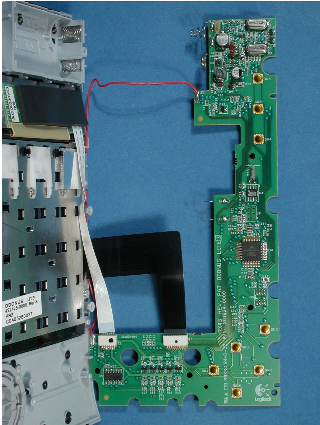
Photograph 2: Y-RX43 internal view (PCB)
