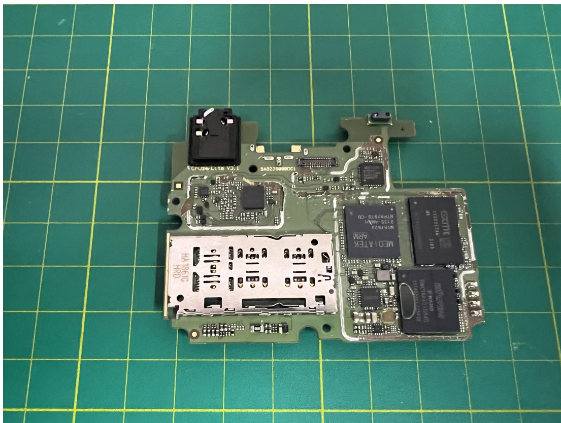
6165H Mobile Phone Disassembly
