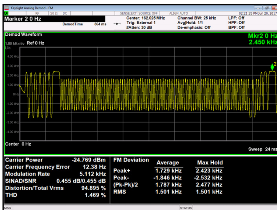
Figure 22 - 162.025 MHz - 01010101
