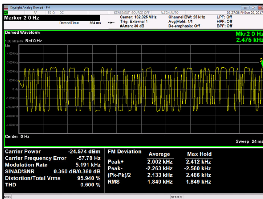
Figure 24- 162.025 MHz - PRBS
