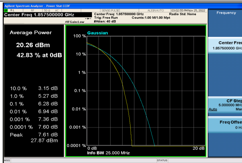
Band2-15MHz-64QAM-18675-75RB#0
