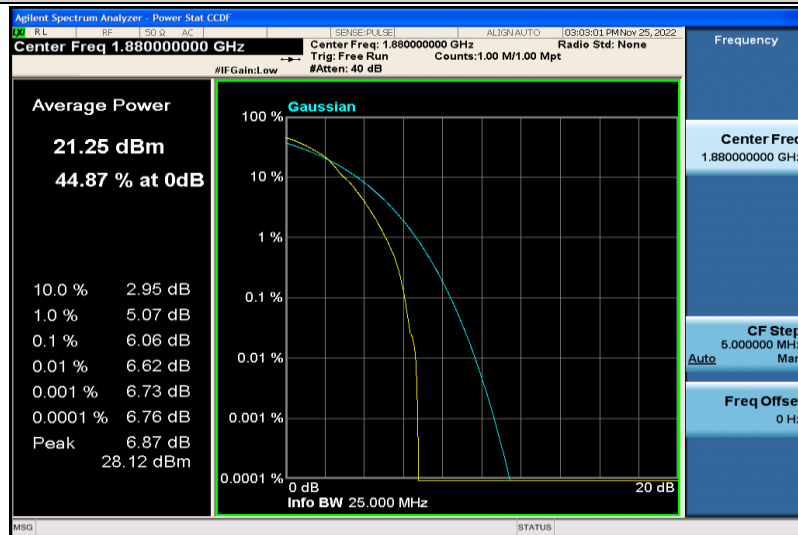
Band2-15MHz-64QAM-18900-1RB#0
