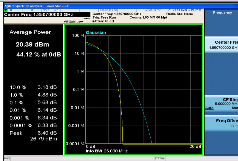
Band2-1.4MHz-64QAM-18607-6RB#0
