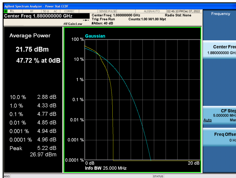
Band2-1.4MHz-16QAM-18900-1RB#0
