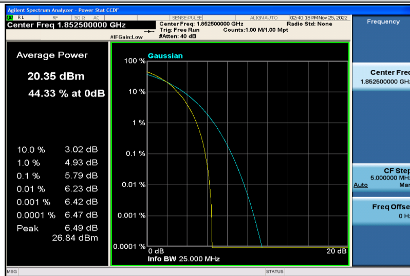
Band2-5MHz-64QAM-18625-25RB#0
