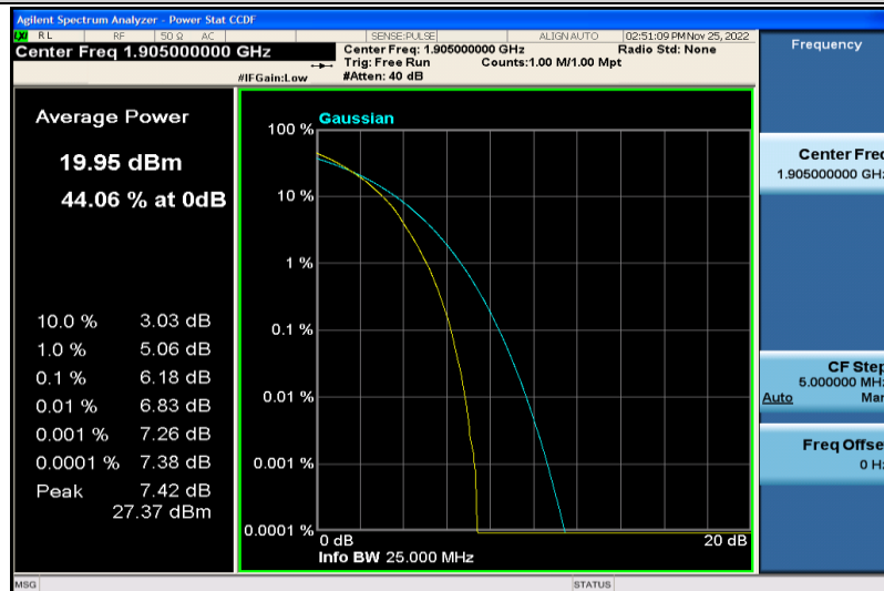
Band2-10MHz-64QAM-19150-50RB#0
