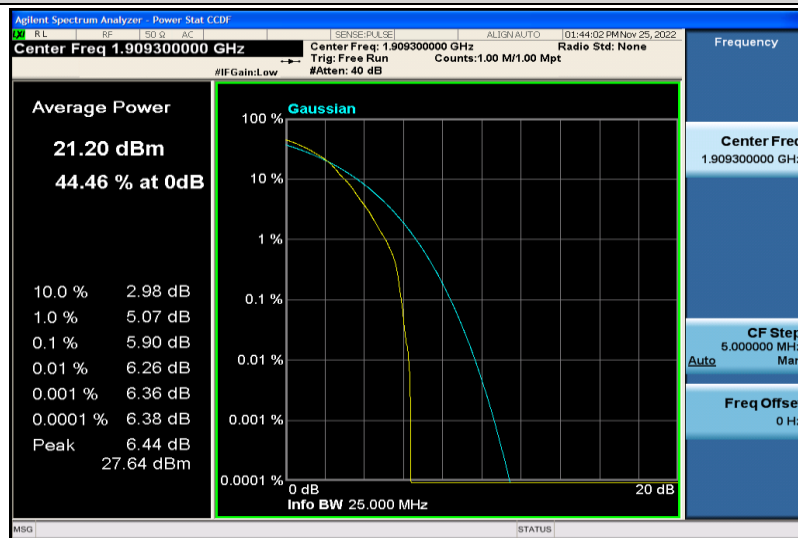
Band2-1.4MHz-64QAM-19193-1RB#0
