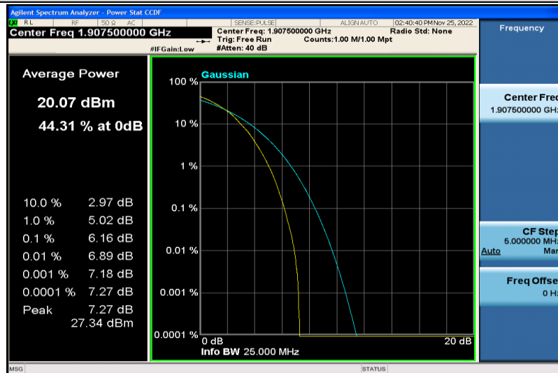
Band2-5MHz-64QAM-19175-25RB#0
