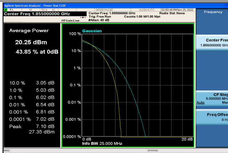
Band2-10MHz-64QAM-18650-50RB#0
