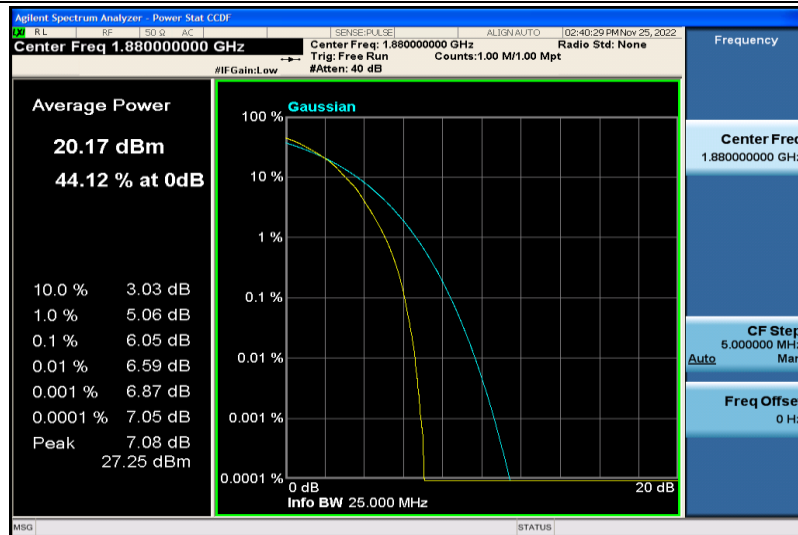
Band2-5MHz-64QAM-18900-25RB#0
