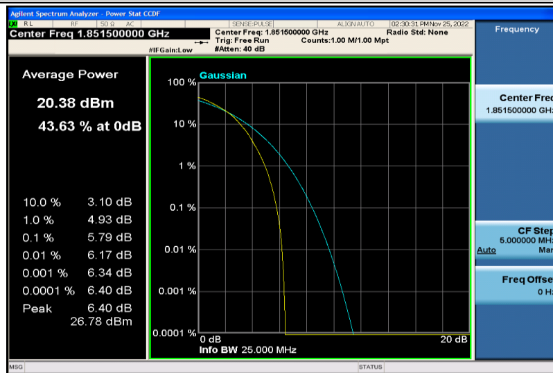
Band2-3MHz-64QAM-18615-15RB#0
