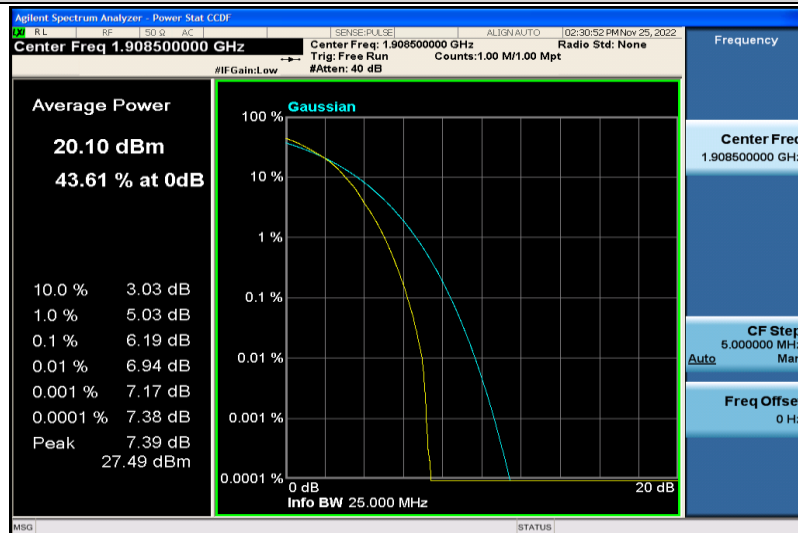
Band2-3MHz-64QAM-19185-15RB#0
