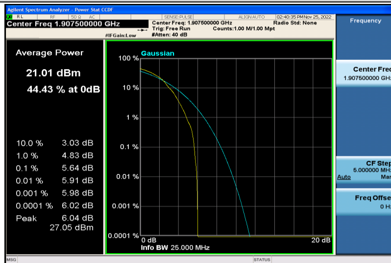
Band2-5MHz-64QAM-19175-1RB#0
