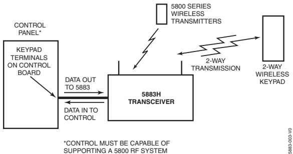
Figure 1: Block Diagram
