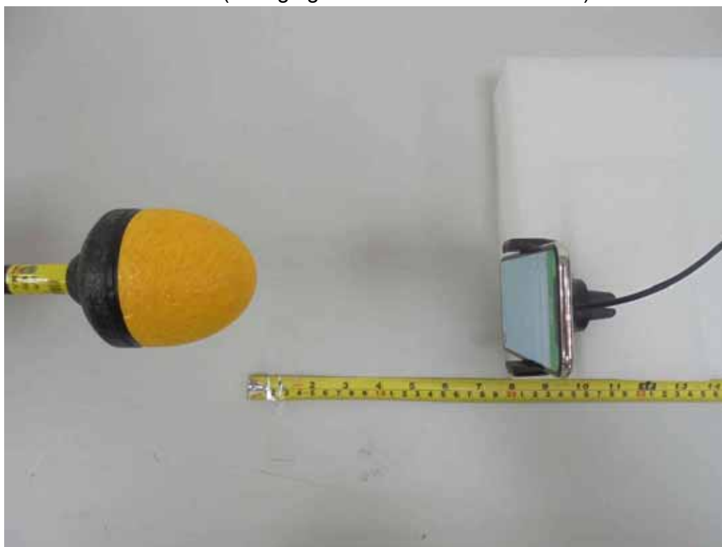
E-Field (Charging Mode with iPhone - Z-axis)
