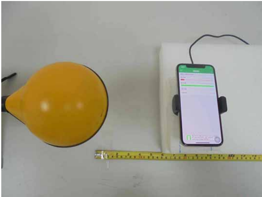
H-Field (Charging Mode with iPhone - Left)
