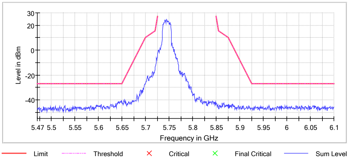
Graph 4: 20 MHz N Mode Low
