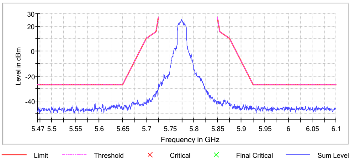
Graph 5: 20 MHz N Mode Mid
