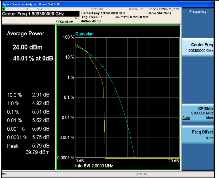
Band2-1.4MHz-16QAM-19193-1RB#0-PASS
