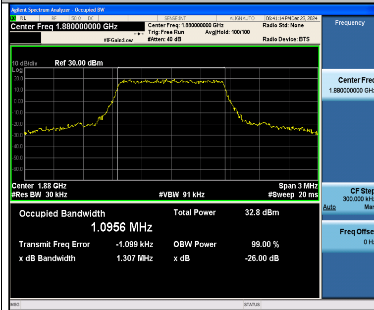
Band2-1.4MHz-QPSK-18900-6RB#0-PASS
