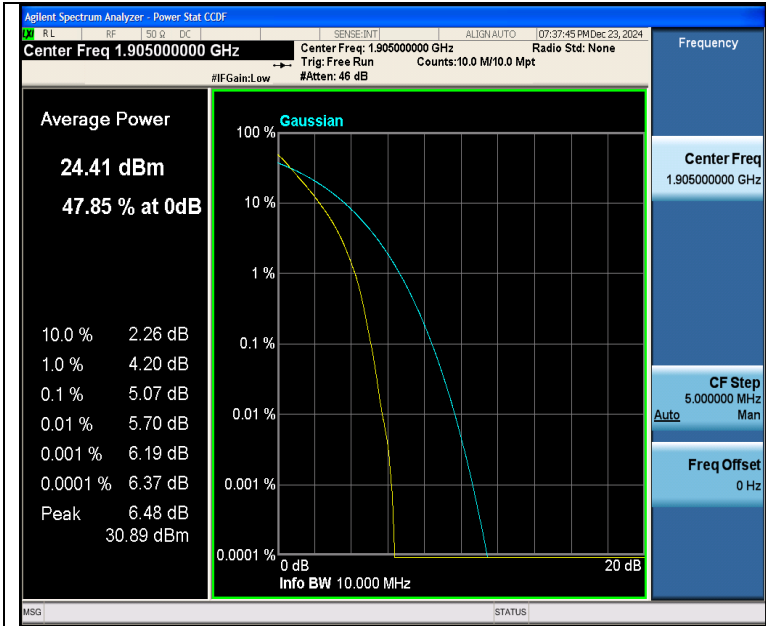
Band2-10MHz-QPSK-19150-50RB#0-PASS
