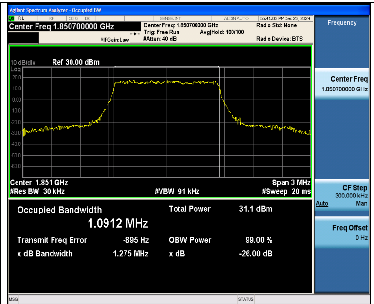
Band2-1.4MHz-16QAM-18607-6RB#0-PASS
