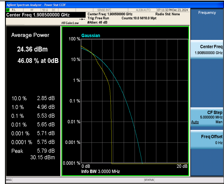
Band2-3MHz-16QAM-19185-1RB#0-PASS
