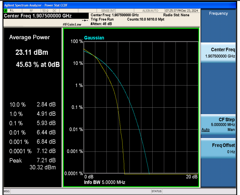
Band2-5MHz-16QAM-19175-25RB#0-PASS
