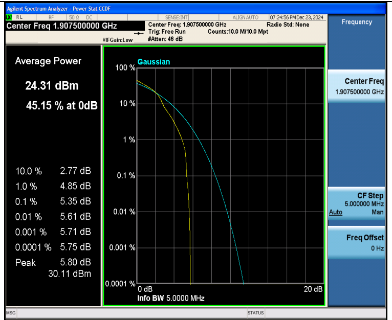
Band2-5MHz-16QAM-19175-1RB#0-PASS
