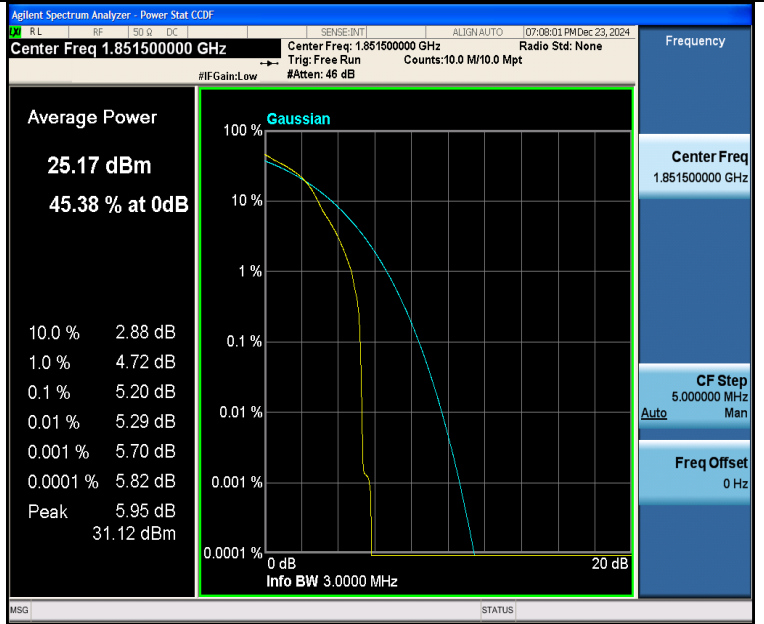
Band2-3MHz-16QAM-18615-1RB#0-PASS
