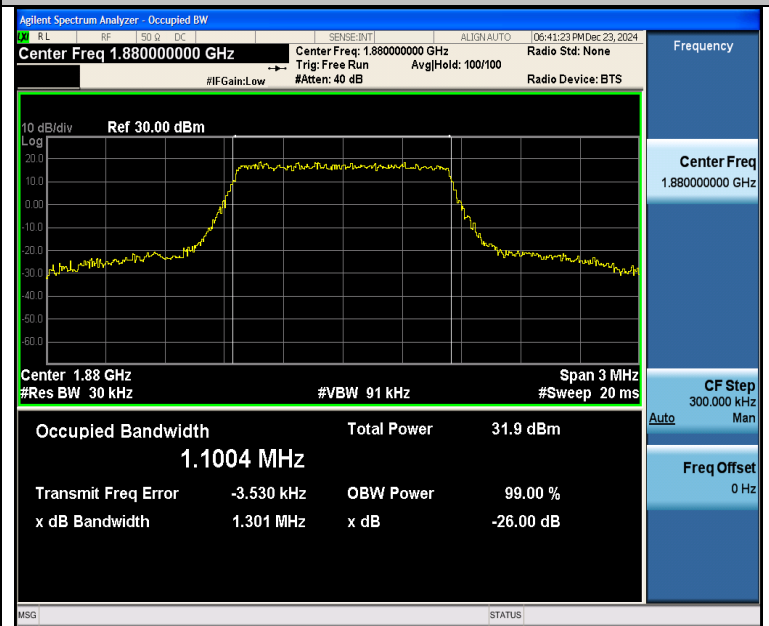
Band2-1.4MHz-16QAM-18900-6RB#0-PASS
