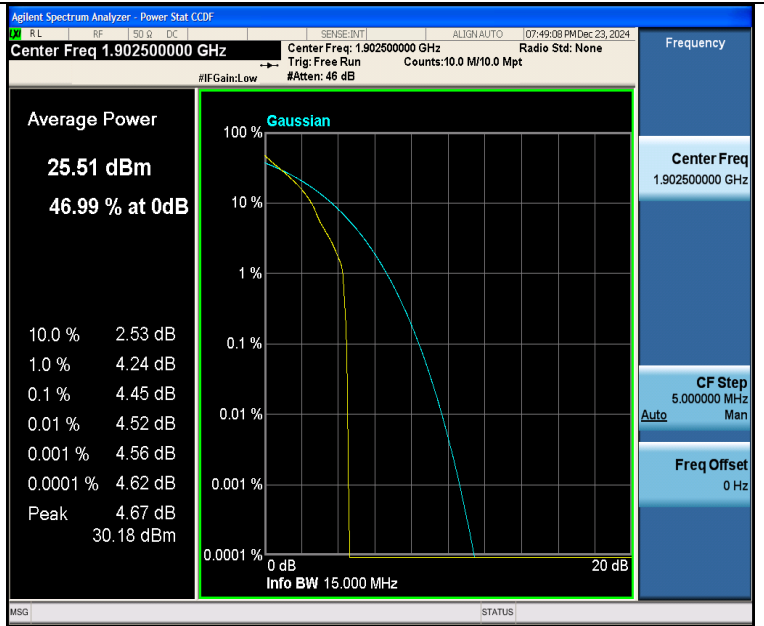
Band2-15MHz-QPSK-19125-1RB#0-PASS
