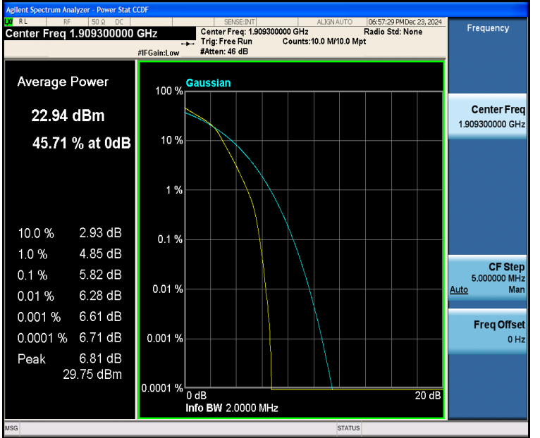
Band2-1.4MHz-16QAM-19193-6RB#0-PASS
