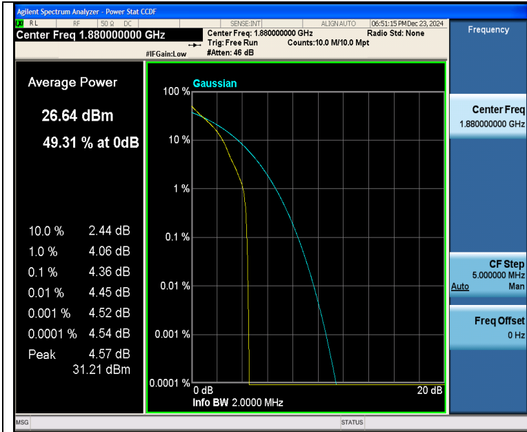
Band2-1.4MHz-QPSK-18900-1RB#0-PASS
