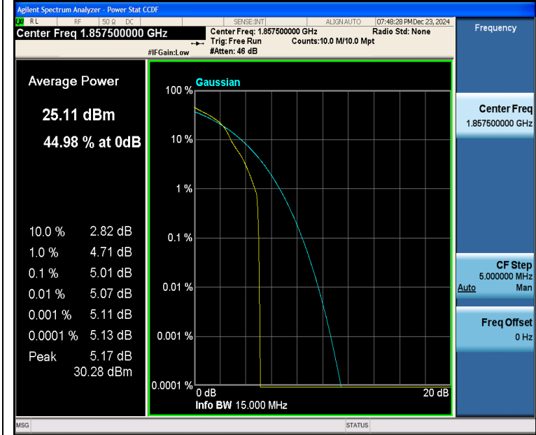
Band2-15MHz-16QAM-18675-1RB#0-PASS
