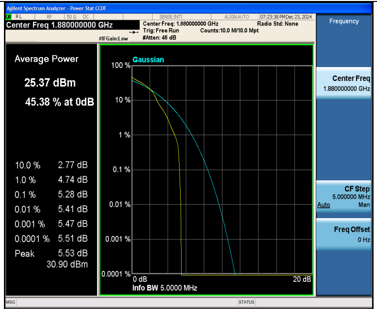
Band2-5MHz-16QAM-18900-1RB#0-PASS
