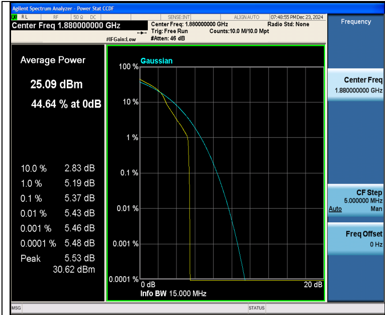
Band2-15MHz-16QAM-18900-1RB#0-PASS
