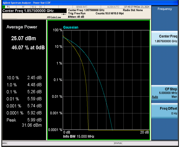
Band2-15MHz-QPSK-18675-75RB#0-PASS
