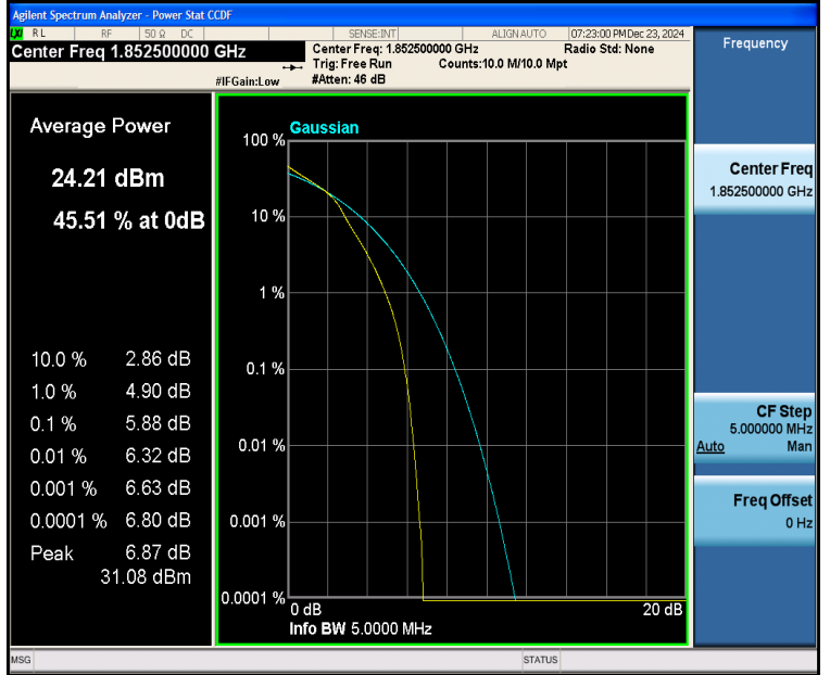
Band2-5MHz-16QAM-18625-25RB#0-PASS
