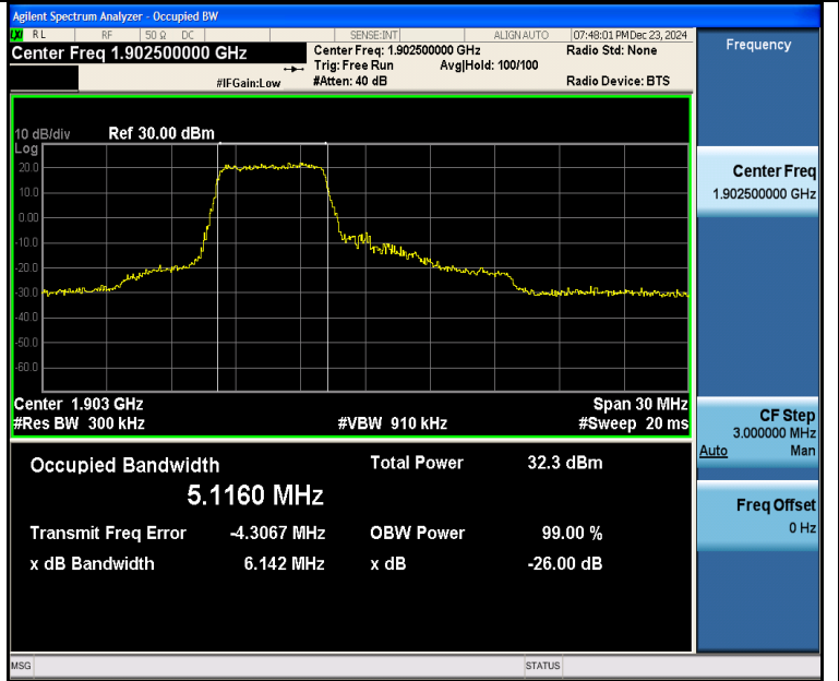
Band2-15MHz-16QAM-19125-27RB#0-PASS
