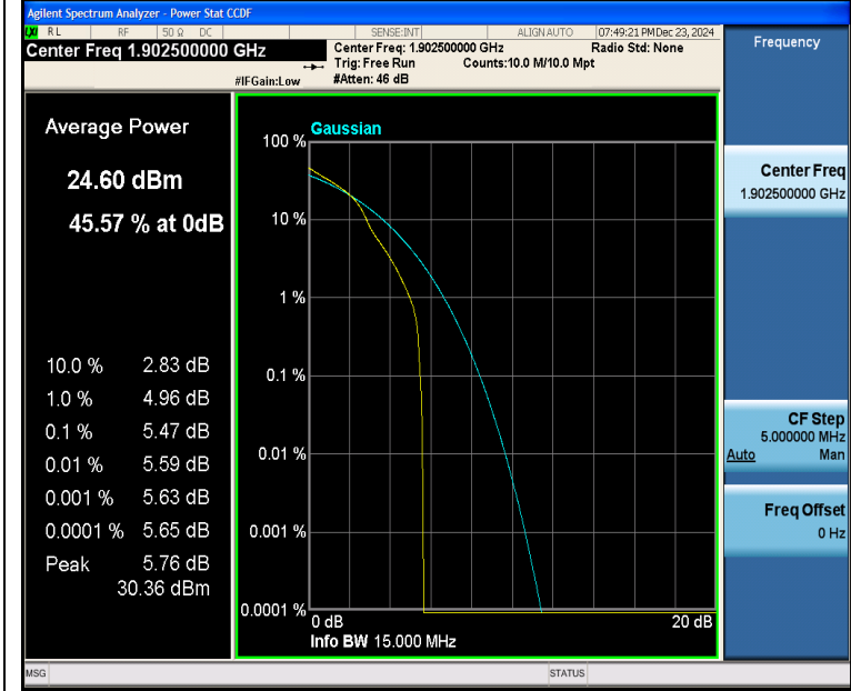
Band2-15MHz-16QAM-19125-1RB#0-PASS
