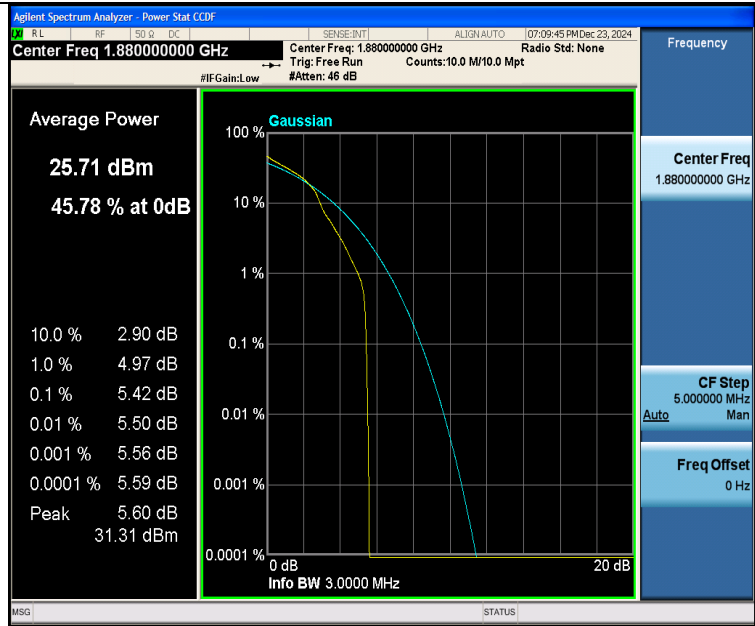
Band2-3MHz-16QAM-18900-1RB#0-PASS
