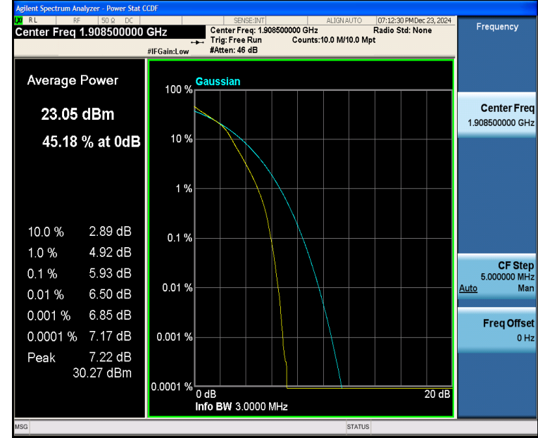
Band2-3MHz-16QAM-19185-15RB#0-PASS
