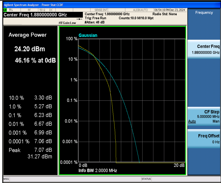
Band2-1.4MHz-16QAM-18900-6RB#0-PASS
