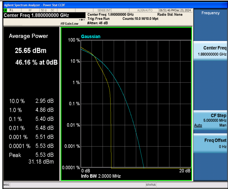
Band2-1.4MHz-16QAM-18900-1RB#0-PASS
