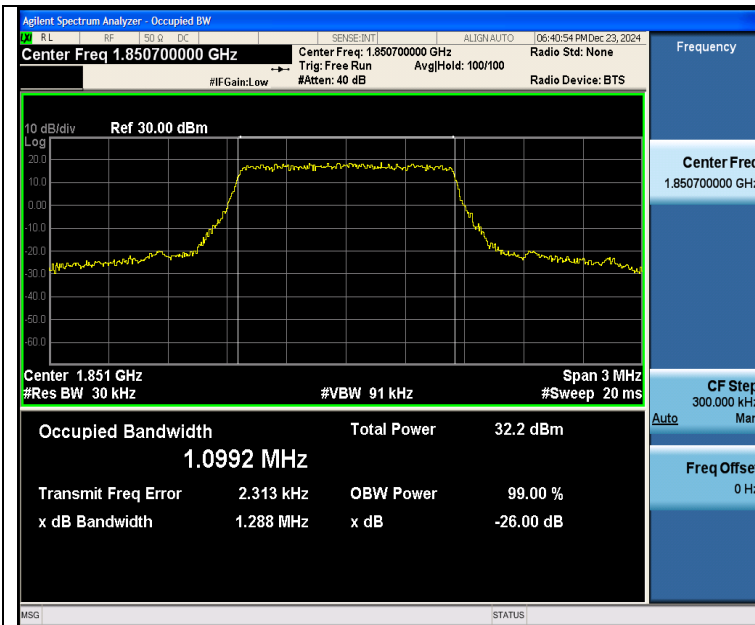
Band2-1.4MHz-QPSK-18607-6RB#0-PASS
