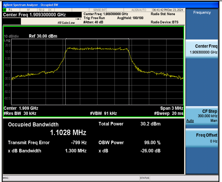
Band2-1.4MHz-16QAM-19193-6RB#0-PASS
