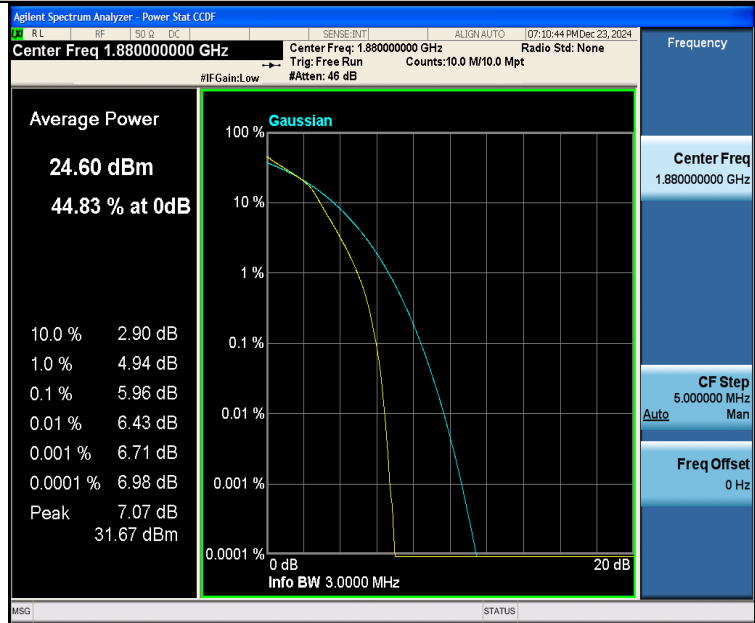
Band2-3MHz-16QAM-18900-15RB#0-PASS
