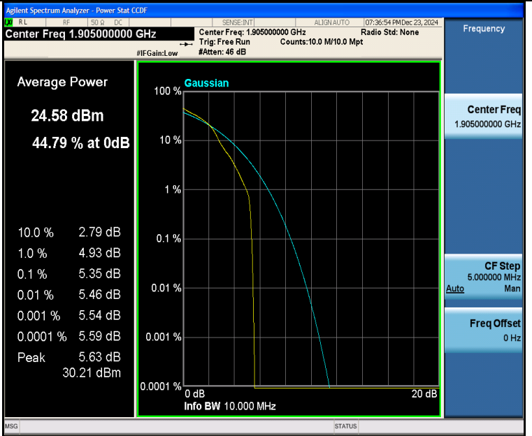
Band2-10MHz-16QAM-19150-1RB#0-PASS
