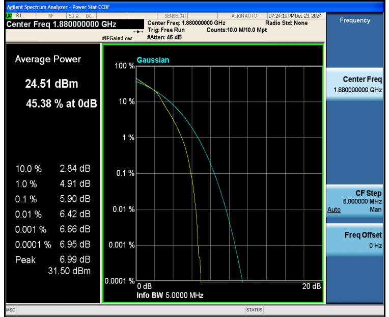
Band2-5MHz-16QAM-18900-25RB#0-PASS
