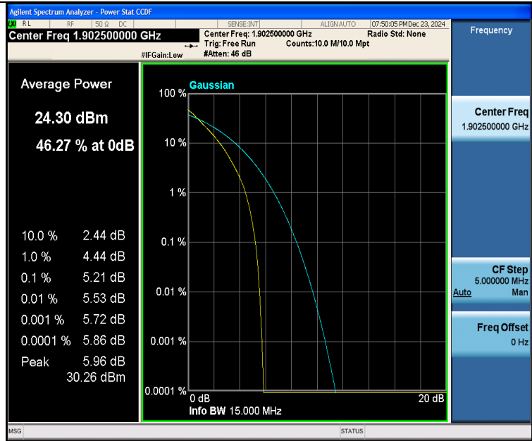
Band2-15MHz-QPSK-19125-75RB#0-PASS
