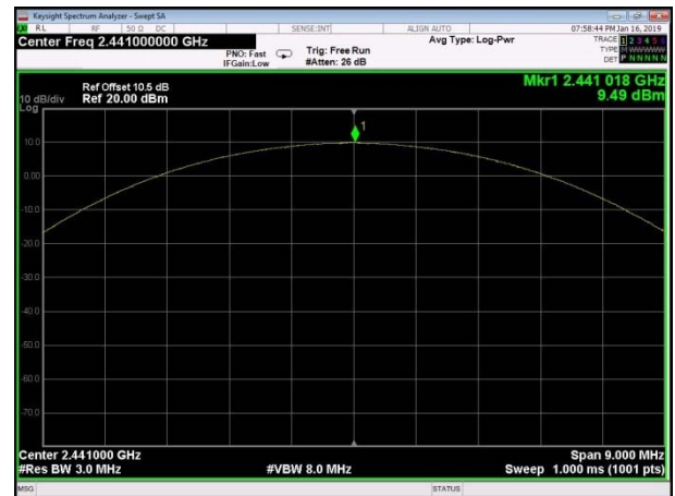
Output Power: 8DPSK,2441MHz,3DH5
