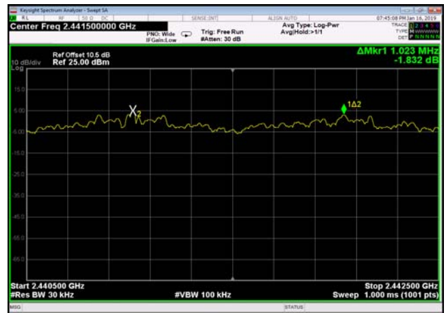
8DPSK,Hopping3DH5,2440.5~2442.5
