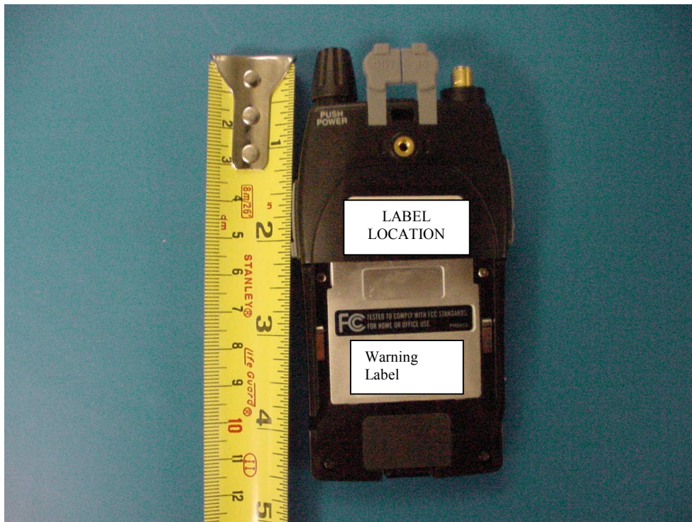
PHOTOGRAPH 3: LABEL LOCATION
