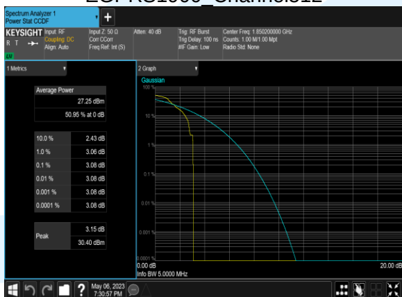
EGPRS1900 Channel512
