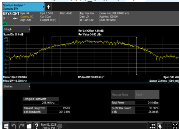
EGPRS850_Channel128
