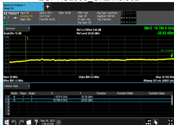
EGPRS1900 Channel661
