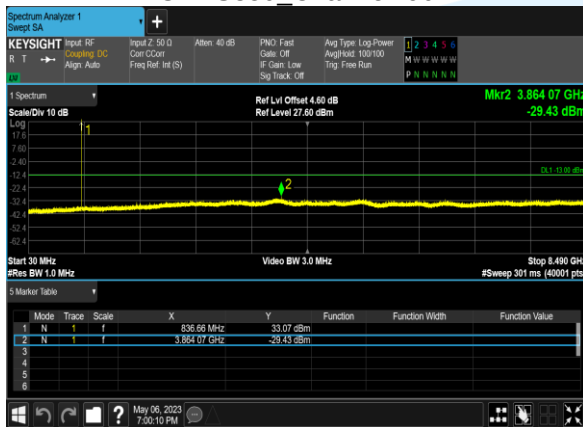
GPRS850_Channel190
