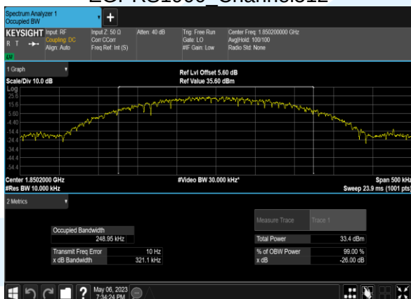
EGPRS1900 Channel512
