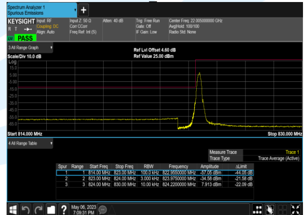
EGPRS850_Channel128
