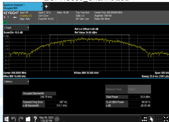
EGPRS850_Channel251
