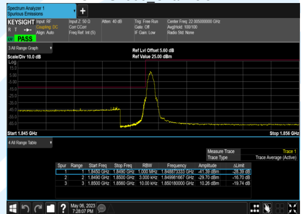
EGPRS1900 Channel512
