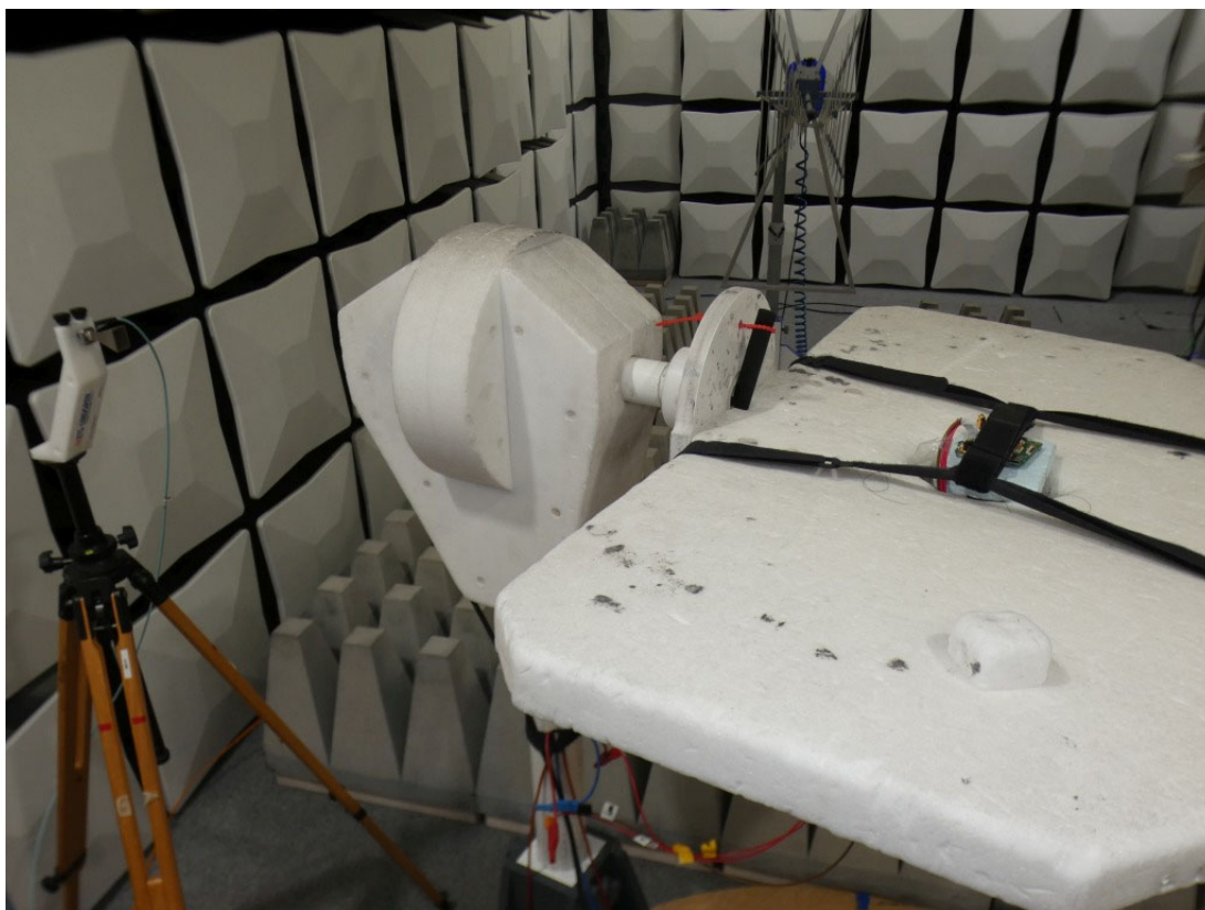
Photo 4: Test setup for radiated measurements above 26 GHz
