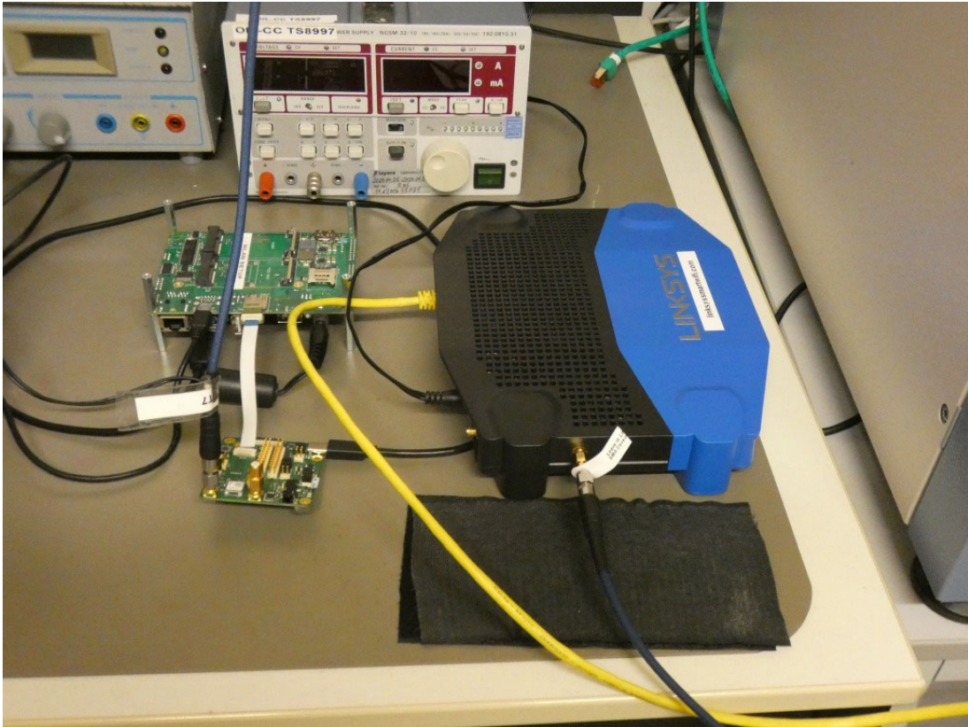
Photo 7: Test setup for conducted measurements EUT Detail DFS
