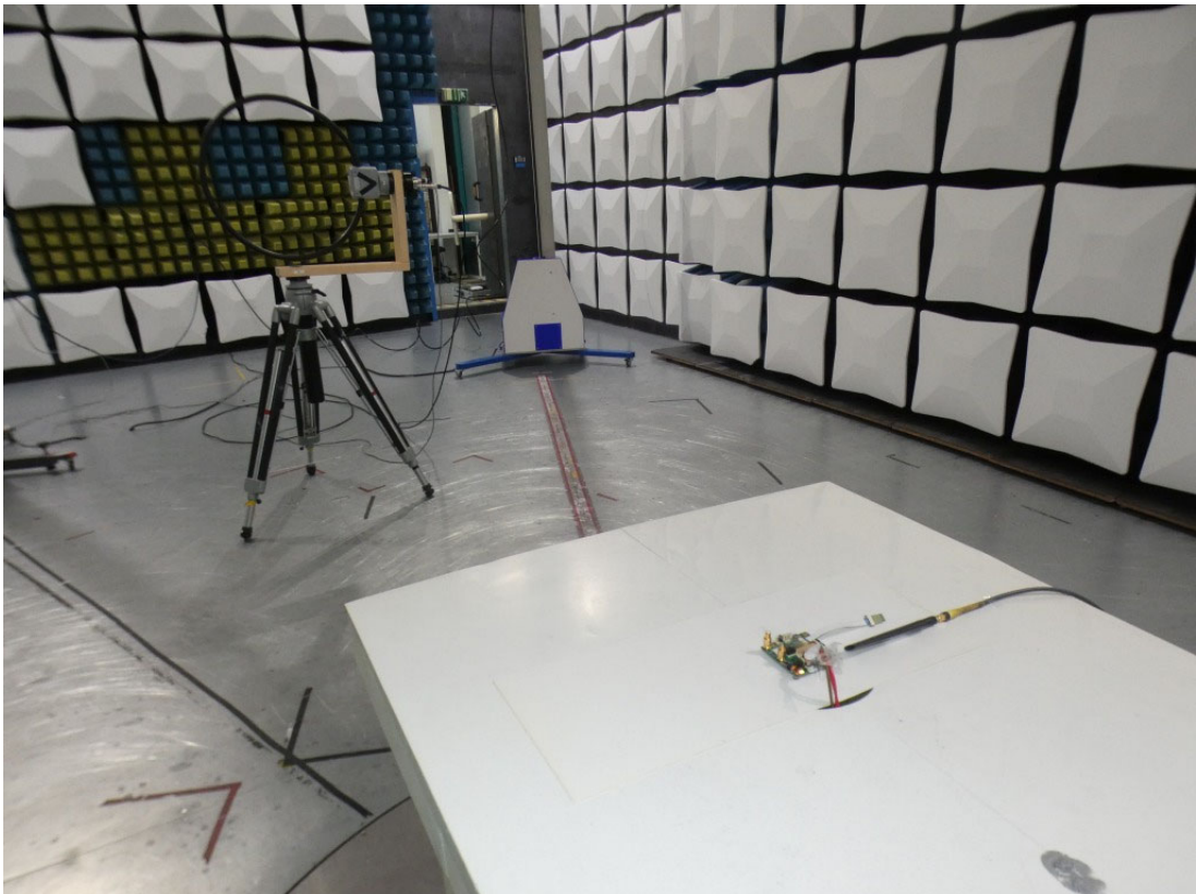
Photo 1: Test setup for H-Field measurements
