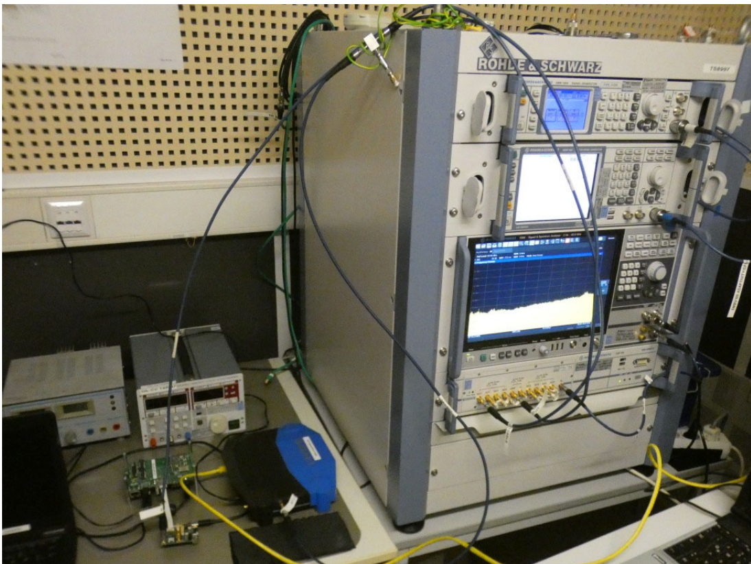
Photo 8: Test Setup for DFS
