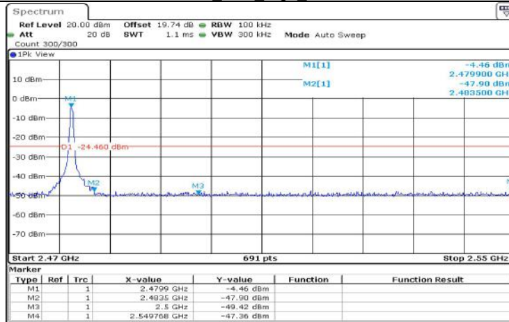
DH1_Ant1_High_2480
