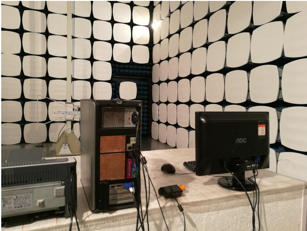
By PC Radiated Emission Below 1GHz
