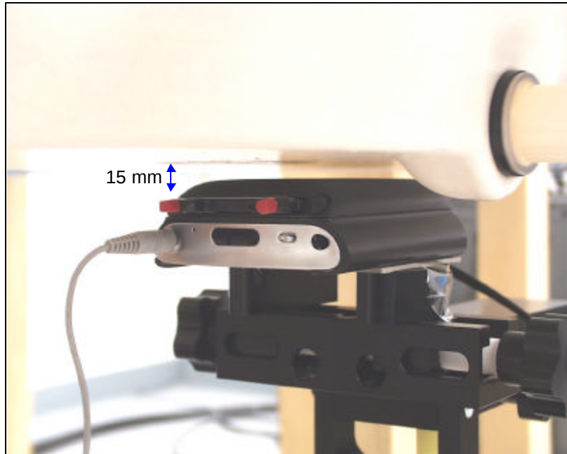
EUT Set-up configuration 4
