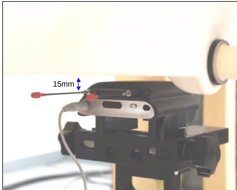
EUT Set-up configuration 3
