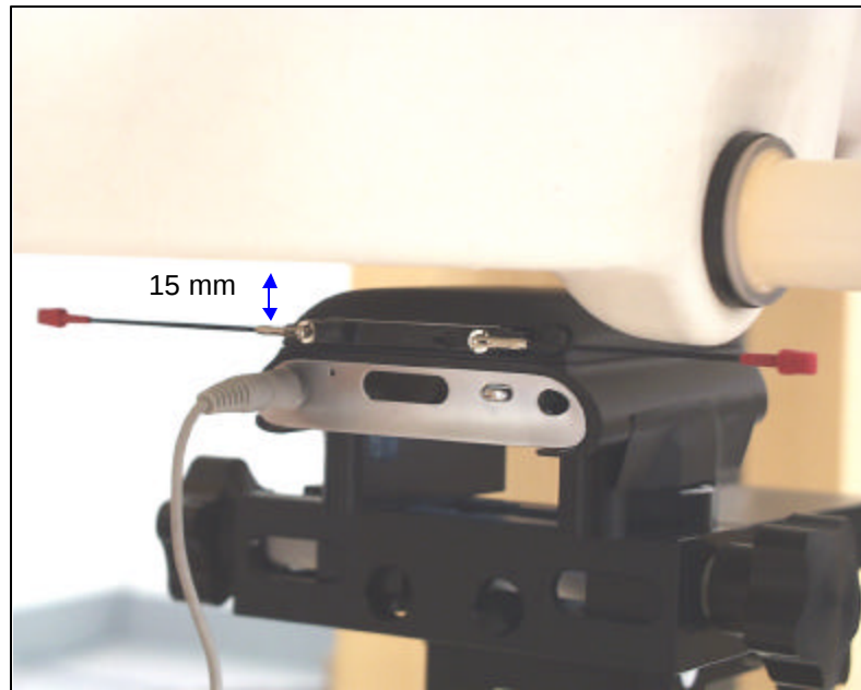
EUT Set-up configuration 2
