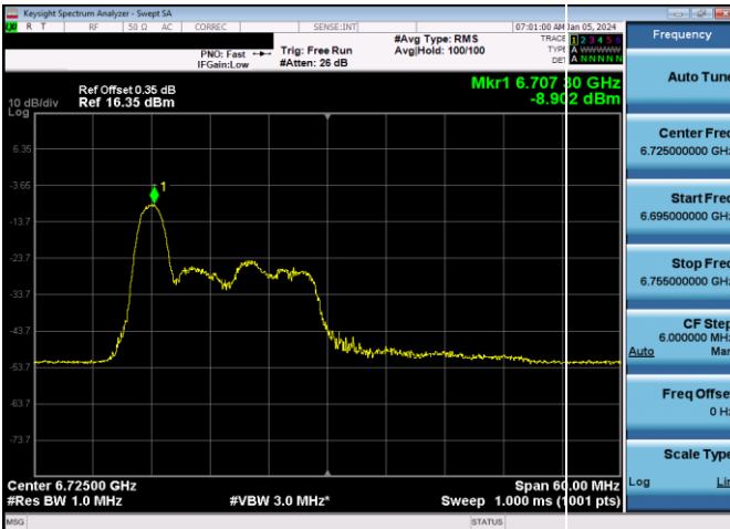
Plot 7-810. LPI Power Spectral Density Plot SDM Antenna WF7b (40MHz 802.11ax RU26 (UNII Band 7) – Ch. 155)
