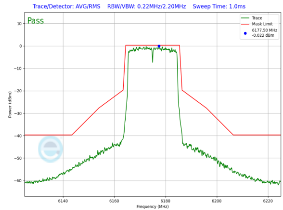
Plot 7-868. SP In-Band Emission Plot Antenna WF7a (20MHz 802.11ax RU242 (UNII Band 5) – Ch. 45)
