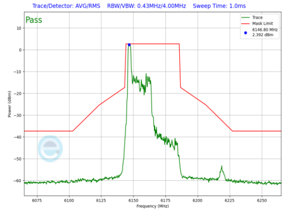
Plot 7-869. SP In-Band Emission Plot Antenna WF7a (40MHz 802.11ax RU26 (UNII Band 5) – Ch. 43)
