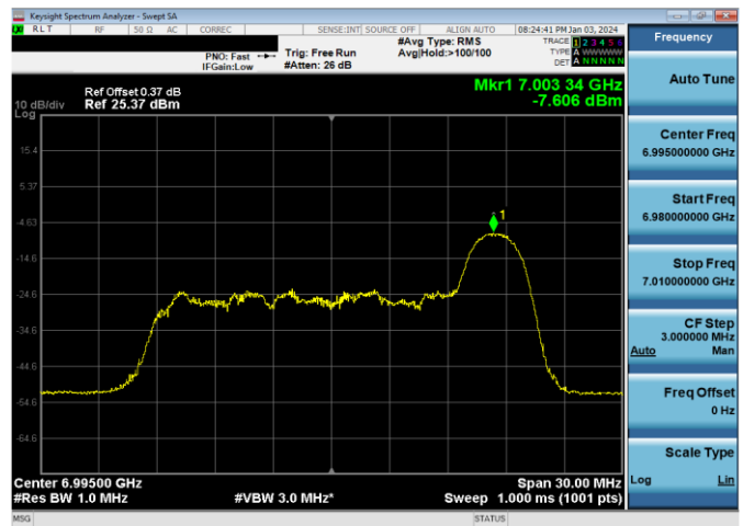
Plot 7-837. LPI Power Spectral Density Plot SDM Antenna WF2a (20MHz 802.11ax RU26 (UNII Band 8) – Ch. 209)
