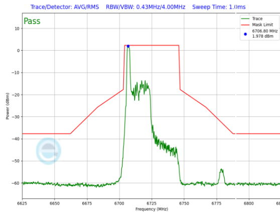
Plot 7-885. SP In-Band Emission Plot Antenna WF7a (40MHz 802.11ax RU26 (UNII Band 7) – Ch. 155)
