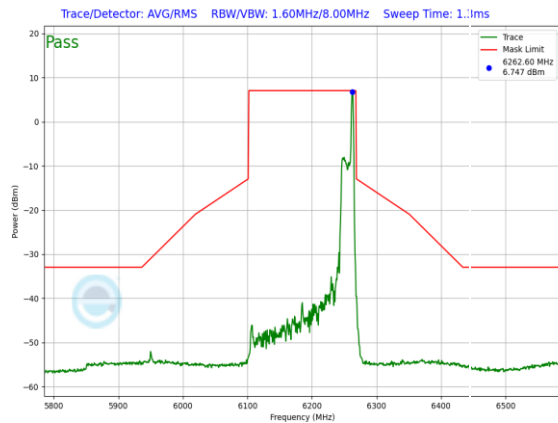
Plot 7-879. SP In-Band Emission Plot Antenna WF7a (160MHz 802.11ax RU26 (UNII Band 5) – Ch. 47)
