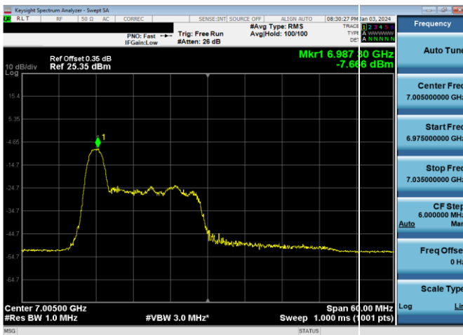
Plot 7-841. LPI Power Spectral Density Plot SDM Antenna WF2a (40MHz 802.11ax RU26 (UNII Band 8) – Ch. 211)
