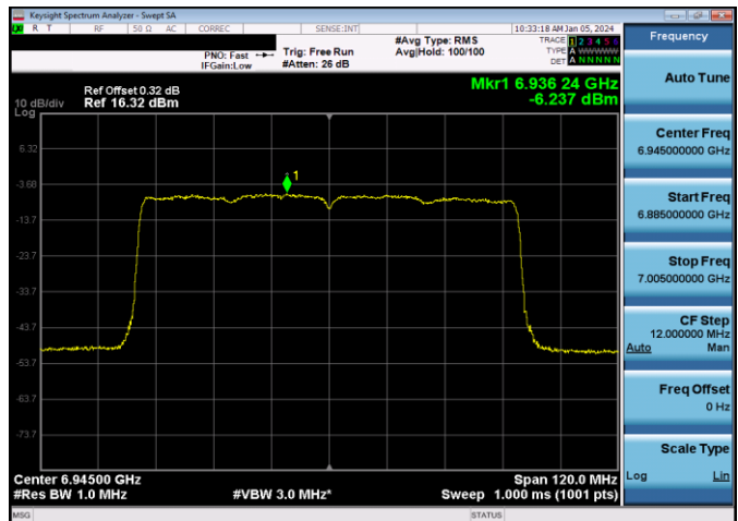
Plot 7-856. LPI Power Spectral Density Plot SDM Antenna WF7b (80MHz 802.11ax RU996 (UNII Band 8) – Ch. 199)
