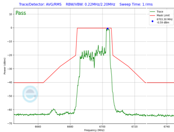
Plot 7-883. SP In-Band Emission Plot Antenna WF7a (20MHz 802.11ax RU26 (UNII Band 7) – Ch. 149)
