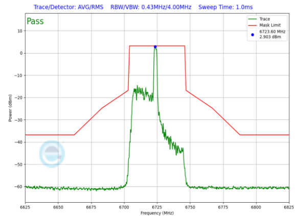
Plot 7-886. SP In-Band Emission Plot Antenna WF7a (40MHz 802.11ax RU26 (UNII Band 7) – Ch. 155)
