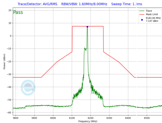
Plot 7-878. SP In-Band Emission Plot Antenna WF7a (160MHz 802.11ax RU26 (UNII Band 5) – Ch. 47)
