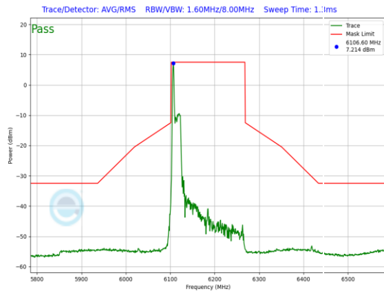
Plot 7-877. SP In-Band Emission Plot Antenna WF7a (160MHz 802.11ax RU26 (UNII Band 5) – Ch. 47)
