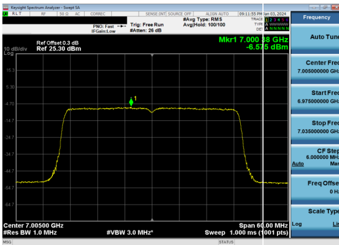
Plot 7-847. LPI Power Spectral Density Plot SDM Antenna WF2a (40MHz 802.11ax RU484 (UNII Band 8) – Ch. 211)
