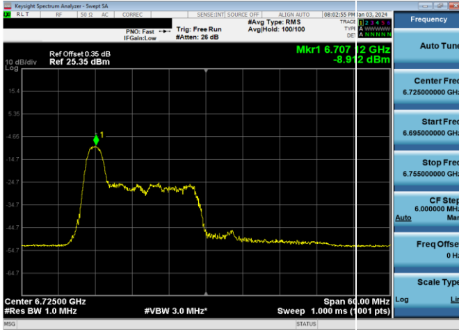
Plot 7-809. LPI Power Spectral Density Plot SDM Antenna WF2a (40MHz 802.11ax RU26 (UNII Band 7) – Ch. 155)
