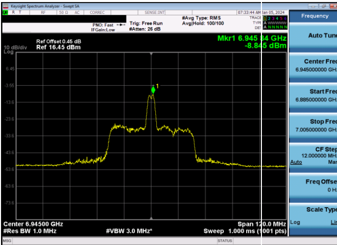
Plot 7-852. LPI Power Spectral Density Plot SDM Antenna WF7b (80MHz 802.11ax RU26 (UNII Band 8) – Ch. 199)
