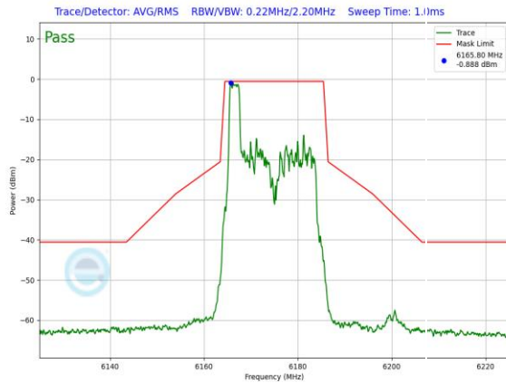
Plot 7-865. SP In-Band Emission Plot Antenna WF7a (20MHz 802.11ax RU26 (UNII Band 5) – Ch. 45)
