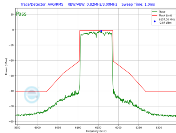
Plot 7-876. SP In-Band Emission Plot Antenna WF7a (80MHz 802.11ax RU996 (UNII Band 5) – Ch. 39)
