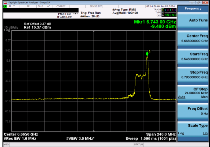
Plot 7-830. LPI Power Spectral Density Plot SDM Antenna WF7b (160MHz 802.11ax RU26 (UNII Band 7) – Ch. 143)
