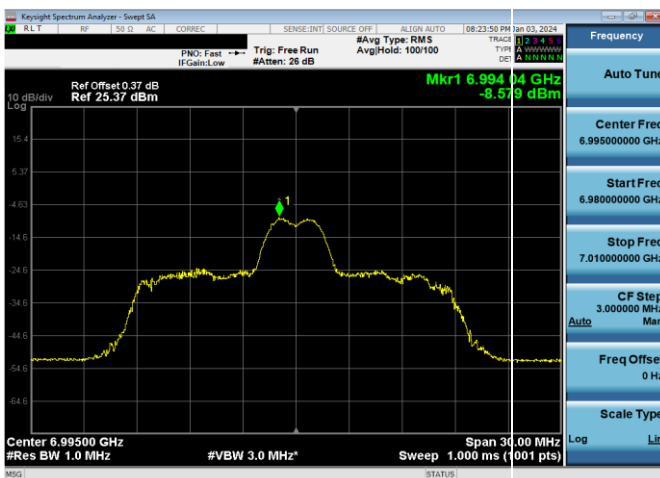
Plot 7-835. LPI Power Spectral Density Plot SDM Antenna WF2a (20MHz 802.11ax RU26 (UNII Band 8) – Ch. 209)
