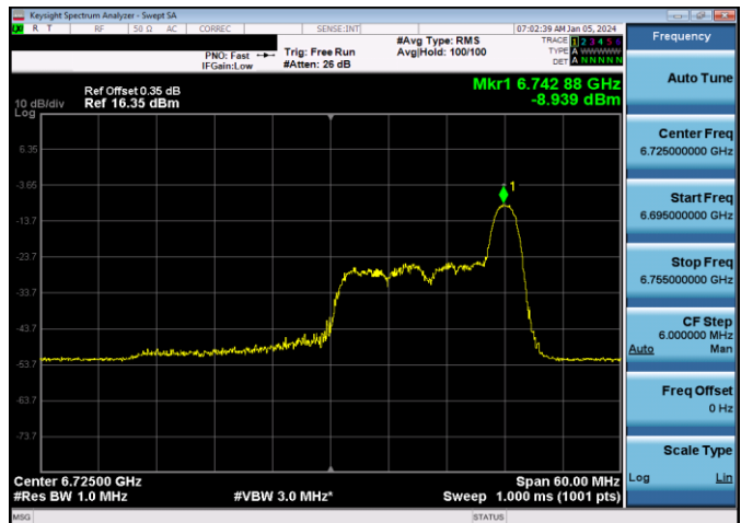
Plot 7-814. LPI Power Spectral Density Plot SDM Antenna WF7b (40MHz 802.11ax RU26 (UNII Band 7) – Ch. 155)
