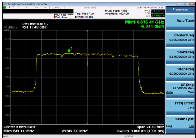
Plot 7-832. LPI Power Spectral Density Plot SDM Antenna WF7b (160MHz 802.11ax RU996x2 (UNII Band 7) – Ch. 143)
