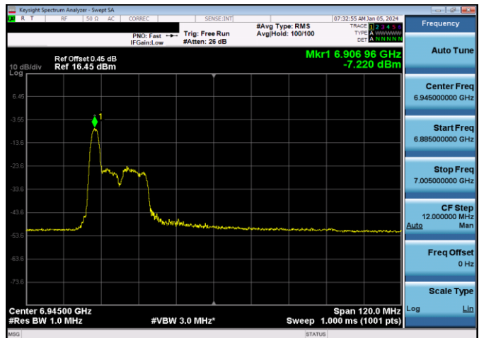
Plot 7-850. LPI Power Spectral Density Plot SDM Antenna WF7b (80MHz 802.11ax RU26 (UNII Band 8) – Ch. 199)
