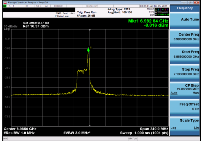
Plot 7-860. LPI Power Spectral Density Plot SDM Antenna WF7b (160MHz 802.11ax RU26 (UNII Band 8) – Ch. 207)
