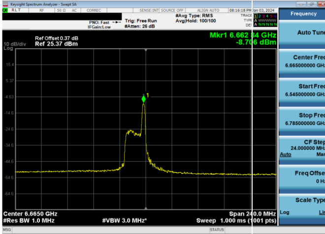
Plot 7-827. LPI Power Spectral Density Plot SDM Antenna WF2a (160MHz 802.11ax RU26 (UNII Band 7) – Ch. 143)
