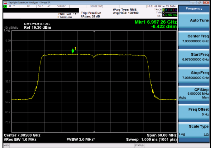
Plot 7-848. LPI Power Spectral Density Plot SDM Antenna WF7b (40MHz 802.11ax RU484 (UNII Band 8) – Ch. 211)
