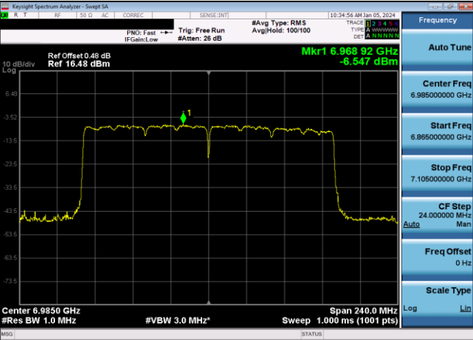
Plot 7-864. LPI Power Spectral Density Plot SDM Antenna WF7b (160MHz 802.11ax RU996x2 (UNII Band 8) – Ch. 207)
