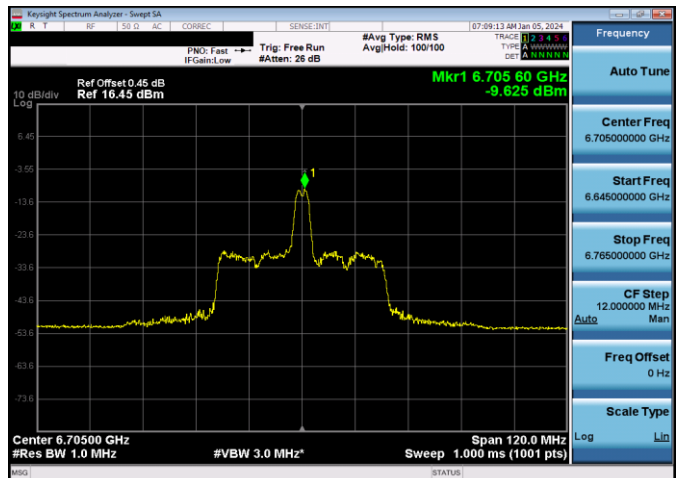
Plot 7-820. LPI Power Spectral Density Plot SDM Antenna WF7b (80MHz 802.11ax RU26 (UNII Band 7) – Ch. 151)
