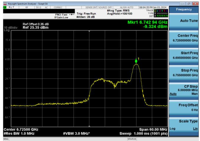
Plot 7-813. LPI Power Spectral Density Plot SDM Antenna WF2a (40MHz 802.11ax RU26 (UNII Band 7) – Ch. 155)
