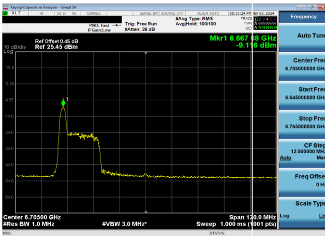
Plot 7-817. LPI Power Spectral Density Plot SDM Antenna WF2a (80MHz 802.11ax RU26 (UNII Band 7) – Ch. 151)
