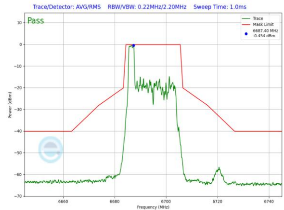
Plot 7-881. SP In-Band Emission Plot Antenna WF7a (20MHz 802.11ax RU26 (UNII Band 7) – Ch. 149)
