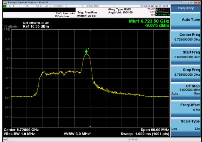
Plot 7-812. LPI Power Spectral Density Plot SDM Antenna WF7b (40MHz 802.11ax RU26 (UNII Band 7) – Ch. 155)
