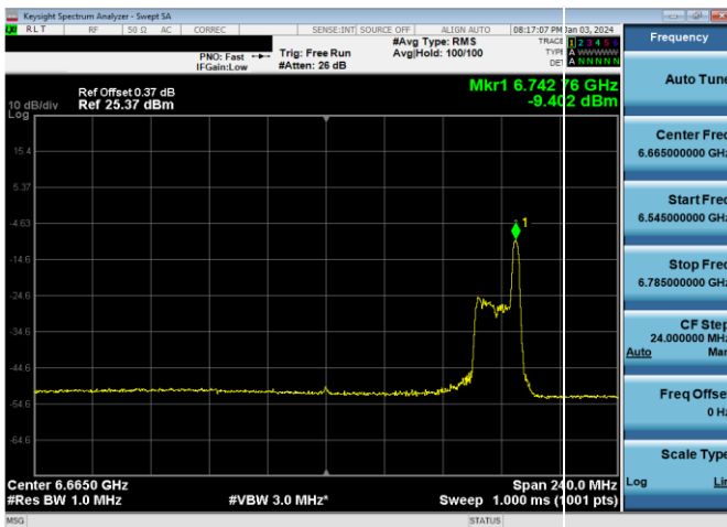
Plot 7-829. LPI Power Spectral Density Plot SDM Antenna WF2a (160MHz 802.11ax RU26 (UNII Band 7) – Ch. 143)
