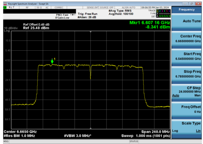
Plot 7-831. LPI Power Spectral Density Plot SDM Antenna WF2a (160MHz 802.11ax RU996x2 (UNII Band 7) – Ch. 143)
