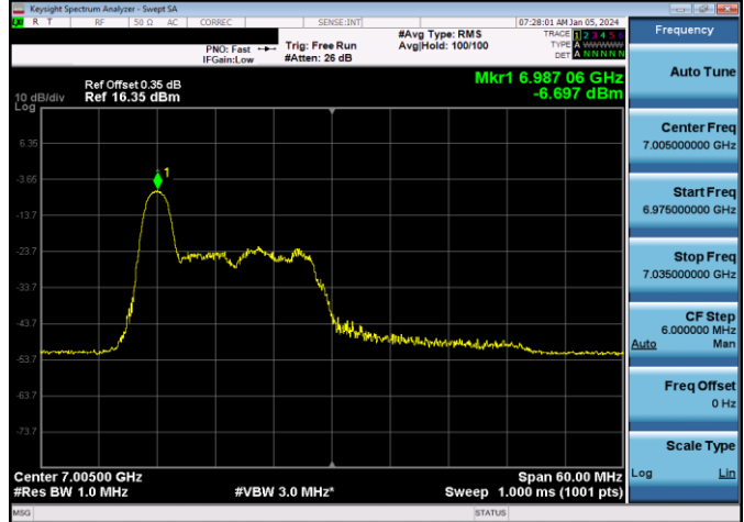
Plot 7-842. LPI Power Spectral Density Plot SDM Antenna WF7b (40MHz 802.11ax RU26 (UNII Band 8) – Ch. 211)
