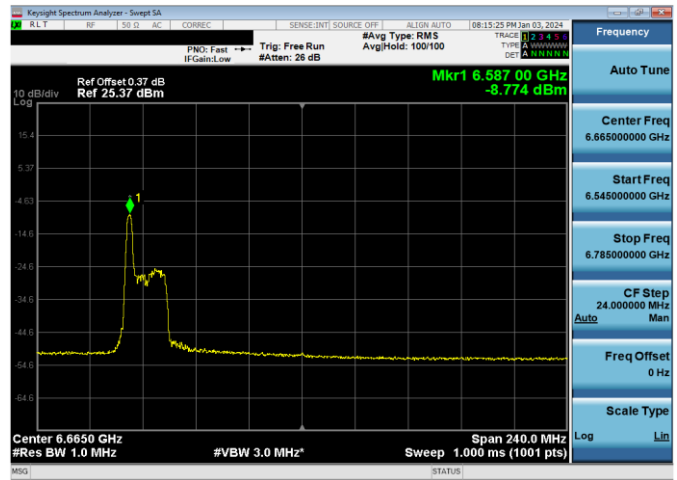
Plot 7-825. LPI Power Spectral Density Plot SDM Antenna WF2a (160MHz 802.11ax RU26 (UNII Band 7) – Ch. 143)
