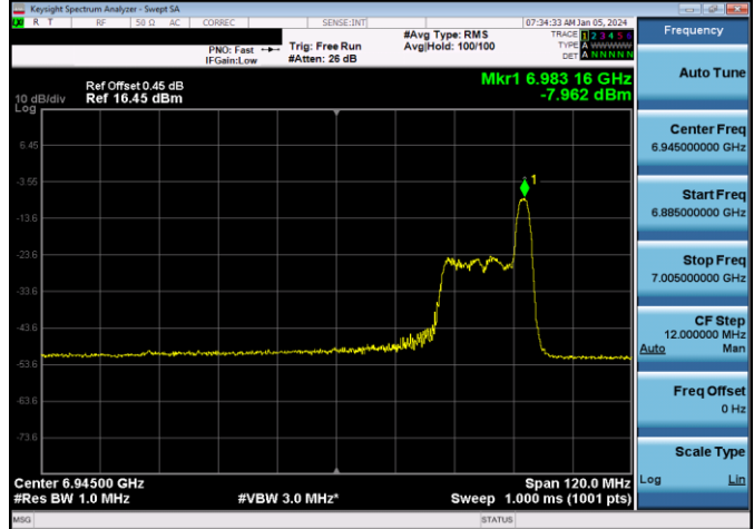
Plot 7-854. LPI Power Spectral Density Plot SDM Antenna WF7b (80MHz 802.11ax RU26 (UNII Band 8) – Ch. 199)
