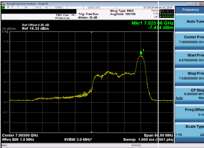
Plot 7-846. LPI Power Spectral Density Plot SDM Antenna WF7b (40MHz 802.11ax RU26 (UNII Band 8) – Ch. 211)
