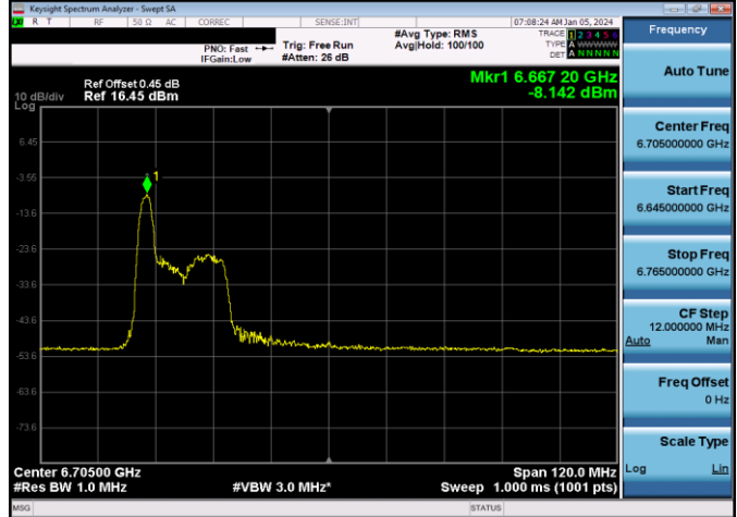
Plot 7-818. LPI Power Spectral Density Plot SDM Antenna WF7b (80MHz 802.11ax RU26 (UNII Band 7) – Ch. 151)
