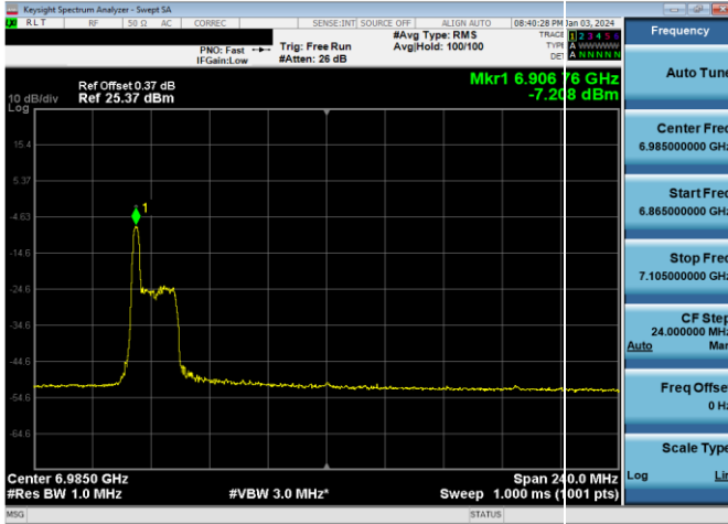
Plot 7-857. LPI Power Spectral Density Plot SDM Antenna WF2a (160MHz 802.11ax RU26 (UNII Band 8) – Ch. 207)
