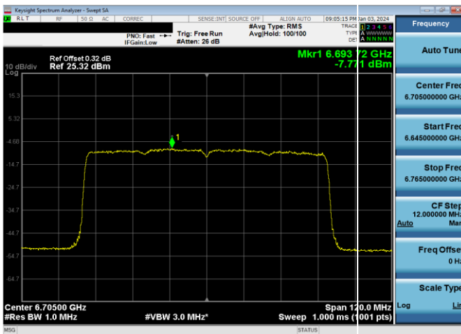
Plot 7-823. LPI Power Spectral Density Plot SDM Antenna WF2a (80MHz 802.11ax RU996 (UNII Band 7) – Ch. 151)
