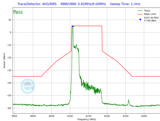
Plot 7-873. SP In-Band Emission Plot Antenna WF7a (80MHz 802.11ax RU26 (UNII Band 5) – Ch. 39)
