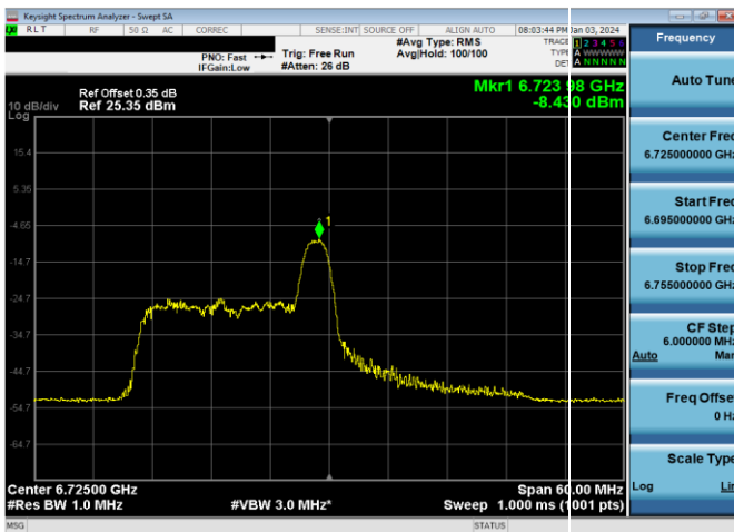
Plot 7-811. LPI Power Spectral Density Plot SDM Antenna WF2a (40MHz 802.11ax RU26 (UNII Band 7) – Ch. 155)
