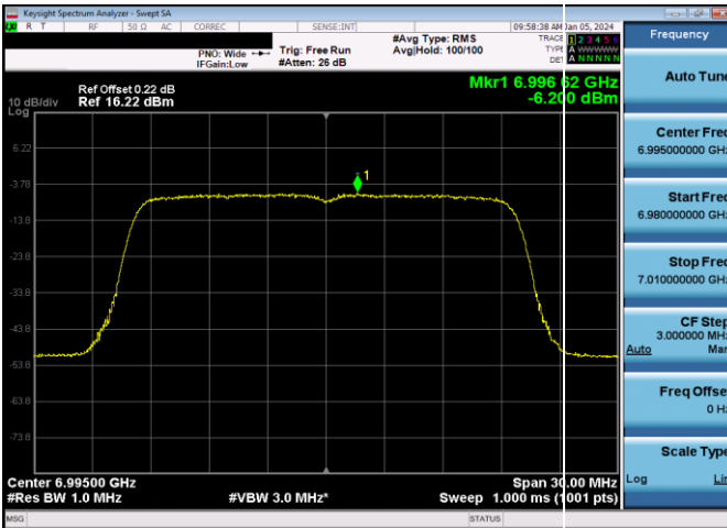
Plot 7-840. LPI Power Spectral Density Plot SDM Antenna WF7b (20MHz 802.11ax RU242 (UNII Band 8) – Ch. 209)
