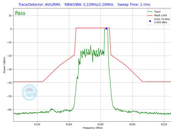
Plot 7-867. SP In-Band Emission Plot Antenna WF7a (20MHz 802.11ax RU26 (UNII Band 5) – Ch. 45)
