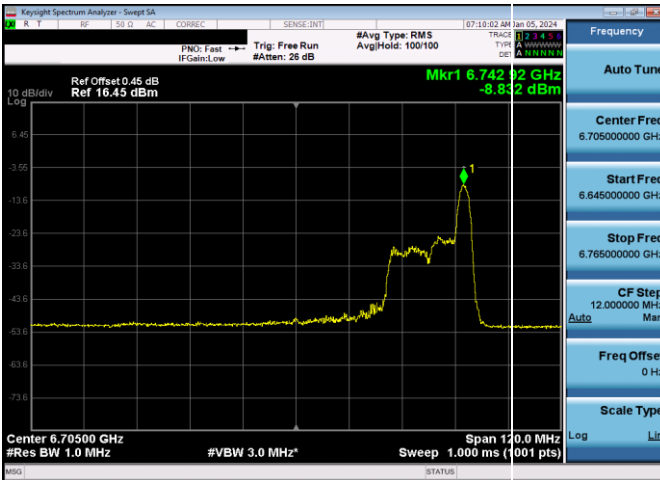
Plot 7-822. LPI Power Spectral Density Plot SDM Antenna WF7b (80MHz 802.11ax RU26 (UNII Band 7) – Ch. 151)
