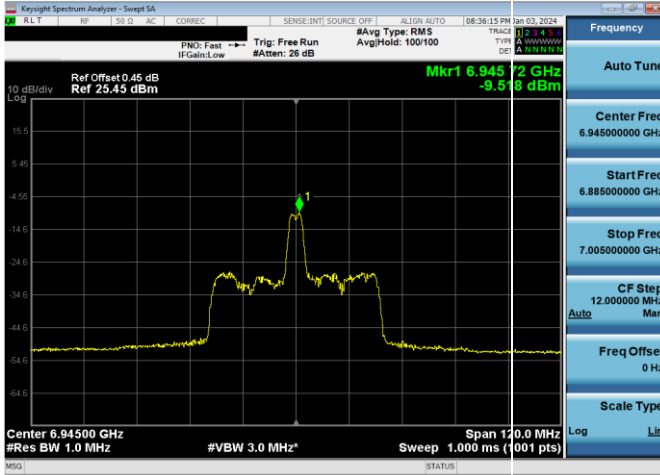
Plot 7-851. LPI Power Spectral Density Plot SDM Antenna WF2a (80MHz 802.11ax RU26 (UNII Band 8) – Ch. 199)
