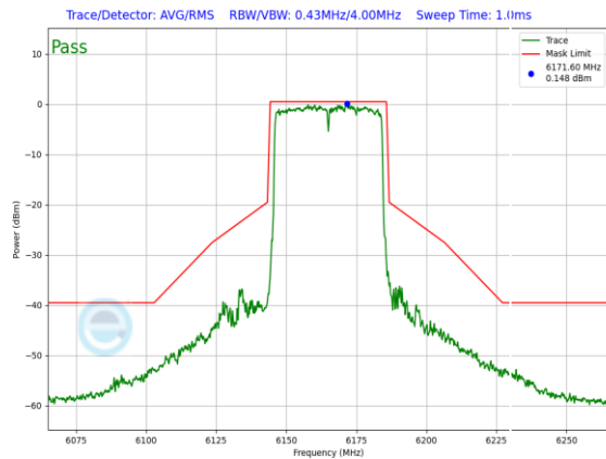
Plot 7-872. SP In-Band Emission Plot Antenna WF7a (40MHz 802.11ax RU484 (UNII Band 5) – Ch. 43)
