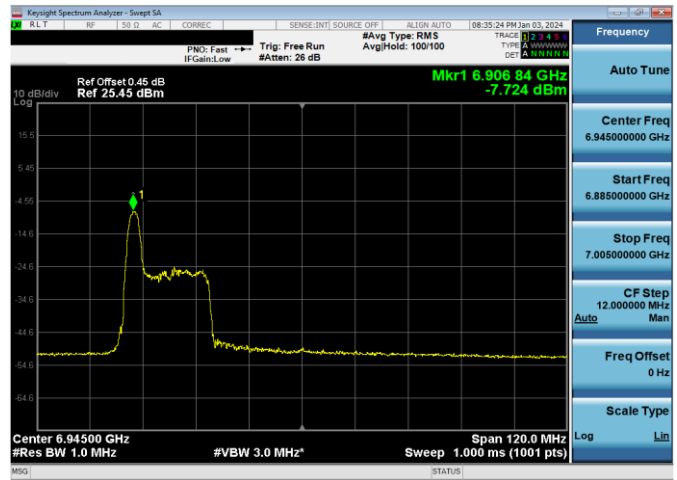
Plot 7-849. LPI Power Spectral Density Plot SDM Antenna WF2a (80MHz 802.11ax RU26 (UNII Band 8) – Ch. 199)
