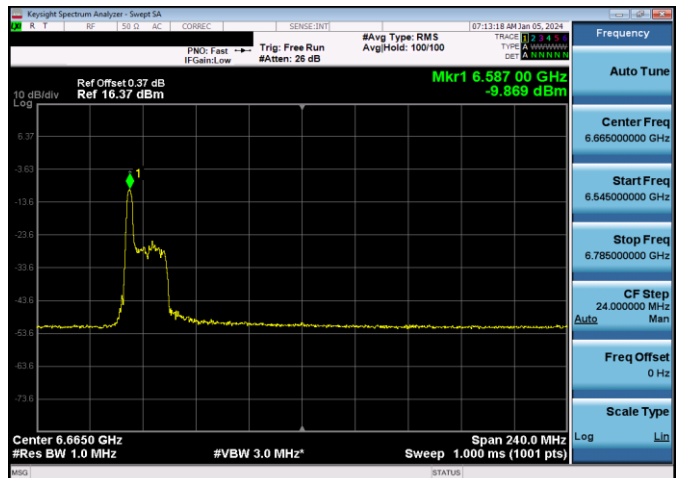
Plot 7-826. LPI Power Spectral Density Plot SDM Antenna WF7b (160MHz 802.11ax RU26 (UNII Band 7) – Ch. 143)
