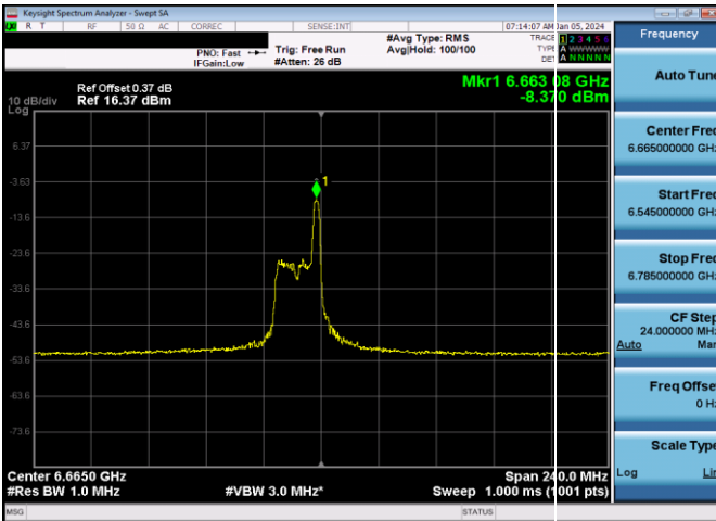
Plot 7-828. LPI Power Spectral Density Plot SDM Antenna WF7b (160MHz 802.11ax RU26 (UNII Band 7) – Ch. 143)
