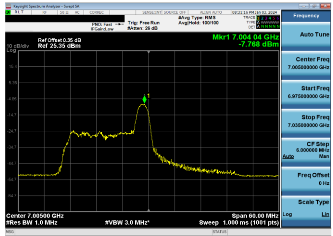
Plot 7-843. LPI Power Spectral Density Plot SDM Antenna WF2a (40MHz 802.11ax RU26 (UNII Band 8) – Ch. 211)
