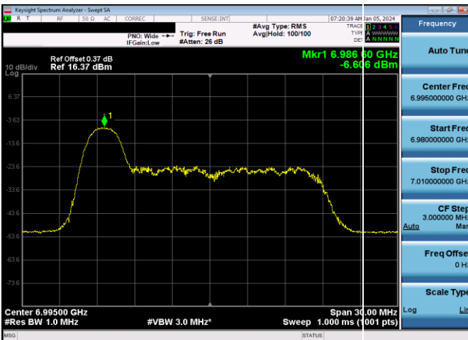
Plot 7-834. LPI Power Spectral Density Plot SDM Antenna WF7b (20MHz 802.11ax RU26 (UNII Band 8) – Ch. 209)
