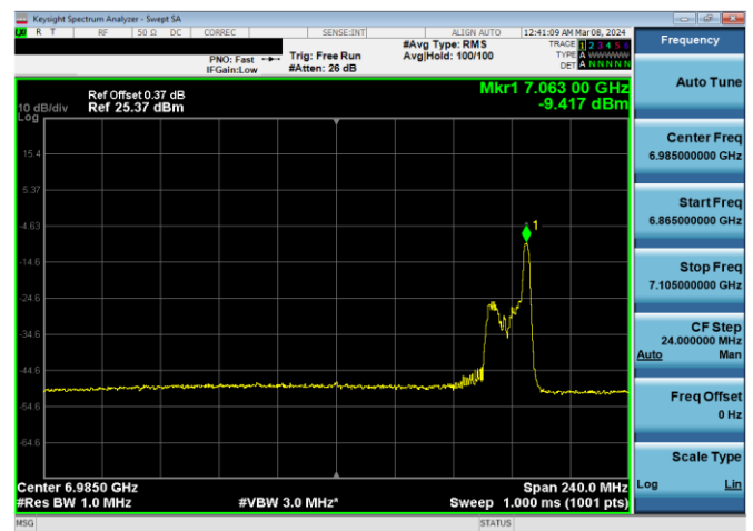
Plot 7-862. LPI Power Spectral Density Plot SDM Antenna WF7b (160MHz 802.11ax RU26 (UNII Band 8) – Ch. 207)
