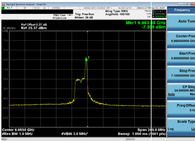
Plot 7-859. LPI Power Spectral Density Plot SDM Antenna WF2a (160MHz 802.11ax RU26 (UNII Band 8) – Ch. 207)
