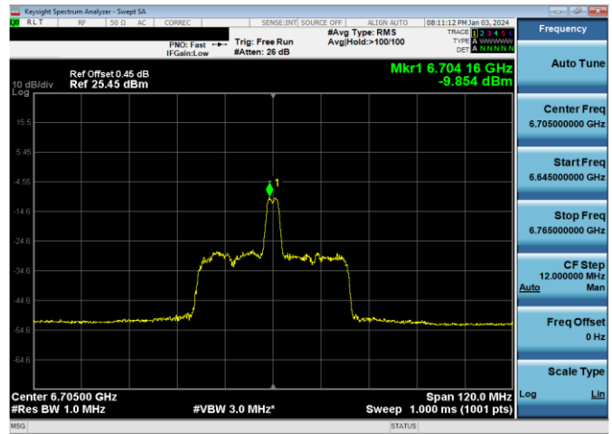
Plot 7-819. LPI Power Spectral Density Plot SDM Antenna WF2a (80MHz 802.11ax RU26 (UNII Band 7) – Ch. 151)
