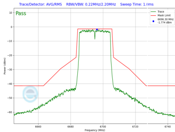
Plot 7-884. SP In-Band Emission Plot Antenna WF7a (20MHz 802.11ax RU242 (UNII Band 7) – Ch. 149)
