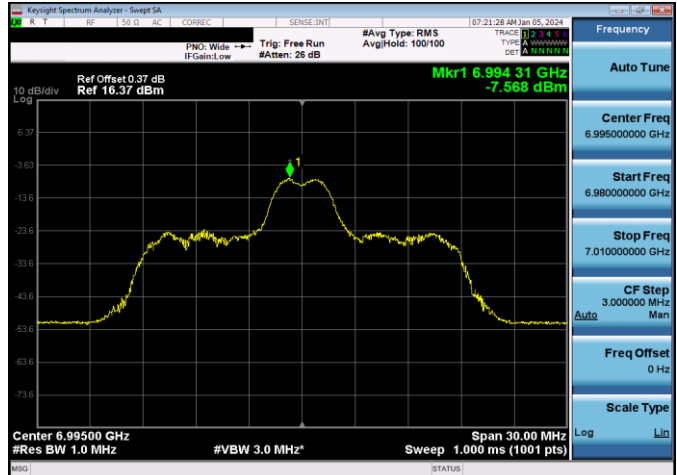
Plot 7-836. LPI Power Spectral Density Plot SDM Antenna WF7b (20MHz 802.11ax RU26 (UNII Band 8) – Ch. 209)
