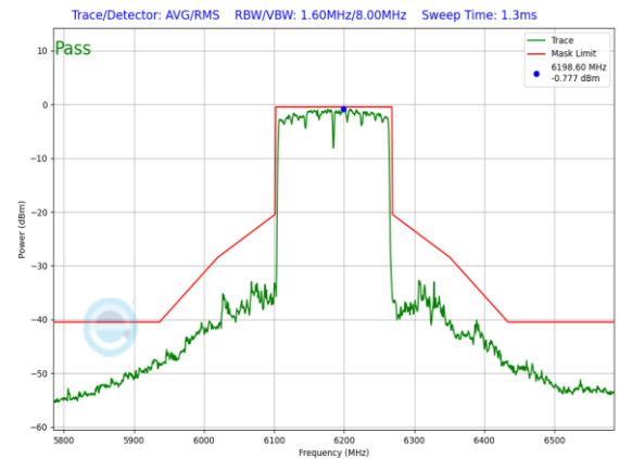
Plot 7-880. SP In-Band Emission Plot Antenna WF7a (160MHz 802.11ax RU996x2 (UNII Band 5) – Ch. 47)
