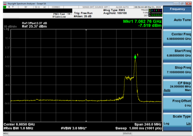
Plot 7-861. LPI Power Spectral Density Plot SDM Antenna WF2a (160MHz 802.11ax RU26 (UNII Band 8) – Ch. 207)
