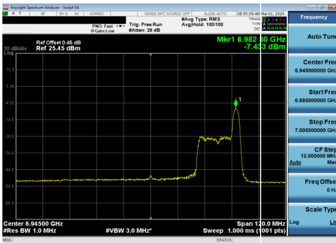
Plot 7-853. LPI Power Spectral Density Plot SDM Antenna WF2a (80MHz 802.11ax RU26 (UNII Band 8) – Ch. 199)
