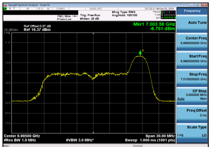
Plot 7-838. LPI Power Spectral Density Plot SDM Antenna WF7b (20MHz 802.11ax RU26 (UNII Band 8) – Ch. 209)
