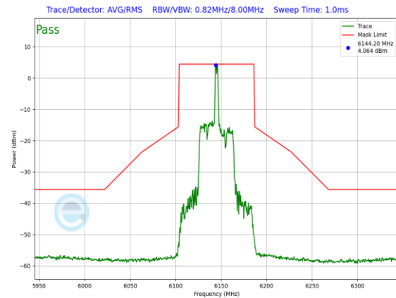
Plot 7-874. SP In-Band Emission Plot Antenna WF7a (80MHz 802.11ax RU26 (UNII Band 5) – Ch. 39)
