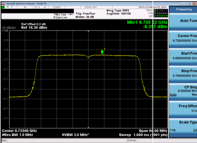
Plot 7-816. LPI Power Spectral Density Plot SDM Antenna WF7b (40MHz 802.11ax RU484 (UNII Band 7) – Ch. 155)
