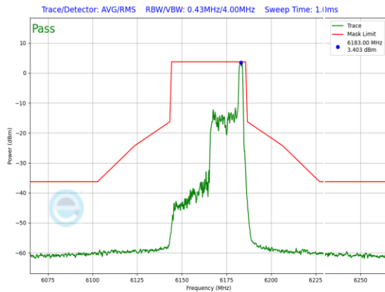
Plot 7-871. SP In-Band Emission Plot Antenna WF7a (40MHz 802.11ax RU26 (UNII Band 5) – Ch. 43)
