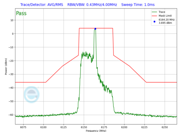
Plot 7-870. SP In-Band Emission Plot Antenna WF7a (40MHz 802.11ax RU26 (UNII Band 5) – Ch. 43)
