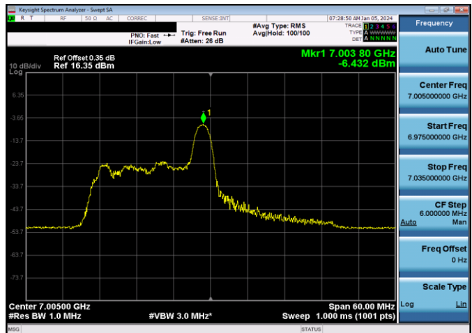
Plot 7-844. LPI Power Spectral Density Plot SDM Antenna WF7b (40MHz 802.11ax RU26 (UNII Band 8) – Ch. 211)
