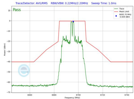
Plot 7-882. SP In-Band Emission Plot Antenna WF7a (20MHz 802.11ax RU26 (UNII Band 7) – Ch. 149)
