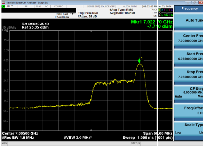
Plot 7-845. LPI Power Spectral Density Plot SDM Antenna WF2a (40MHz 802.11ax RU26 (UNII Band 8) – Ch. 211)
