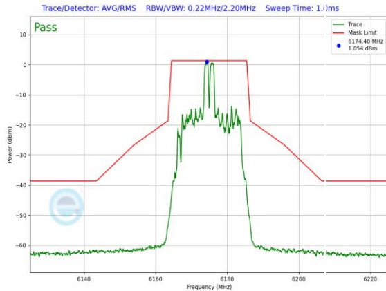
Plot 7-866. SP In-Band Emission Plot Antenna WF7a (20MHz 802.11ax RU26 (UNII Band 5) – Ch. 45)
