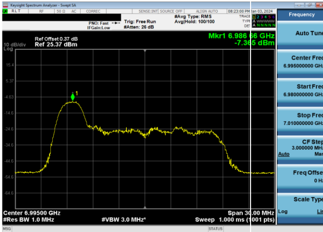
Plot 7-833. LPI Power Spectral Density Plot SDM Antenna WF2a (20MHz 802.11ax RU26 (UNII Band 8) – Ch. 209)
