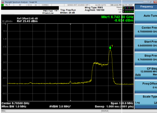
Plot 7-821. LPI Power Spectral Density Plot SDM Antenna WF2a (80MHz 802.11ax RU26 (UNII Band 7) – Ch. 151)
