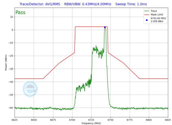
Plot 7-887. SP In-Band Emission Plot Antenna WF7a (40MHz 802.11ax RU26 (UNII Band 7) – Ch. 155)
