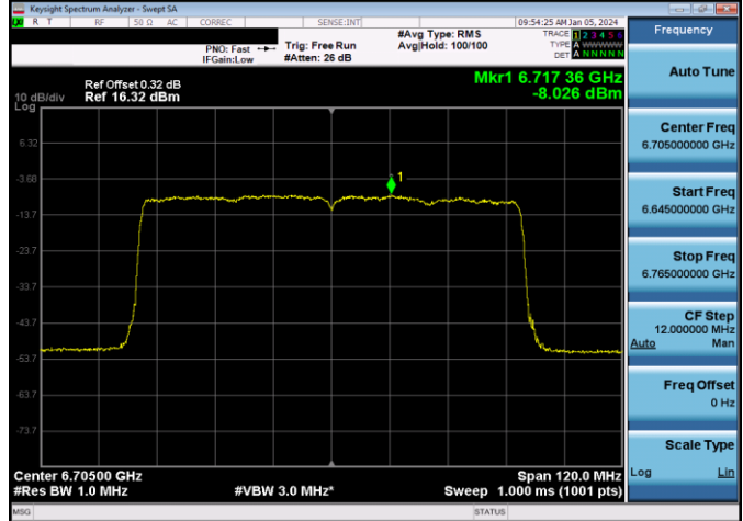
Plot 7-824. LPI Power Spectral Density Plot SDM Antenna WF7b (80MHz 802.11ax RU996 (UNII Band 7) – Ch. 151)
