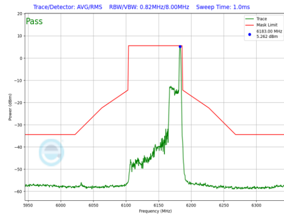
Plot 7-875. SP In-Band Emission Plot Antenna WF7a (80MHz 802.11ax RU26 (UNII Band 5) – Ch. 39)
