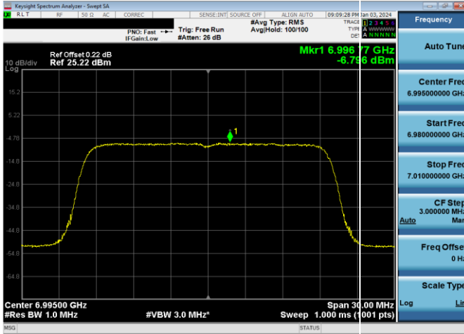
Plot 7-839. LPI Power Spectral Density Plot SDM Antenna WF2a (20MHz 802.11ax RU242 (UNII Band 8) – Ch. 209)
