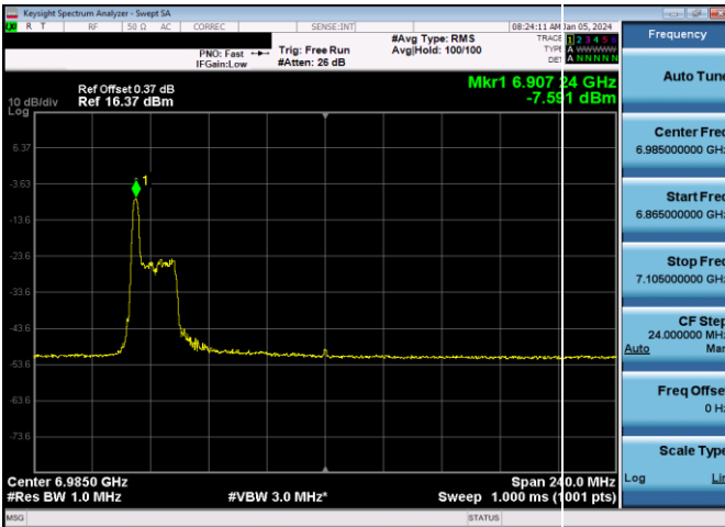
Plot 7-858. LPI Power Spectral Density Plot SDM Antenna WF7b (160MHz 802.11ax RU26 (UNII Band 8) – Ch. 207)
