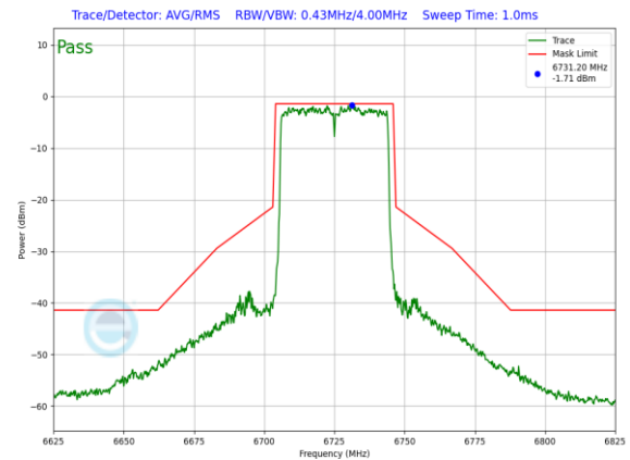
Plot 7-888. SP In-Band Emission Plot Antenna WF7a (40MHz 802.11ax RU484 (UNII Band 7) – Ch. 155)
