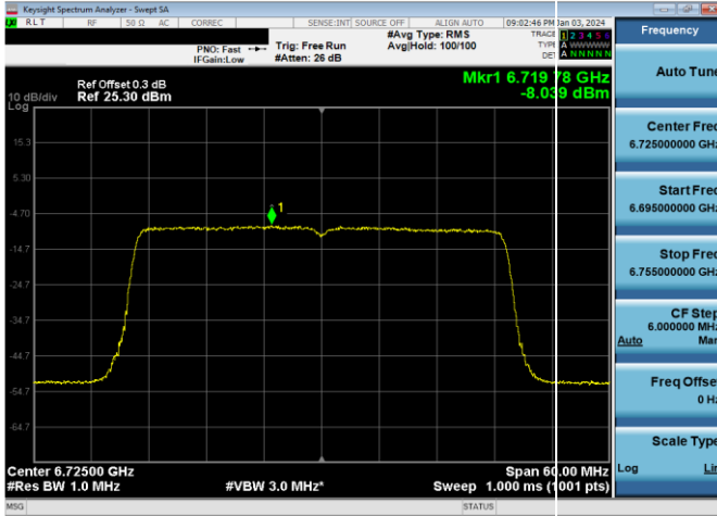
Plot 7-815. LPI Power Spectral Density Plot SDM Antenna WF2a (40MHz 802.11ax RU484 (UNII Band 7) – Ch. 155)
