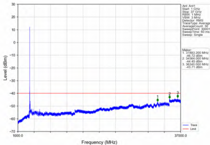
n78d_30kHz_SISO_NTNV_60MHz_DFT-s-OFDM_QPSK_3669.99MHz_Edge_1RB_Right
