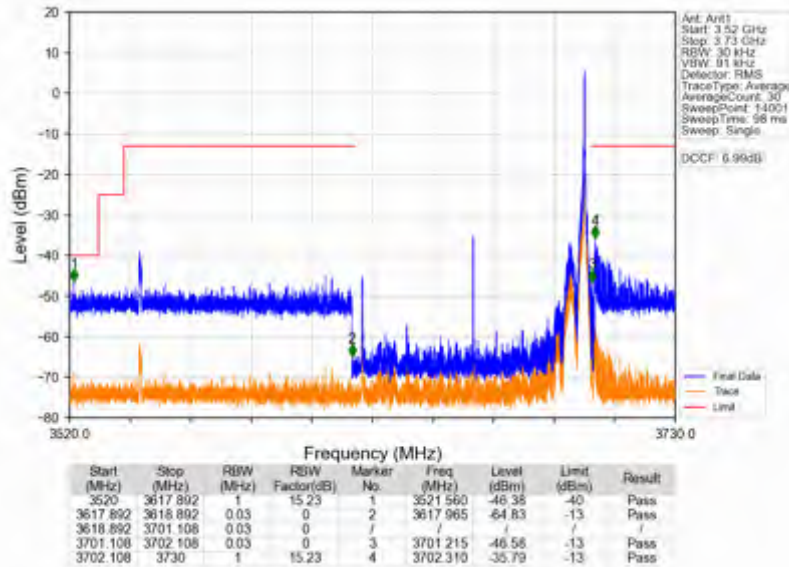
n78d_30kHz_SISO_NTNV_80MHz_DFT-s-OFDM QPSK_3660MHz_Inner_1RB_Right
