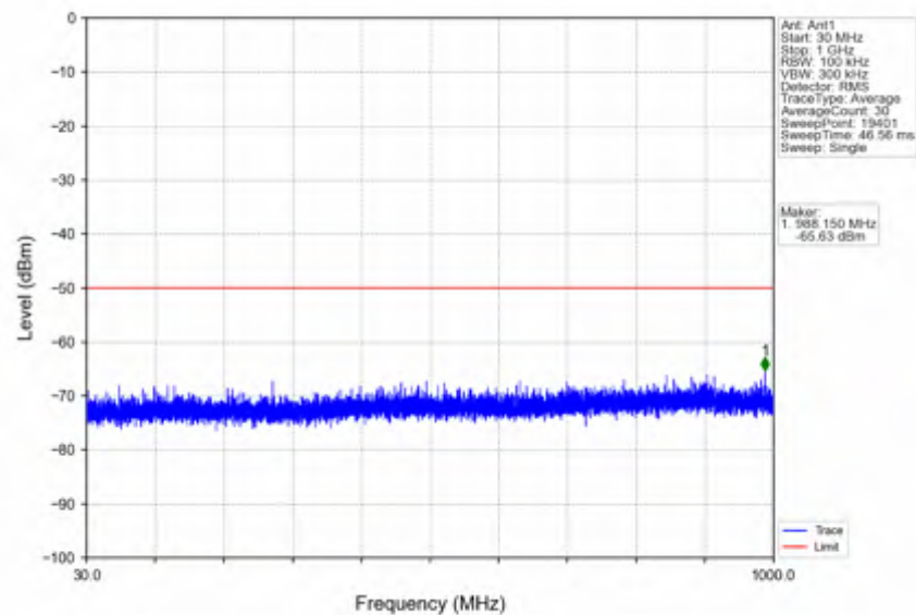
n78d_30kHz_SISO_NTNV_80MHz_CP-OFDM QPSK_3660MHz_Edge_1RB_Right
