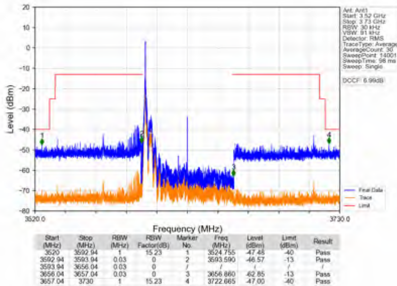
n78d_30kHz_SISO_NTV_60MHz_CP-OFDM QPSK_3624.99MHz_Edge_1RB_Left
