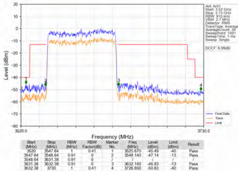
n78d_30kHz_SISO_NTNV_80MHz_DFT-s-OFDM_QPSK_3590.01MHz_Outer_Full
