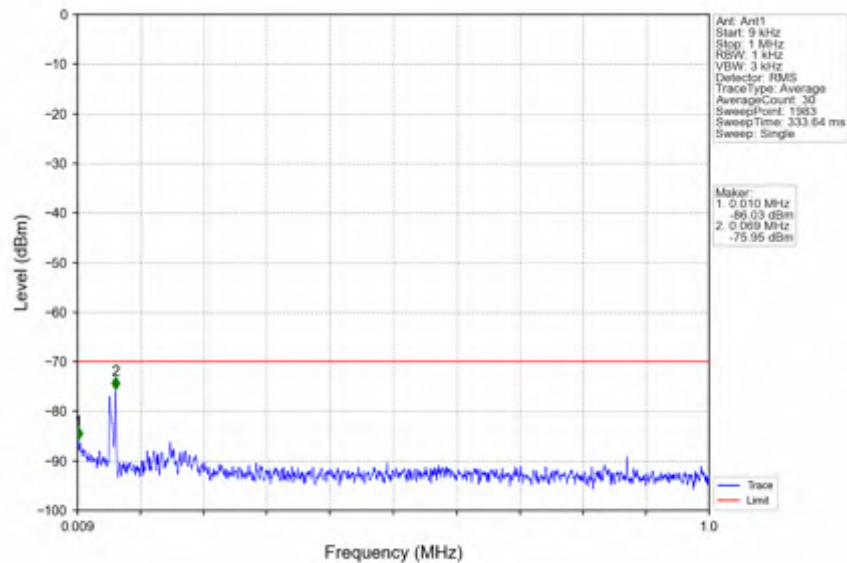
n78d_30kHz_SISO_NTNV_70MHz_DFT-s-OFDM QPSK_3664.98MHz_Edge_1RB_Right
