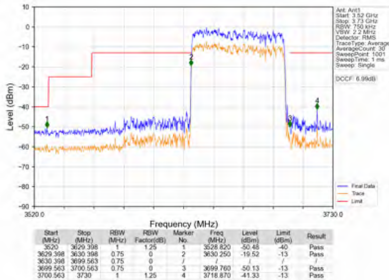
n78d_30kHz_SISO_NTNV_70MHz_DFT-s-OFDM_QPSK_3664.98MHz_Outer_Full
