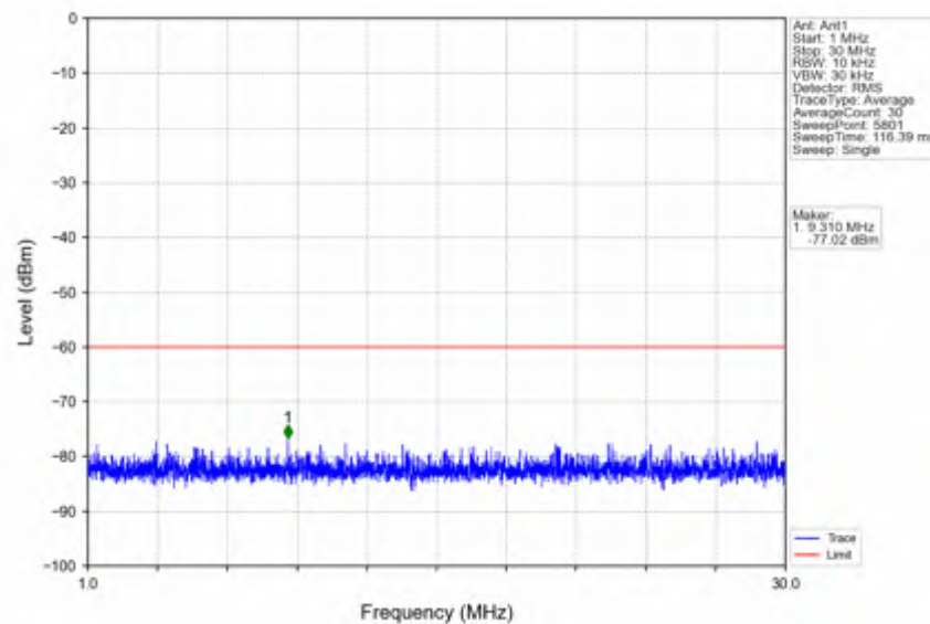
n78d_30kHz_SISO_NTNV_80MHz_CP-OFDM_QPSK_3660MHz_Inner_1RB_Right
