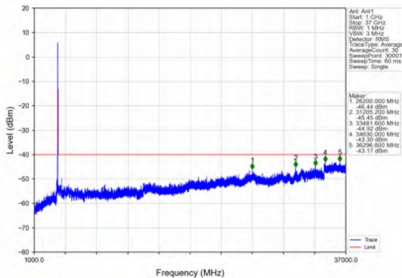
n78d_30kHz_SISO_NTNV_60MHz_CP-OFDM_QPSK_3669.99MHz_Outer_Full
