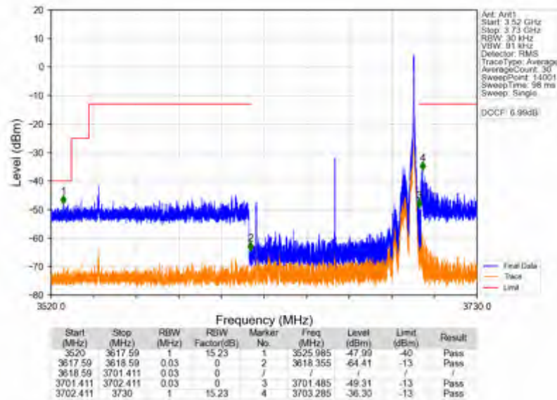
n78d_30kHz_SISO_NTNV_80MHz_CP-OFDM QPSK_3660MHz_Edge_1RB_Right
