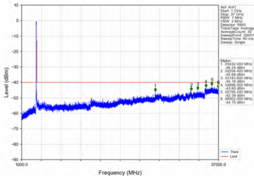
n78d_30kHz_SISO_NTNV_70MHz_DFT-s-OFDM QPSK_3664.98MHz_Inner_1RB_Right
