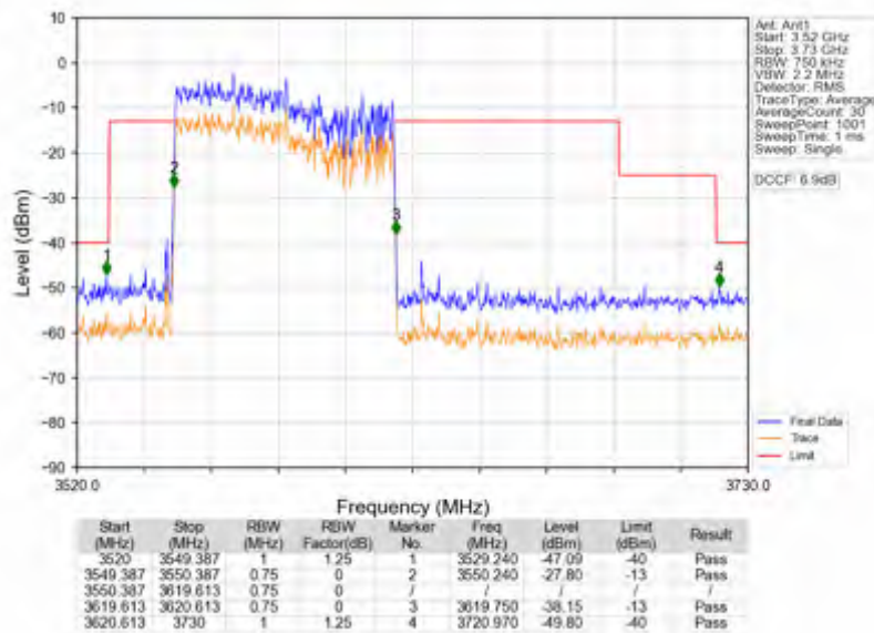
n78d_30kHz_SISO_NTNV_70MHz_CP-OFDM QPSK_3585MHz_Outer_Full
