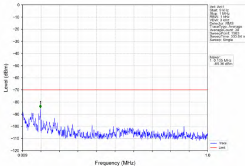
n78d_30kHz_SISO_NTNV_60MHz_DFT-s-OFDM_QPSK_3580.02MHz_Outer_Full
