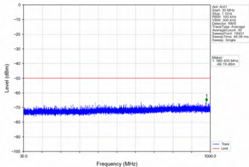
n78d_30kHz_SISO_NTNV_70MHz_CP-OFDM QPSK_3664.98MHz_Outer_Full
