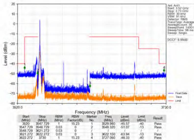
n78d_30kHz_SISO_NTNV_70MHz_DFT-s-OFDM_QPSK_3585MHz_Inner_1RB_Left
