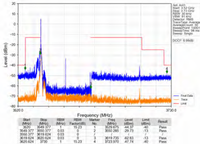
n78d_30kHz_SISO_NTNV_70MHz_CP-OFDM_QPSK_3585MHz_Edge_1RB_Left
