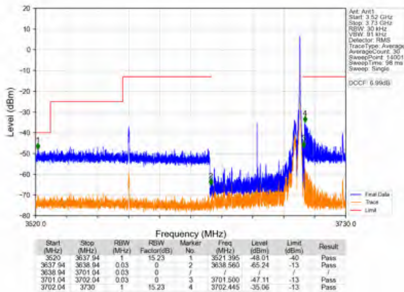
n78d_30kHz_SISO_NTNV_60MHz_DFT-s-OFDM_QPSK_3669.99MHz_Edge_1RB_Right
