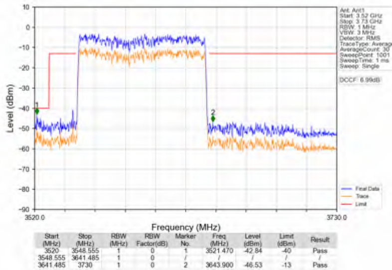
n78d_30kHz_SISO_NTNV_90MHz_DFT-s-OFDM_QPSK_3595.02MHz_Outer_Full
