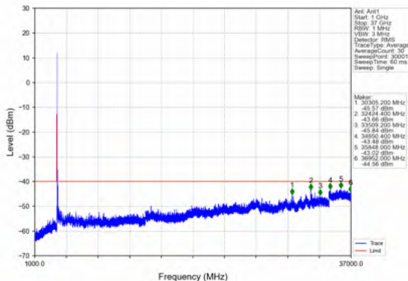
n78d_30kHz_SISO_NTNV_70MHz_CP-OFDM QPSK_3585MHz_Outer_Full
