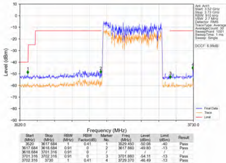
n78d_30kHz_SISO_NTNV_80MHz_CP-OFDM QPSK_3660MHz_Outer_Full
