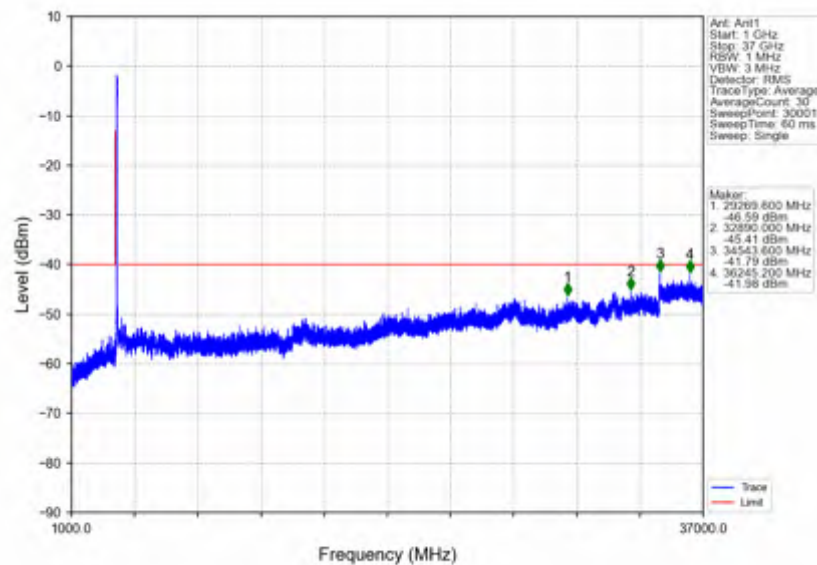
n78d_30kHz_SISO_NTNV_60MHz_CP-OFDM QPSK_3580.02MHz_Outer_Full
