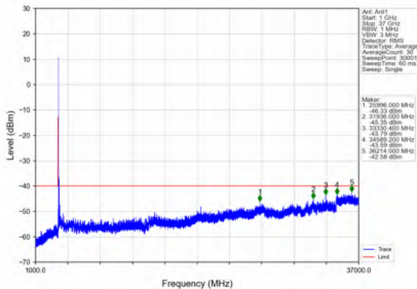
n78d_30kHz_SISO_NTV_70MHz_CP-OFDM QPSK_3624.99MHz_Edge_1RB_Left
