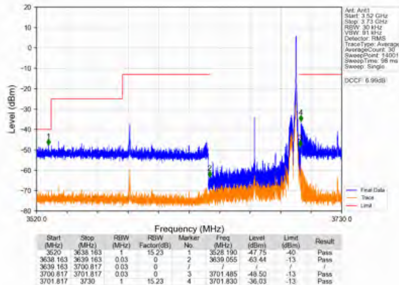
n78d_30kHz_SISO_NTNV_60MHz_CP-OFDM_QPSK_3669.99MHz_Inner_1RB_Right
