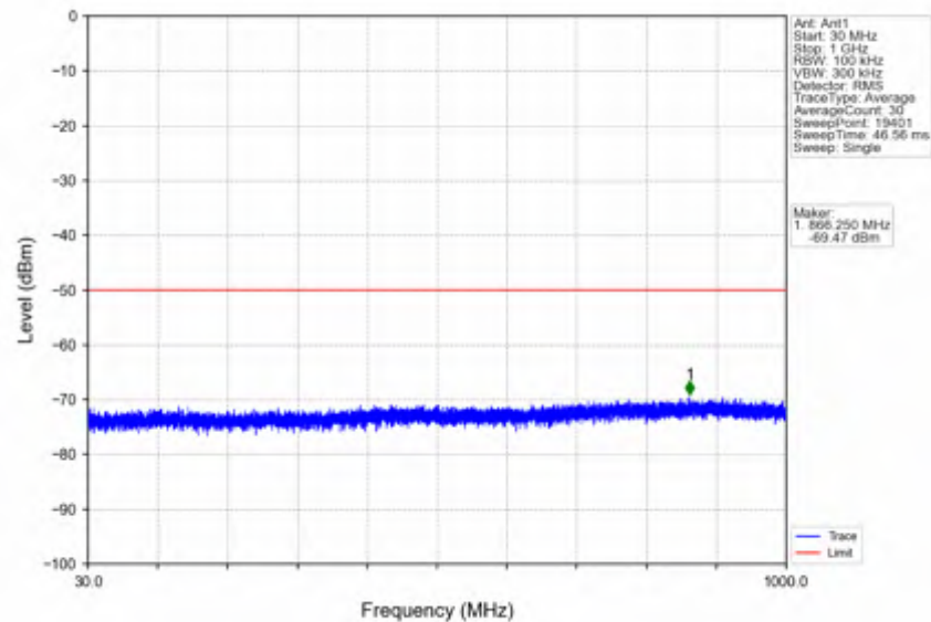
n78d_30kHz_SISO_NTNV_80MHz_DFT-s-OFDM_PI/2_BPSK_3660MHz_Outer_Full
