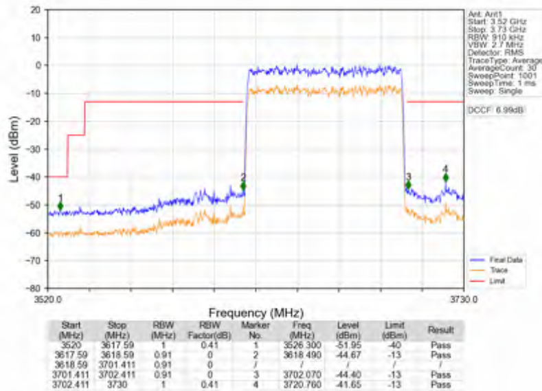
n78d_30kHz_SISO_NTNV_80MHz_DFT-s-OFDM_PI/2_BPSK_3660MHz_Outer_Full
