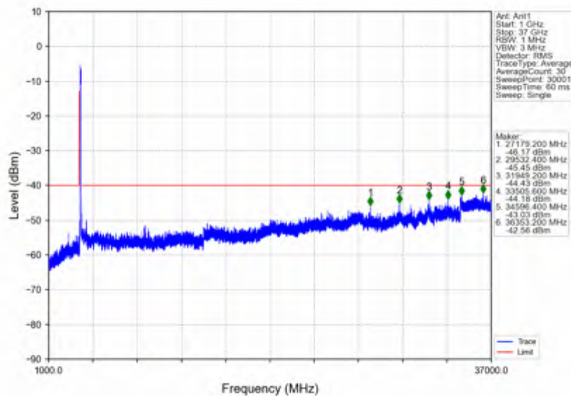
n78d_30kHz_SISO_NTNV_80MHz_DFT-s-OFDM_QPSK_3590.01MHz_Inner_1RB_Left
