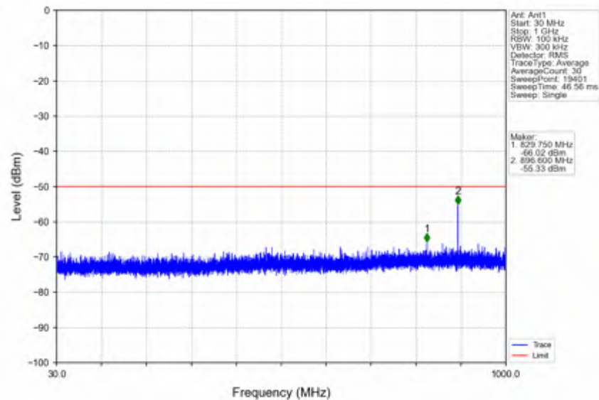
n78d_30kHz_SISO_NTNV_60MHz_DFT-s-OFDM QPSK_3669.99MHz_Inner_1RB_Right
