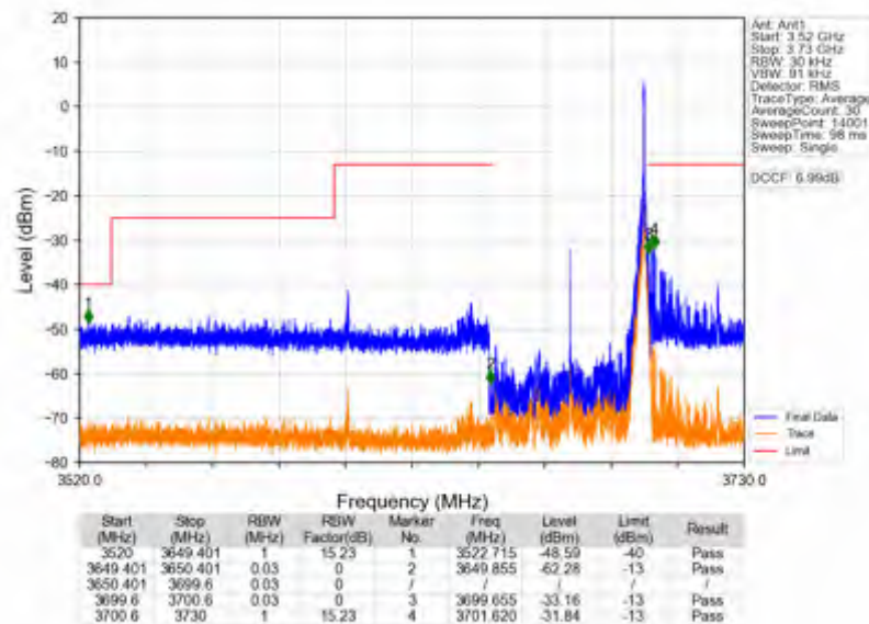
n78d_30kHz_SISO_NTNV_50MHz_CP-OFDM_QPSK_3675MHz_Inner_1RB_Right
