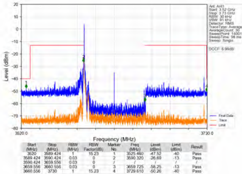
n78d_30kHz_SISO_NTV_70MHz_CP-OFDM QPSK_3624.99MHz_Edge_1RB_Left
