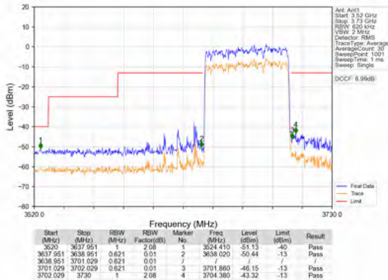
n78d_30kHz_SISO_NTNV_60MHz_DFT-s-OFDM_QPSK_3669.99MHz_Outer_Full
