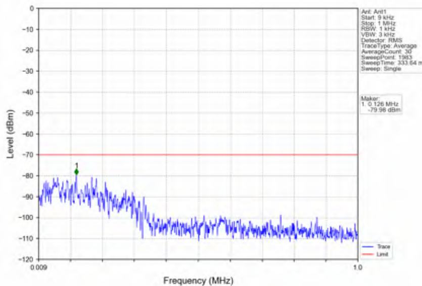
n78d_30kHz_SISO_NTNV_70MHz_CP-OFDM_QPSK_3585MHz_Edge_1RB_Left
