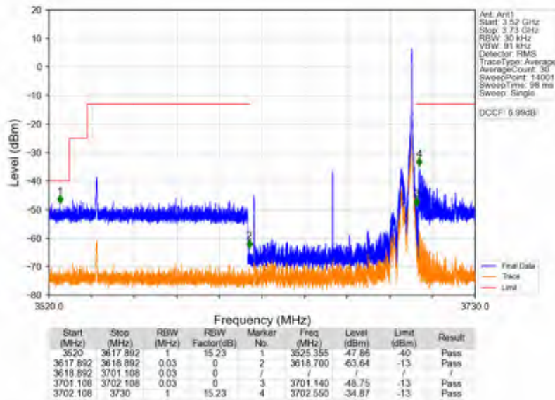
n78d_30kHz_SISO_NTNV_80MHz_DFT-s-OFDM QPSK_3660MHz_Edge_1RB_Right
