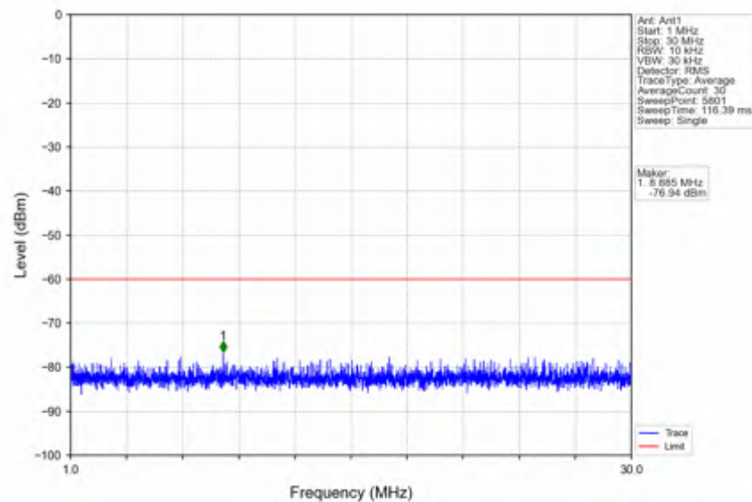
n78d_30kHz_SISO_NTNV_80MHz_CP-OFDM QPSK_3660MHz_Edge_1RB_Right
