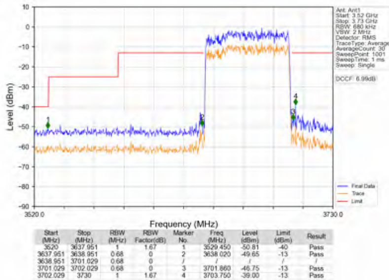
n78d_30kHz_SISO_NTNV_60MHz_CP-OFDM_QPSK_3669.99MHz_Outer_Full
