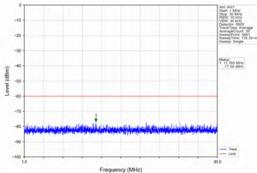
n78d_30kHz_SISO_NTNV_70MHz_CP-OFDM_QPSK_3585MHz_Edge_1RB_Left
