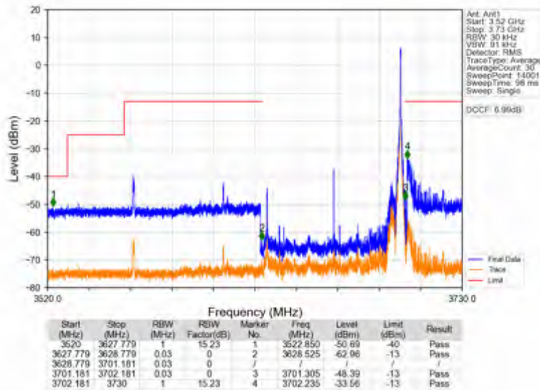
n78d_30kHz_SISO_NTNV_70MHz_DFT-s-OFDM QPSK_3664.98MHz_Edge_1RB_Right
