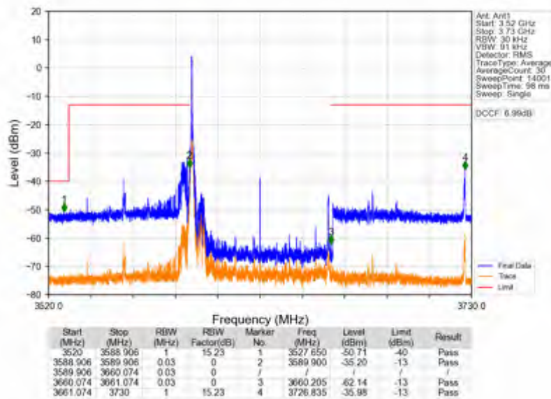
n78d_30kHz_SISO_NTNV_70MHz_DFT-s-OFDM_PI/2_BPSK_3624.99MHz_Edge_1RB_Left
