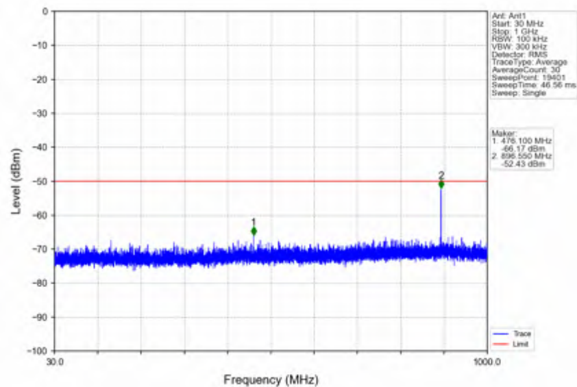
n78d_30kHz_SISO_NTNV_60MHz_CP-OFDM QPSK_3580.02MHz_Outer_Full
