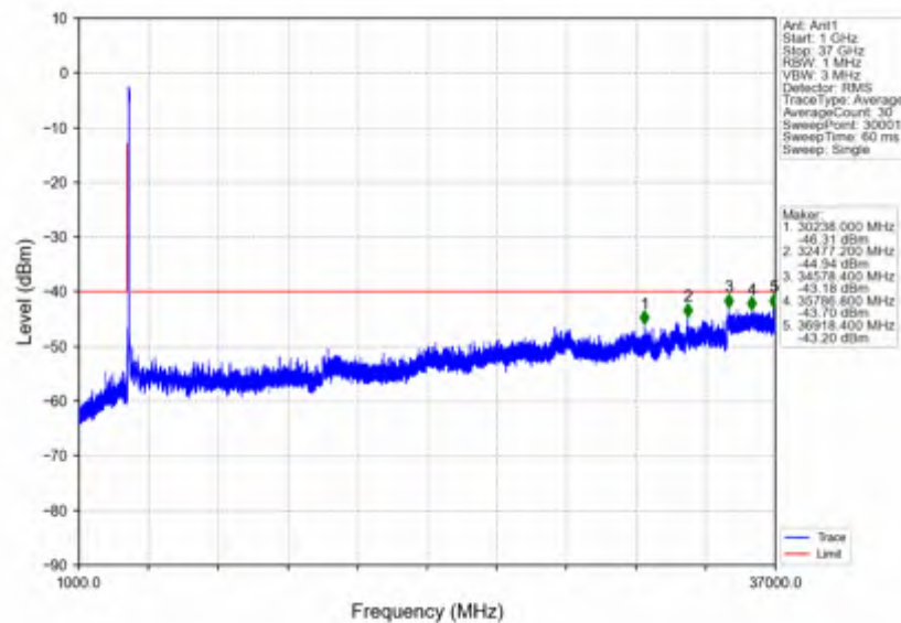
n78d_30kHz_SISO_NTNV_70MHz_DFT-s-OFDM_QPSK_3585MHz_Inner_1RB_Left
