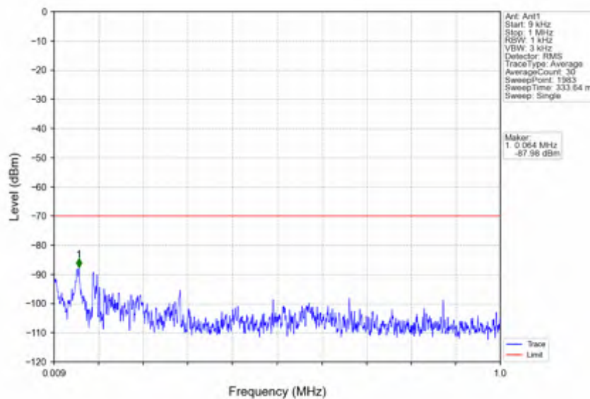
n78d_30kHz_SISO_NTNV_70MHz_DFT-s-OFDM_QPSK_3664.98MHz_Outer_Full
