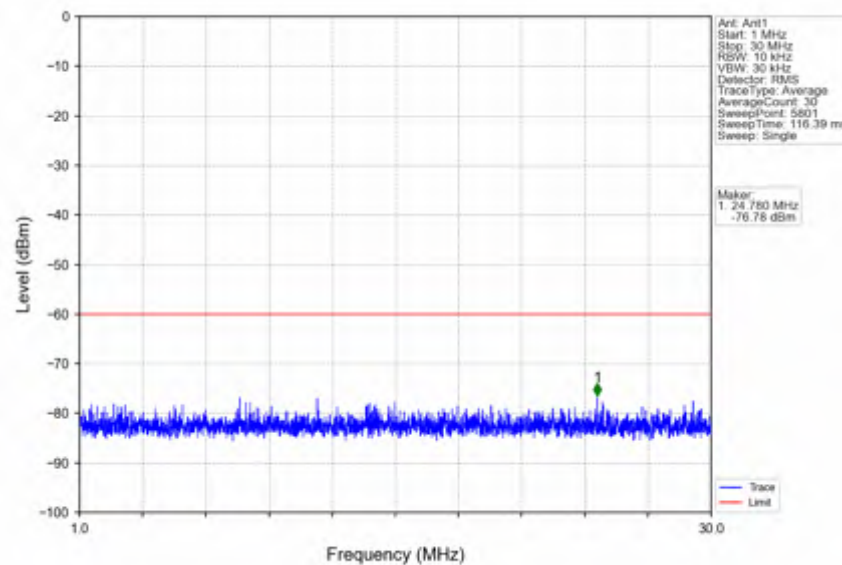
n78d_30kHz_SISO_NTNV_70MHz_CP-OFDM QPSK_3664.98MHz_Inner_1RB_Right
