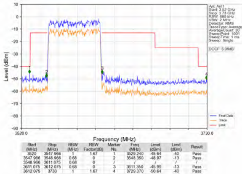
n78d_30kHz_SISO_NTNV_60MHz_DFT-s-OFDM_QPSK_3580.02MHz_Outer_Full
