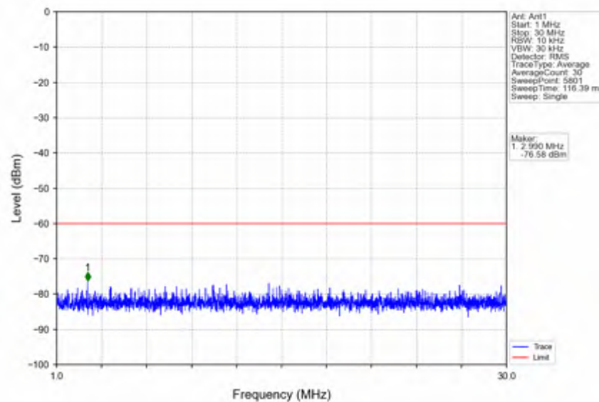
n78d_30kHz_SISO_NTNV_50MHz_CP-OFDM_QPSK_3675MHz_Inner_1RB_Right
