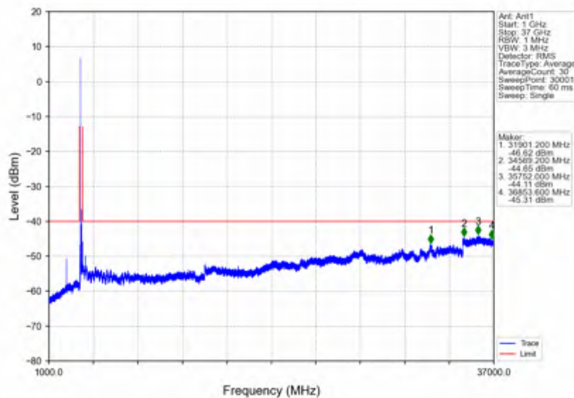
n78d_30kHz_SISO_NTNV_90MHz_DFT-s-OFDM_PI/2_BPSK_3595.02MHz_Outer_Full
