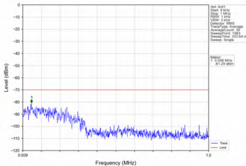
n78d_30kHz_SISO_NTNV_80MHz_CP-OFDM QPSK_3660MHz_Edge_1RB_Right
