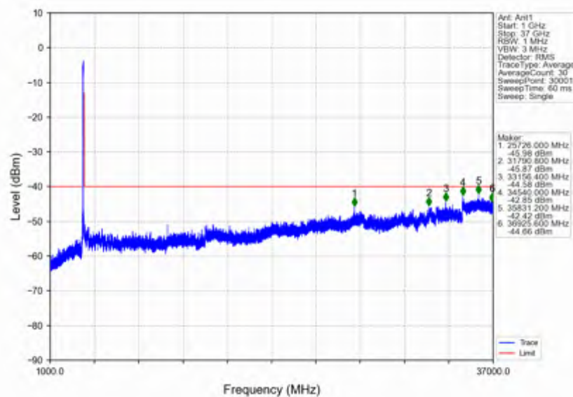
n78d_30kHz_SISO_NTNV_70MHz_CP-OFDM QPSK_3664.98MHz_Outer_Full
