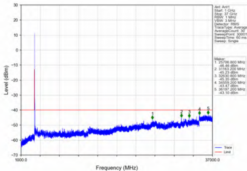
n78d_30kHz_SISO_NTV_60MHz_CP-OFDM QPSK_3624.99MHz_Edge_1RB_Left
