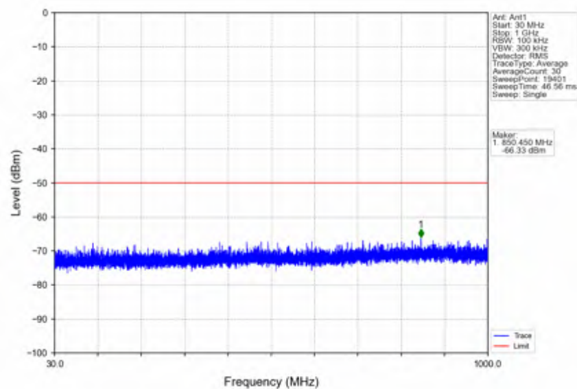
n78d_30kHz_SISO_NTNV_80MHz_DFT-s-OFDM_QPSK_3660MHz_Outer_Full
