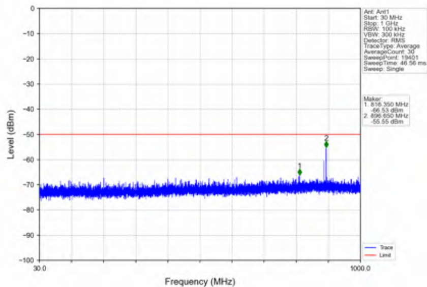
n78d_30kHz_SISO_NTNV_70MHz_CP-OFDM_QPSK_3585MHz_Outer_Full
