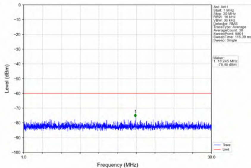
n78d_30kHz_SISO_NTNV_60MHz_CP-OFDM QPSK_3669.99MHz_Outer_Full
