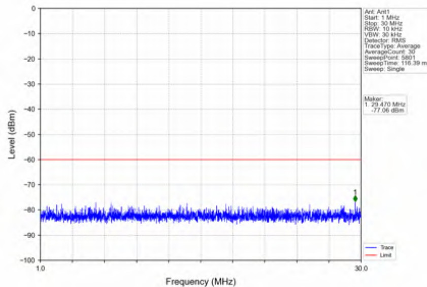
n78d_30kHz_SISO_NTNV_70MHz_DFT-s-OFDM_QPSK_3585MHz_Outer_Full
