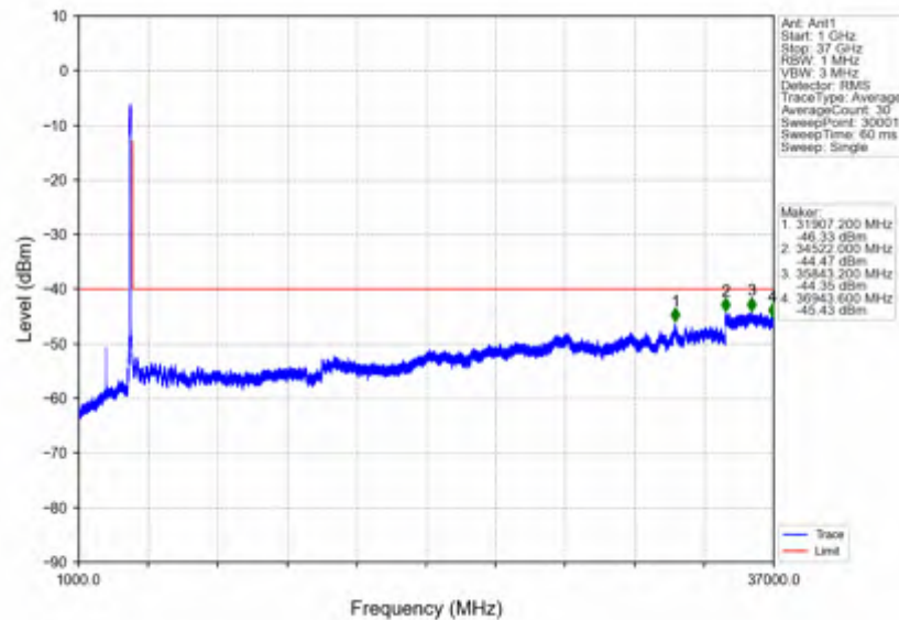
n78d_30kHz_SISO_NTNV_80MHz_DFT-s-OFDM_PI/2_BPSK_3660MHz_Outer_Full
