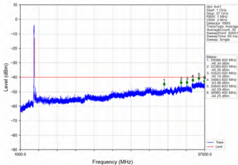
n78d_30kHz_SISO_NTNV_80MHz_DFT-s-OFDM QPSK_3660MHz_Inner_1RB_Right
