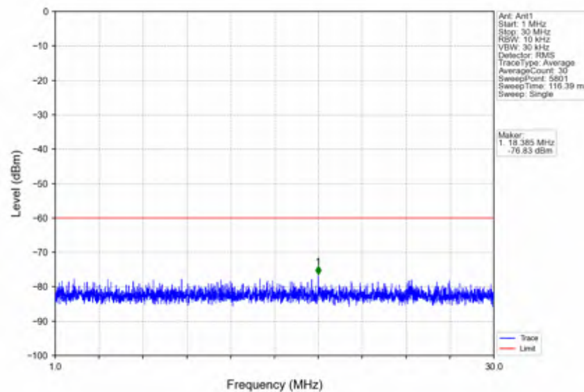
n78d_30kHz_SISO_NTNV_90MHz_DFT-s-OFDM_QPSK_3595.02MHz_Outer_Full
