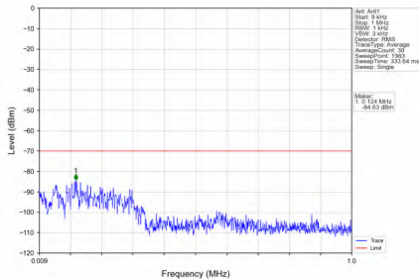
n78d_30kHz_SISO_NTNV_80MHz_DFT-s-OFDM QPSK_3660MHz_Edge_1RB_Right
