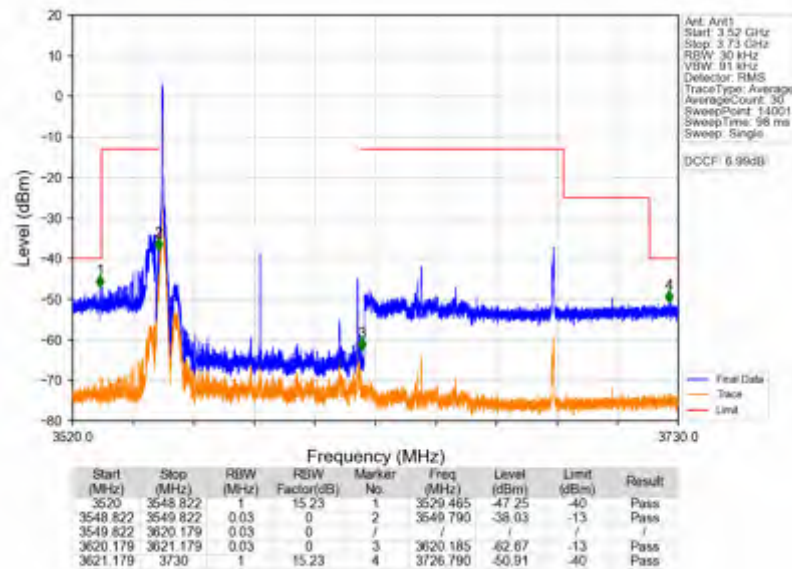
n78d_30kHz_SISO_NTNV_70MHz_DFT-s-OFDM_PI/2_BPSK_3585MHz_Edge_1RB_Left
