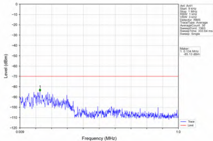
n78d_30kHz_SISO_NTNV_60MHz_DFT-s-OFDM QPSK_3669.99MHz_Inner_1RB_Right
