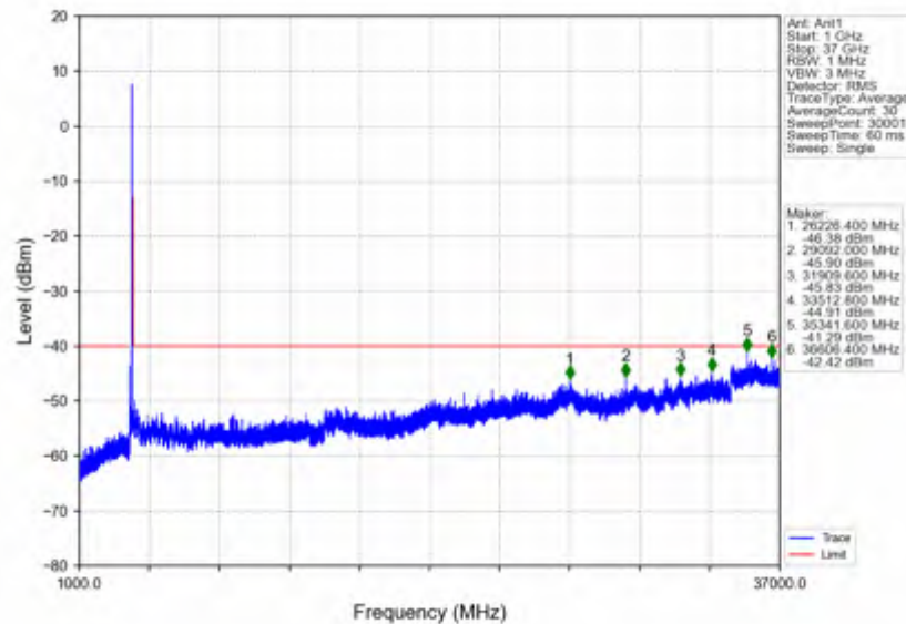
n78d_30kHz_SISO_NTNV_60MHz_DFT-s-OFDM QPSK_3669.99MHz_Inner_1RB_Right
