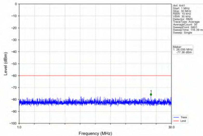
n78d_30kHz_SISO_NTNV_70MHz_CP-OFDM QPSK_3664.98MHz_Edge_1RB_Right
