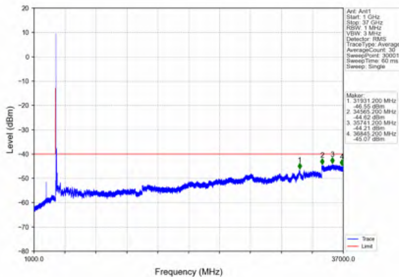
n78d_30kHz_SISO_NTNV_70MHz_DFT-s-OFDM_PI/2_BPSK_3624.99MHz_Edge_1RB_Left
