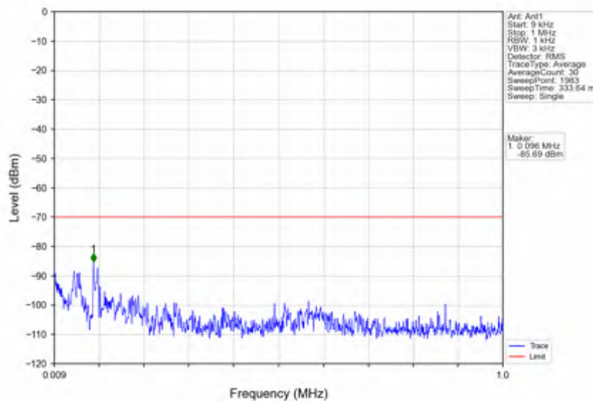
n78d_30kHz_SISO_NTNV_60MHz_DFT-s-OFDM_QPSK_3669.99MHz_Outer_Full
