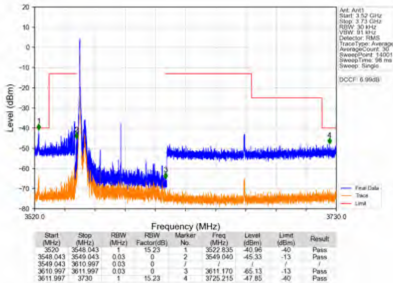
n78d_30kHz_SISO_NTNV_60MHz_DFT-s-OFDM_QPSK_3580.02MHz_Inner_1RB_Left
