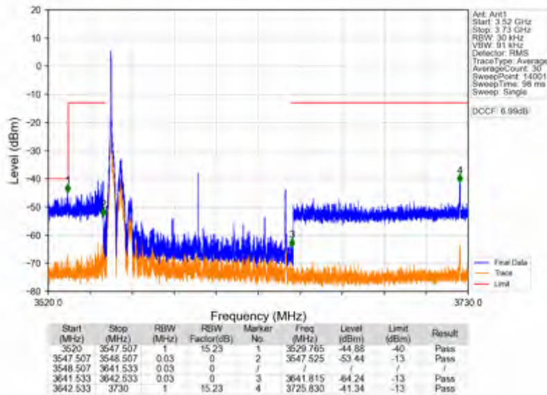
n78d_30kHz_SISO_NTNV_90MHz_DFT-s-OFDM_QPSK_3595.02MHz_Inner_1RB_Left
