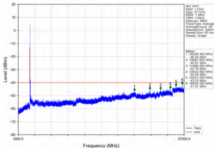
n78d_30kHz_SISO_NTNV_80MHz_CP-OFDM_QPSK_3590.01MHz_Outer_Full
