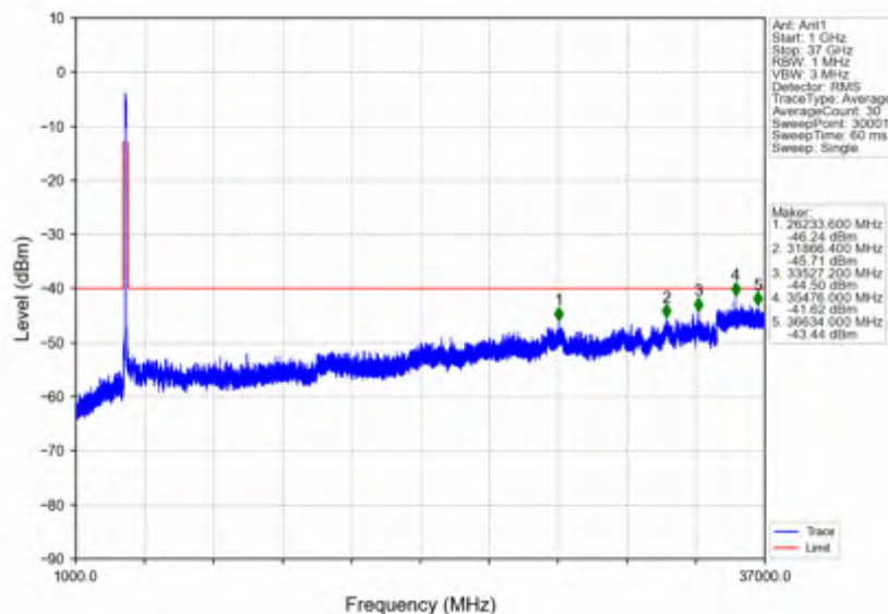
n78d_30kHz_SISO_NTNV_90MHz_DFT-s-OFDM_QPSK_3595.02MHz_Inner_1RB_Left
