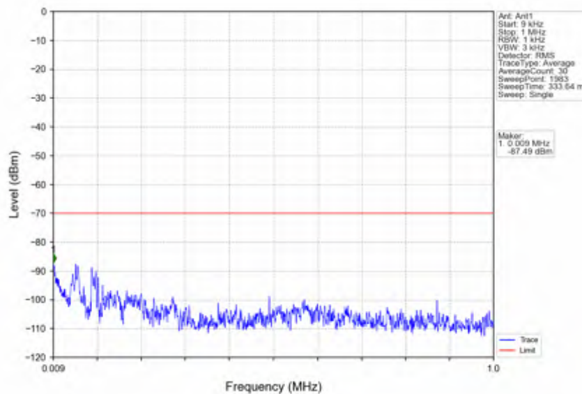
n78d_30kHz_SISO_NTNV_80MHz_DFT-s-OFDM_QPSK_3590.01MHz_Outer_Full
