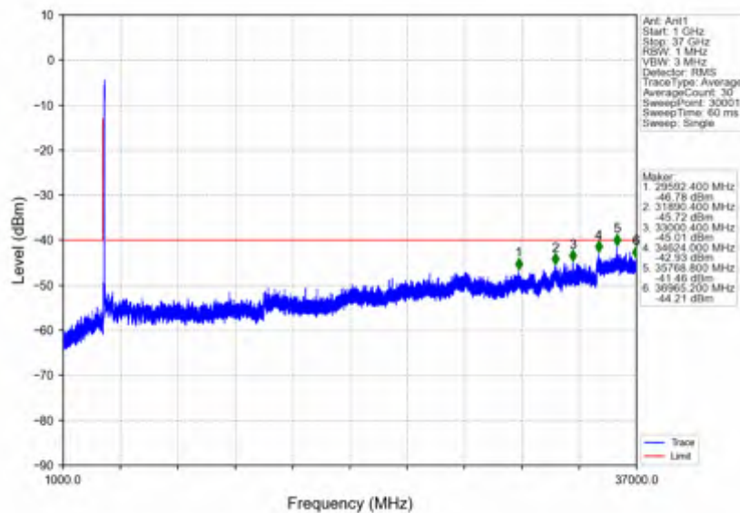
n78d_30kHz_SISO_NTNV_60MHz_DFT-s-OFDM_QPSK_3580.02MHz_Inner_1RB_Left
