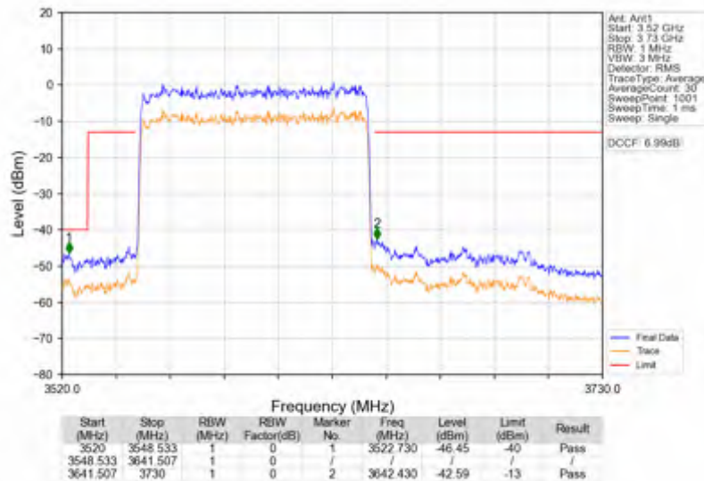
n78d_30kHz_SISO_NTNV_90MHz_DFT-s-OFDM_PI/2_BPSK_3595.02MHz_Outer_Full
