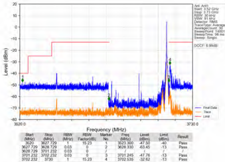
n78d_30kHz_SISO_NTNV_70MHz_DFT-s-OFDM QPSK_3664.98MHz_Inner_1RB_Right
