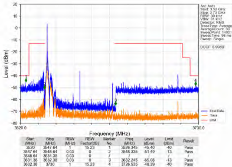
n78d_30kHz_SISO_NTNV_80MHz_DFT-s-OFDM_QPSK_3590.01MHz_Inner_1RB_Left
