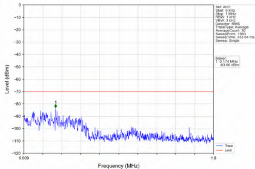
n78d_30kHz_SISO_NTNV_60MHz_DFT-s-OFDM QPSK_3669.99MHz_Edge_1RB_Right
