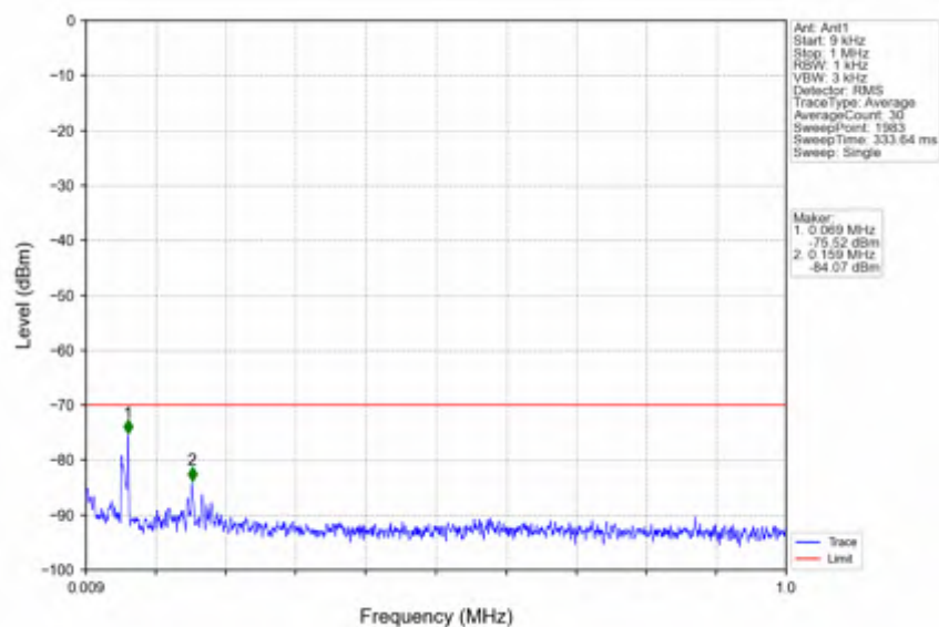
n78d_30kHz_SISO_NTNV_70MHz_DFT-s-OFDM_PI/2_BPSK_3585MHz_Edge_1RB_Left
