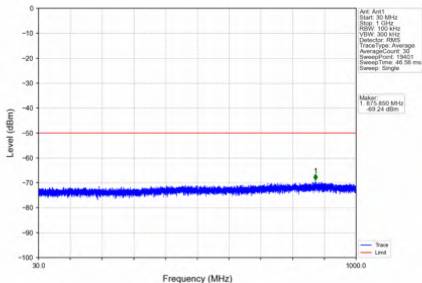
n78d_30kHz_SISO_NTNV_70MHz_DFT-s-OFDM QPSK_3664.98MHz_Edge_1RB_Right
