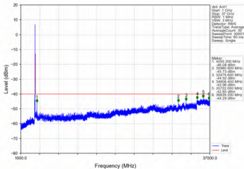
n78d_30kHz_SISO_NTNV_80MHz_CP-OFDM QPSK_3660MHz_Outer_Full
