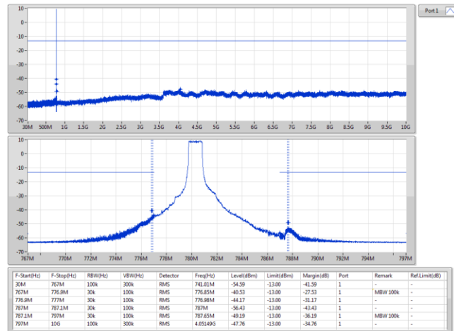
Band 13 LTE-M1_5MHz_Nss1_1TX 782MHz_16QAM_RB 6,#RB 0,NB 0
