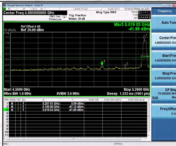
11N20MIMO_Ant1_High_5320
