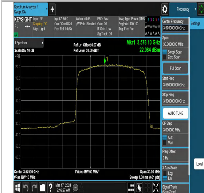
42(3550-3600)-10MHz-QPSK-43340-1RB#49-PASS
