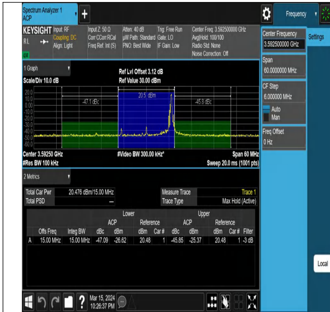
42(3550-3600)-15MHz-16QAM-43515-1RB#74-PASS
