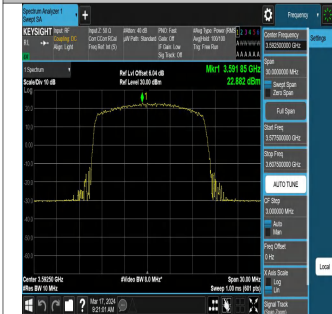
42(3550-3600)-15MHz-QPSK-43515-1RB#38-PASS
