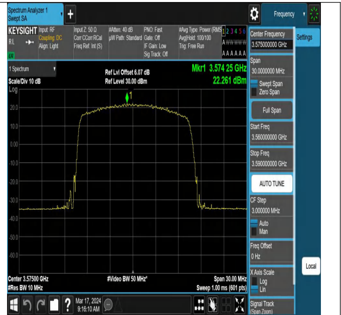
42(3550-3600)-10MHz-QPSK-43340-1RB#24-PASS
