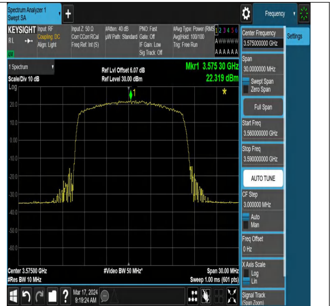
42(3550-3600)-15MHz-QPSK-43340-1RB#38-PASS
