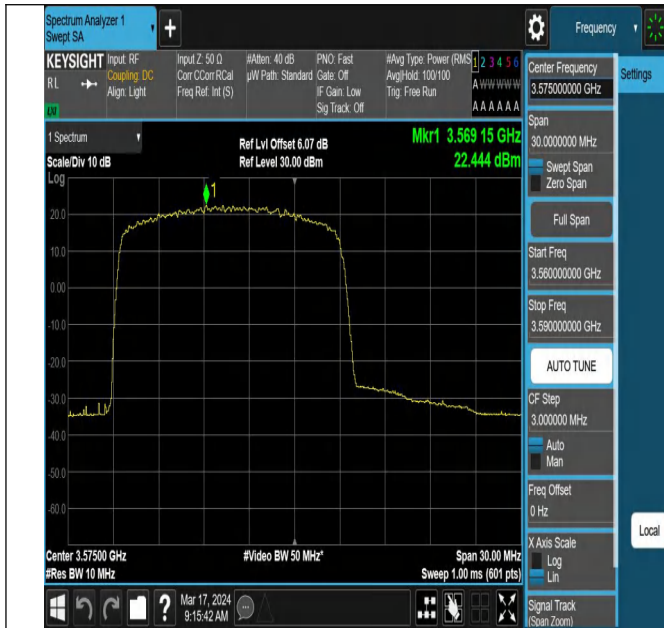
42(3550-3600)-10MHz-QPSK-43340-1RB#0-PASS
