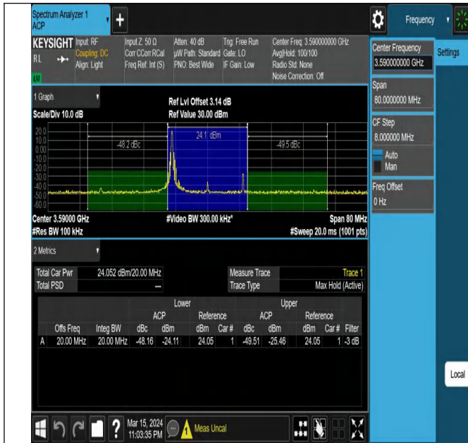
42(3550-3600)-20MHz-QPSK-43490-1RB#0-PASS
