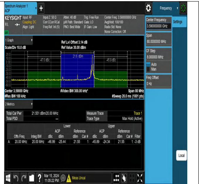
42(3550-3600)-20MHz-QPSK-43490-1RB#99-PASS
