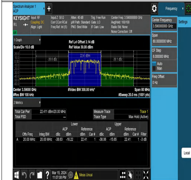
42(3550-3600)-20MHz-QPSK-43490-100RB#0-PASS
