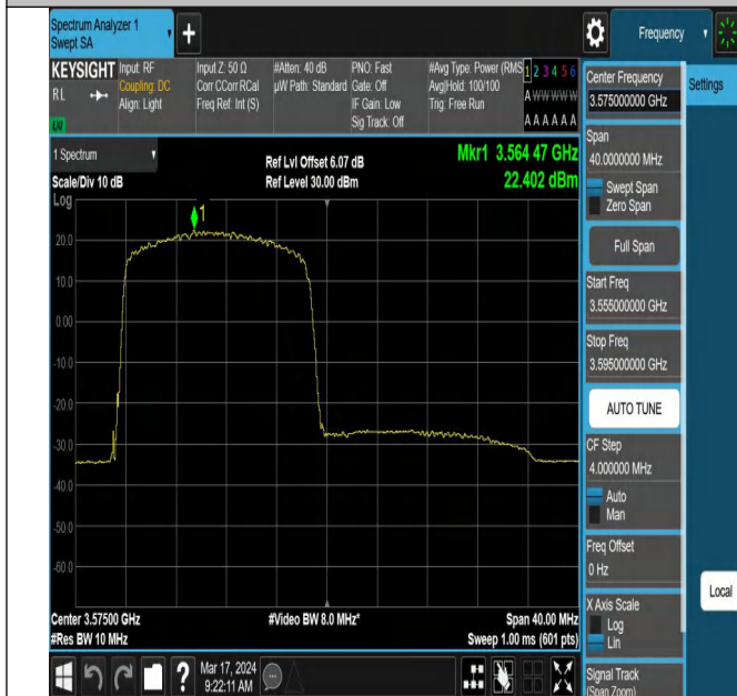
42(3550-3600)-20MHz-QPSK-43340-1RB#0-PASS
