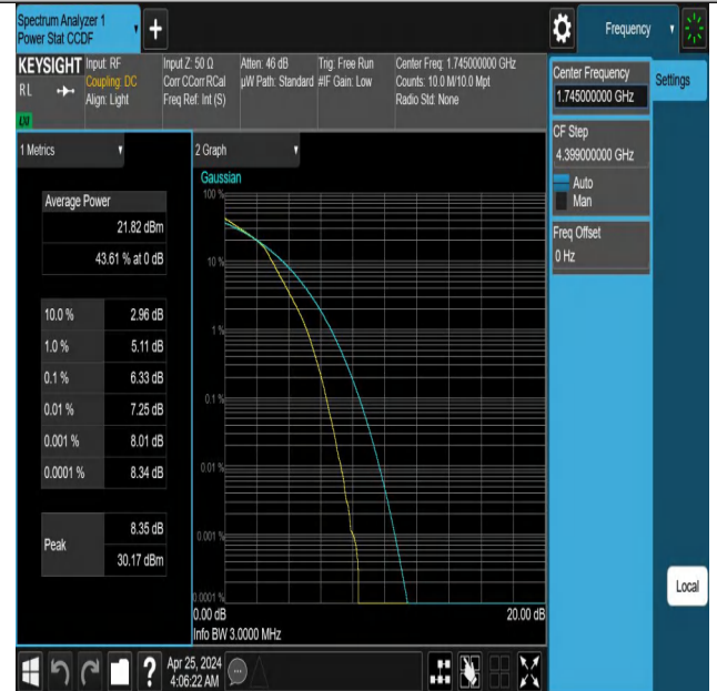
Band66-3MHz-16QAM-132322-15RB#0-PASS
