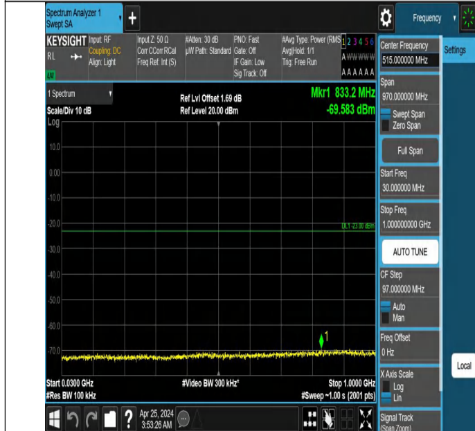
Band66_1.4MHz_QPSK_131979_1RB#0_30~1000_30~1000
