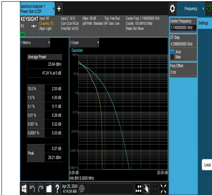
Band66-5MHz-QPSK-132322-1RB#0-PASS
