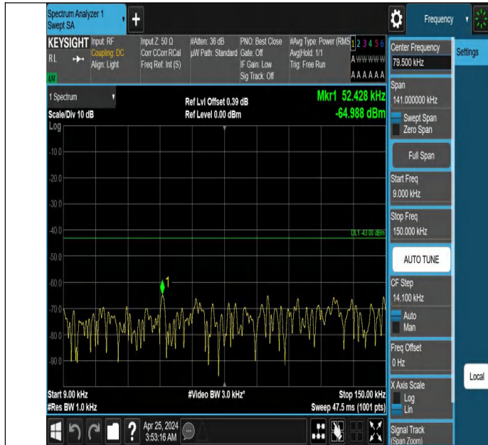
Band66_1.4MHz_QPSK_131979_1RB#0_0.009~0.15_0.009~0.15
