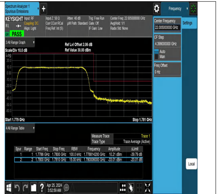
Band66_1.4MHz_QPSK_132665_6RB#0
