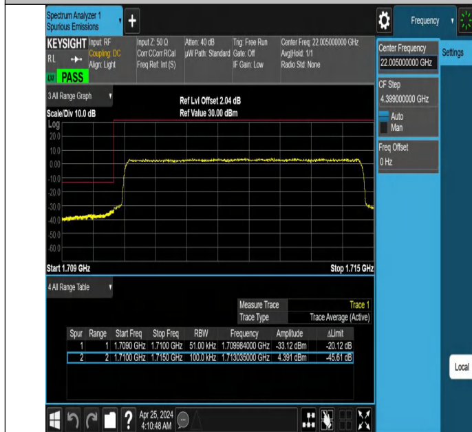
Band66_5MHz_QPSK_131997_25RB#0
