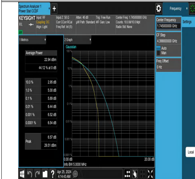
Band66-5MHz-16QAM-132322-1RB#0-PASS
