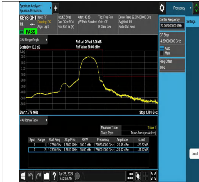
Band66_1.4MHz_QPSK_132665_1RB#5
