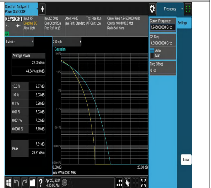
Band66-5MHz-16QAM-132322-25RB#0-PASS
