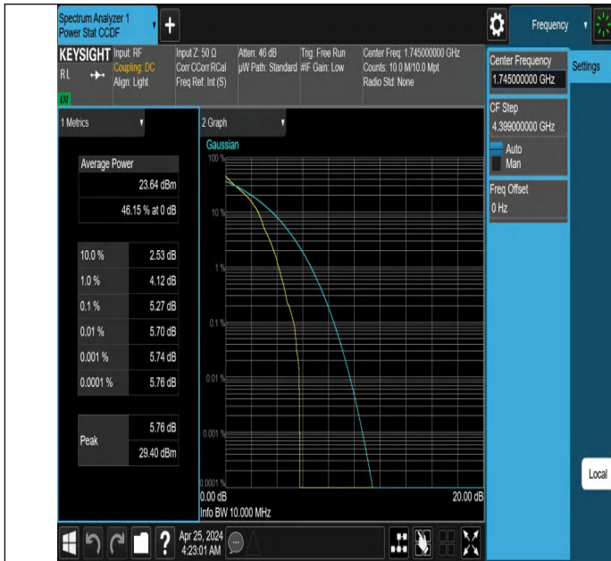
Band66-10MHz-QPSK-132322-1RB#0-PASS
