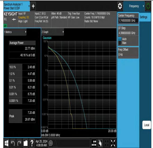
Band66-3MHz-QPSK-132322-15RB#0-PASS
