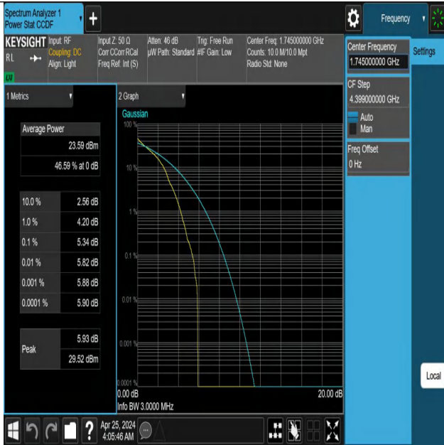
Band66-3MHz-QPSK-132322-1RB#0-PASS
