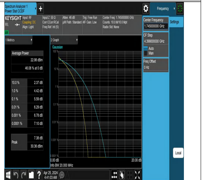
Band66-20MHz-QPSK-132322-100RB#0-PASS
