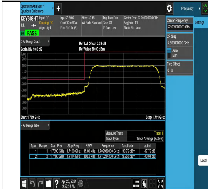
Band66_1.4MHz_QPSK_131979_6RB#0
