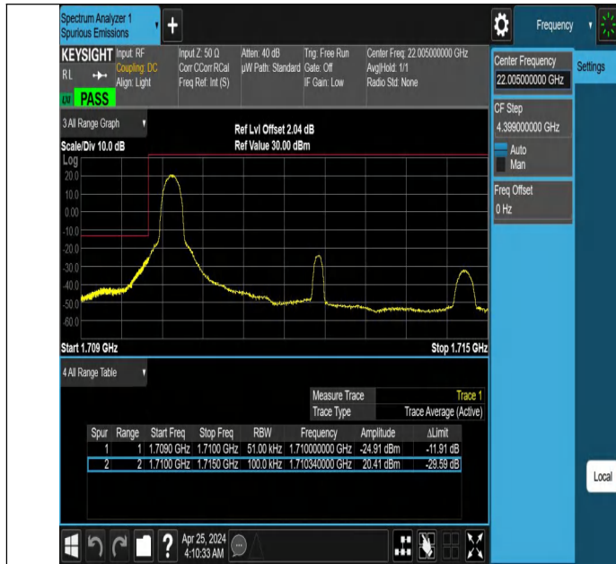
Band66_5MHz_QPSK_131997_1RB#0
