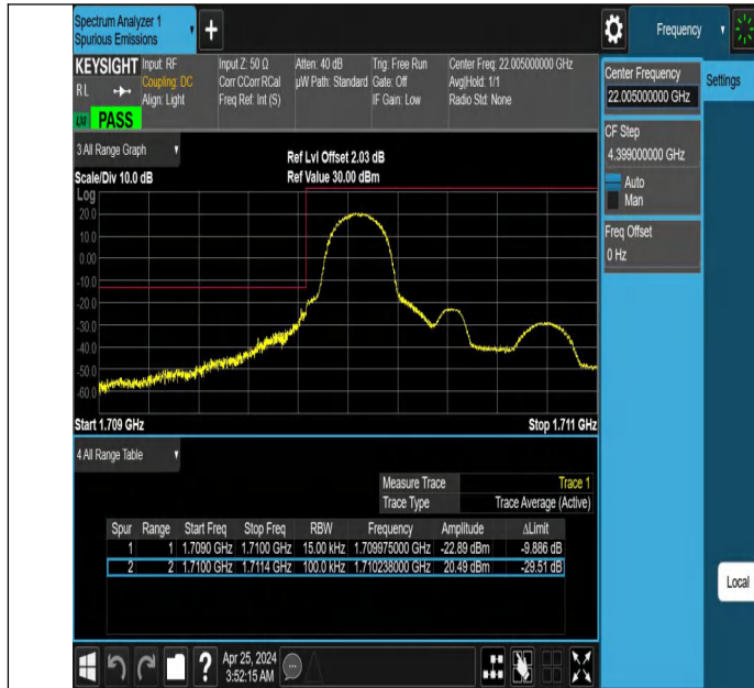
Band66_1.4MHz_QPSK_131979_1RB#0
