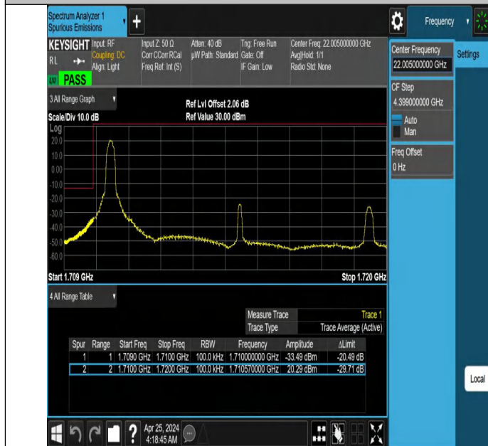
Band66_10MHz_QPSK_132022_1RB#0
