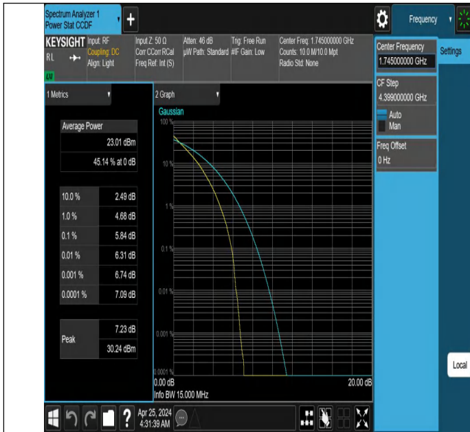
Band66-15MHz-QPSK-132322-75RB#0-PASS
