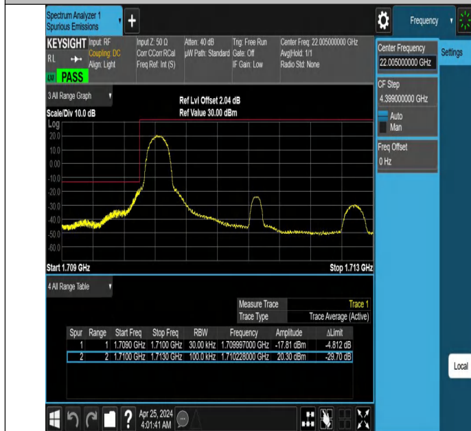
Band66_3MHz_QPSK_131987_1RB#0
