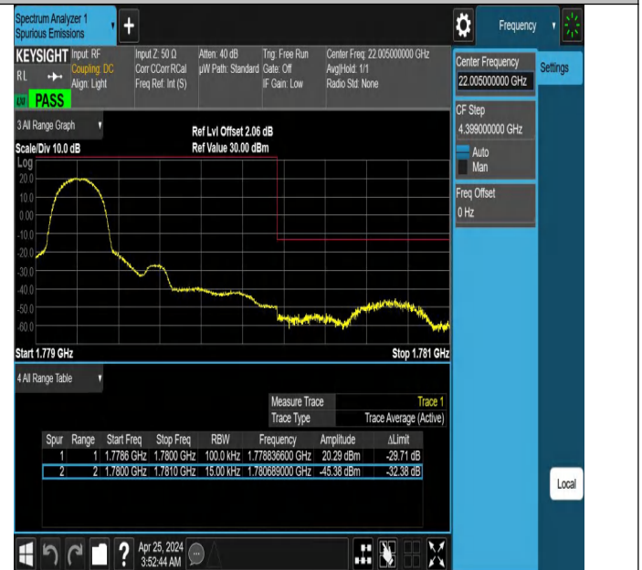
Band66_1.4MHz_QPSK_132665_1RB#0
