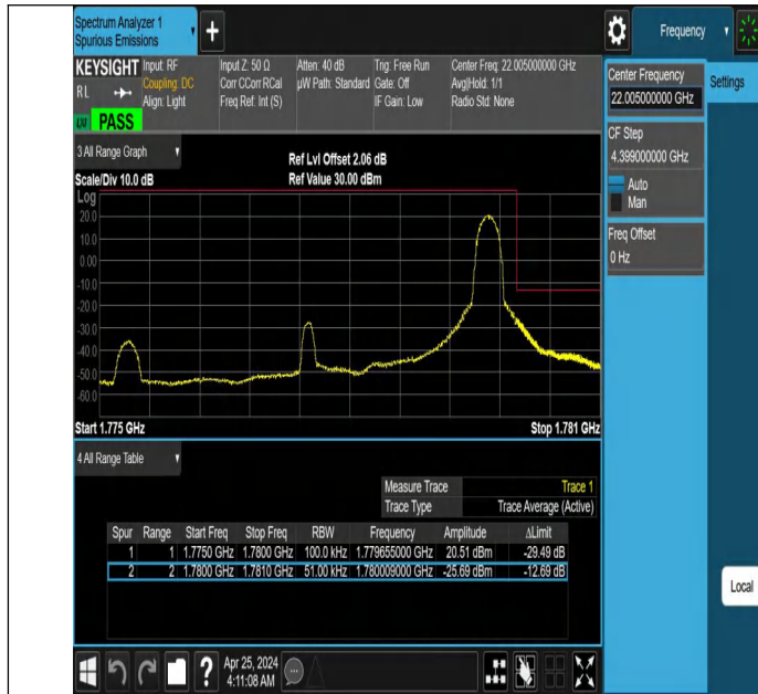
Band66_5MHz_QPSK_132647_1RB#24
