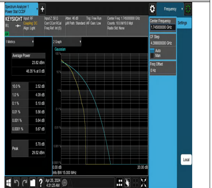
Band66-15MHz-QPSK-132322-1RB#0-PASS
