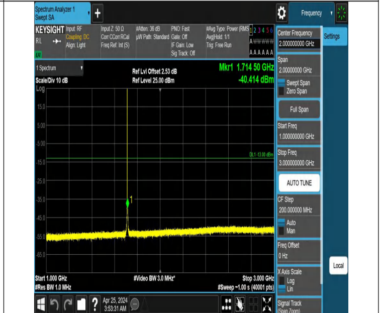
Band66_1.4MHz_QPSK_131979_1RB#0_1000~3000_1000~3000
