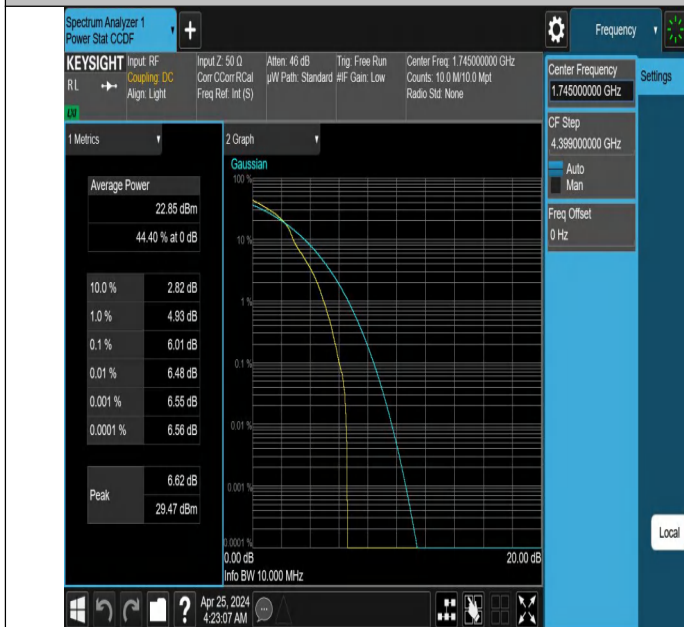
Band66-10MHz-16QAM-132322-1RB#0-PASS
