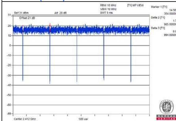
802.11ax (RU26)
