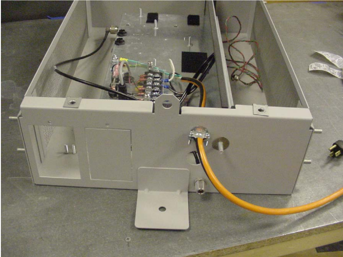
Exterior bottom of NEMA enclosure with cover removed
