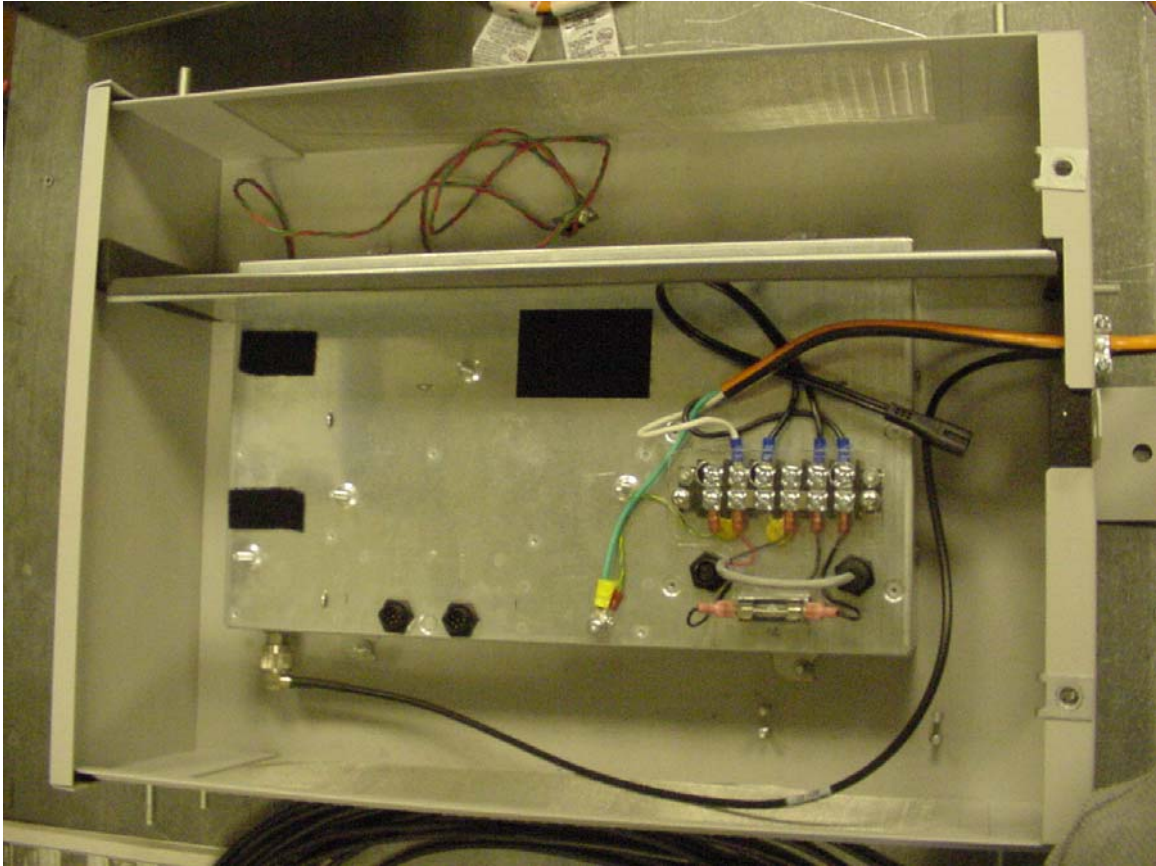
NEMA enclosure with cover removed showing setup without RF amp.
