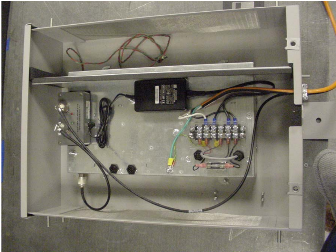
NEMA enclosure with cover removed showing setup with RF amp.
