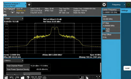
11AX20SISO-Ant1-2437-106Tone-RU53-PASS
