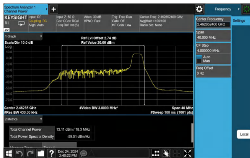
11AX20SISO-Ant1-2462-106Tone-RU54-PASS
