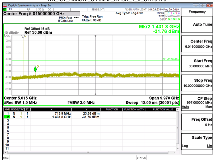
NB_IoT_Band12_3.75kHz_BPSK_1_0_CH23179
