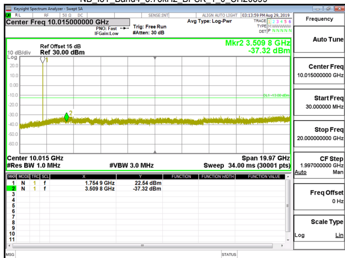
NB_IoT_Band4_3.75kHz_BPSK_1_0_CH20399
