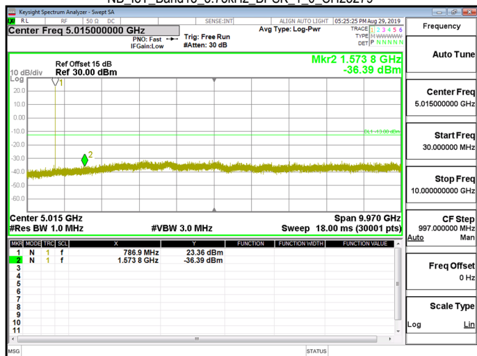
NB_IoT_Band13_3.75kHz_BPSK_1_0_CH23279
