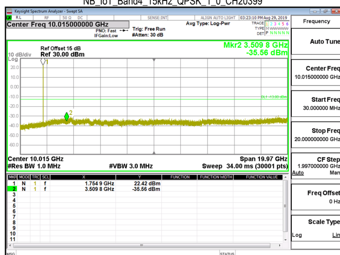
NB_IoT_Band4_15kHz_QPSK_1_0_CH20399
