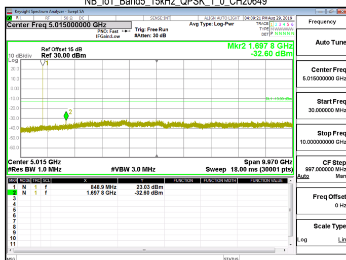
NB_IoT_Band5_15kHz_QPSK_1_0_CH20649
