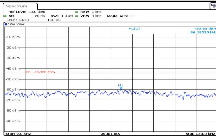
Band4-1.4MHz-QPSK-19957-1RB#0-Range1:0.009~0.15MHz
