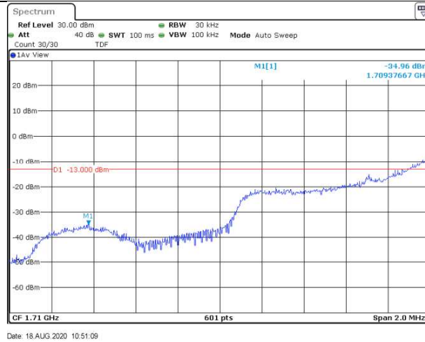
Band4-1.4MHz-16QAM-19957-6RB#0
