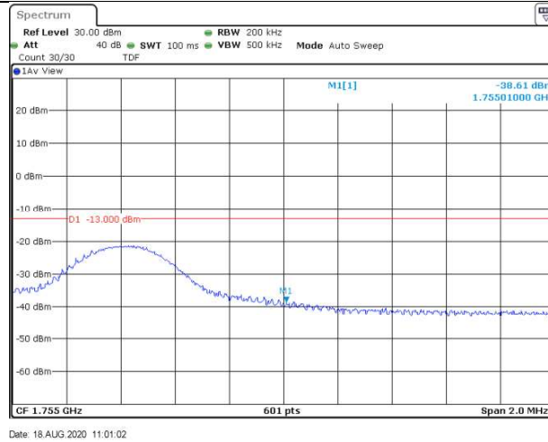
Band4-10MHz-QPSK-20350-50RB#0
