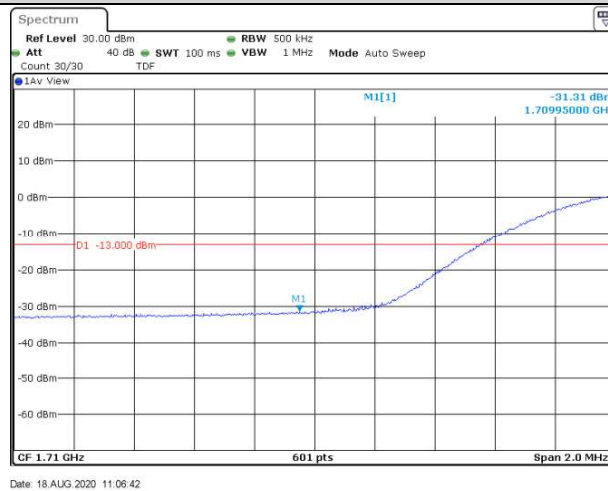
Band4-20MHz-16QAM-20300-1RB#0
