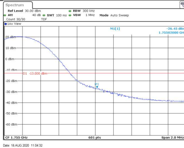
Band4-15MHz-QPSK-20325-75RB#0
