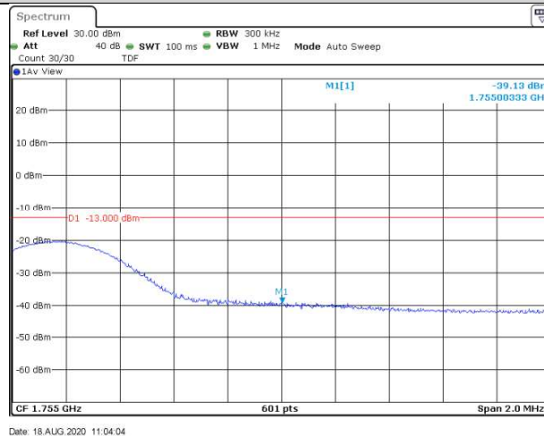
Band4-15MHz-QPSK-20325-1RB#74
