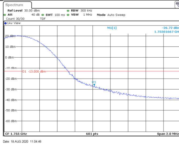
Band4-15MHz-16QAM-20325-75RB#0
