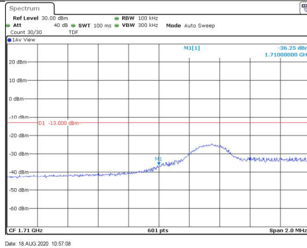
Band4-5MHz-16QAM-19975-25RB#0
