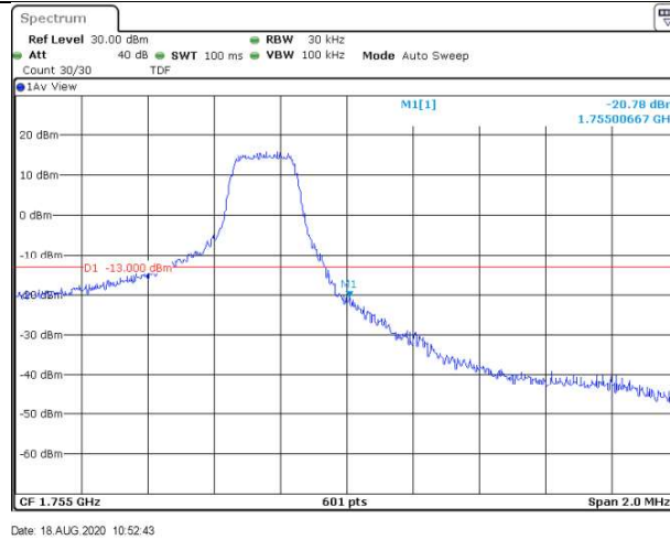
Band4-1.4MHz-16QAM-20393-6RB#0
