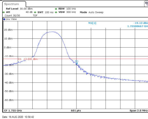
Band4-5MHz-16QAM-20375-25RB#0
