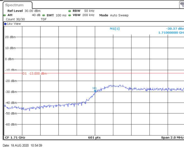
Band4-3MHz-16QAM-19965-15RB#0
