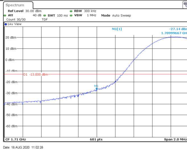
Band4-15MHz-QPSK-20025-75RB#0
