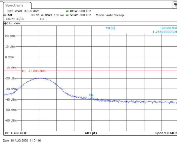
Band4-10MHz-16QAM-20350-1RB#49
