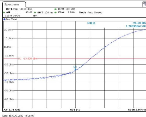
Band4-20MHz-16QAM-20050-1RB#99
