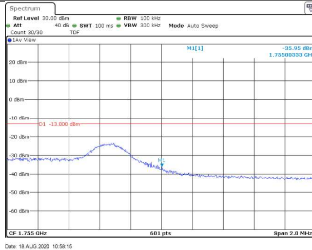
Band4-5MHz-16QAM-20375-1RB#24
