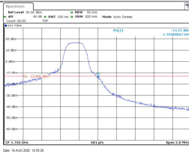
Band4-3MHz-QPSK-20385-1RB#0
