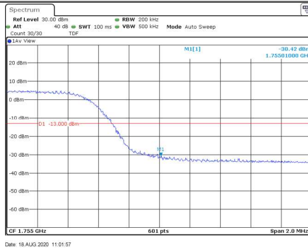
Band4-10MHz-16QAM-20000-1RB#49
