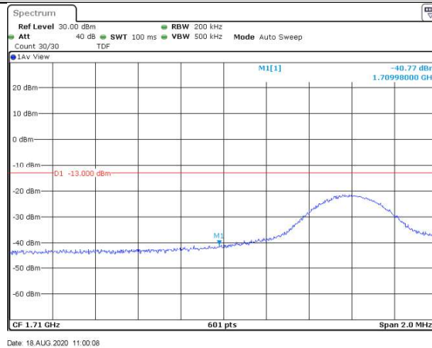
Band4-10MHz-16QAM-20000-1RB#0
