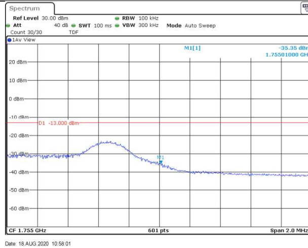
Band4-5MHz-QPSK-20375-25RB#0
