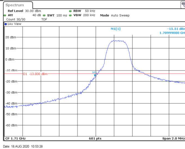
Band4-3MHz-QPSK-19965-15RB#0
