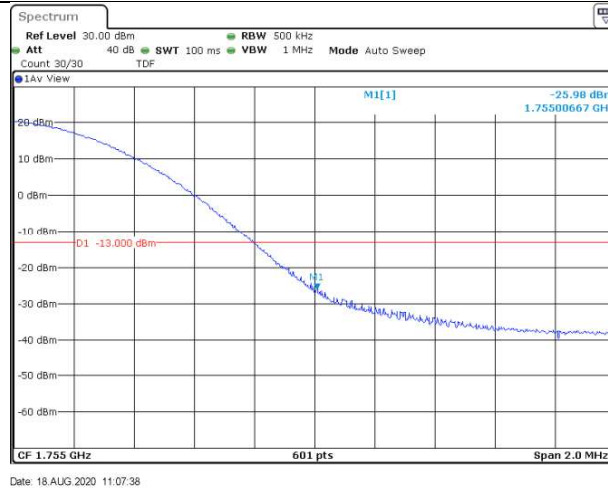
Band4-20MHz-QPSK-20300-100RB#0
