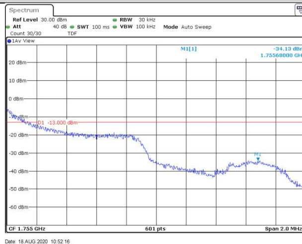
Band4-1.4MHz-16QAM-20393-1RB#5
