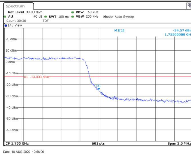
Band4-5MHz-QPSK-19975-1RB#24
