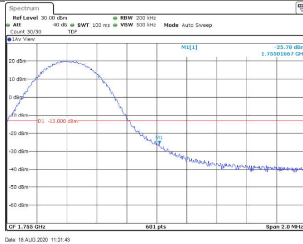
Band4-10MHz-16QAM-20350-50RB#0
