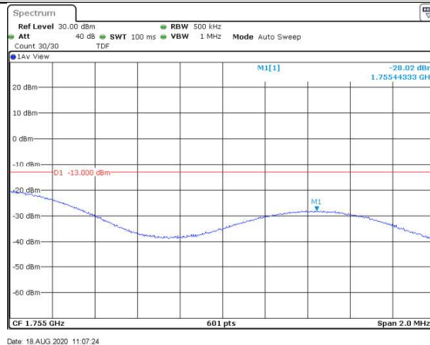
Band4-20MHz-16QAM-20300-1RB#99
