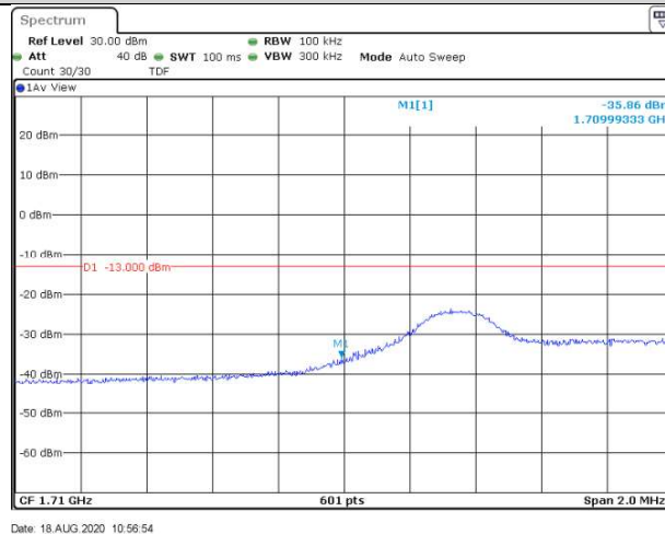
Band4-5MHz-QPSK-19975-1RB#0
