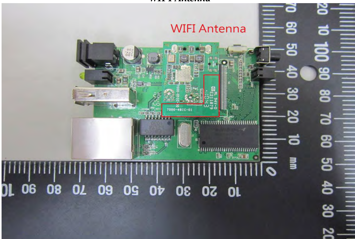
WIFI Antenna
