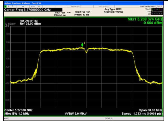
IEEE 802.11n Channel 54 40MHz Antenna 3
