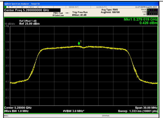
IEEE 802.11n Channel 56 20MHz Antenna 3
