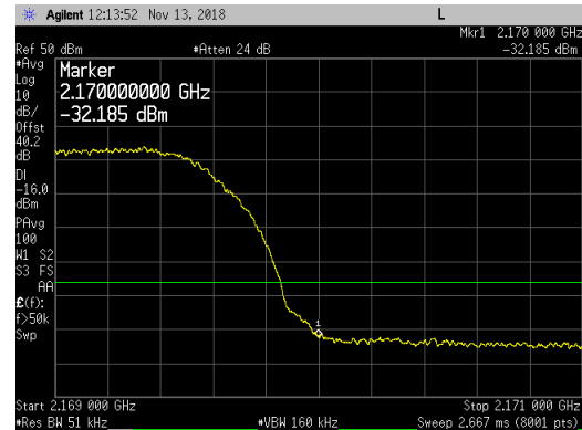
Port 2_UBE_2169 to 2171MHz
