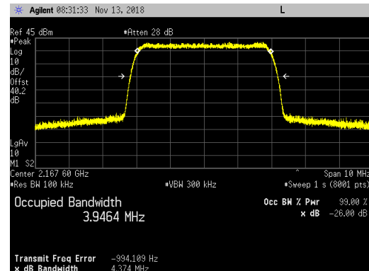
Top Channel_2167.6MHz_16QAM Modulation
