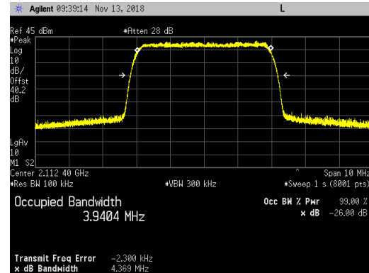
Bottom Channel_2112.4MHz_16QAM Modulation
