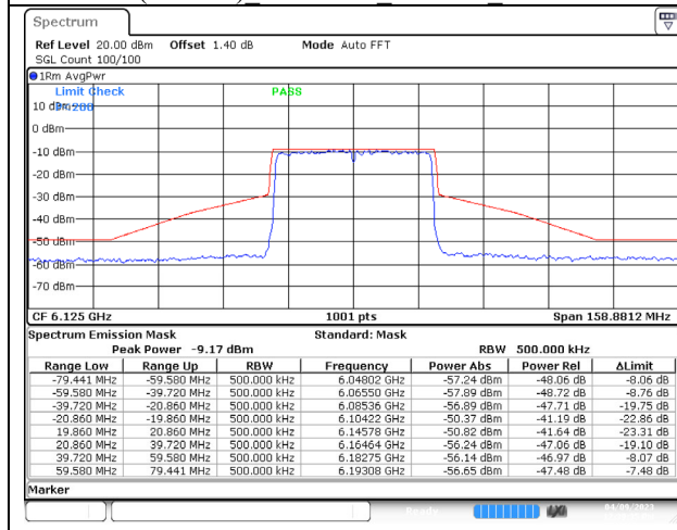
802.11ax (40MHz) 6125MHz Chain A NSS-4
