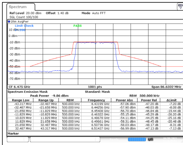
802.11ax (20MHz) 6475MHz Chain C NSS-4
