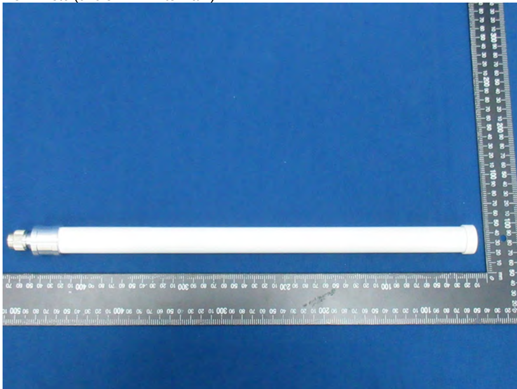
(10) EUT Photo (926.3 MHz Antenna 1)
