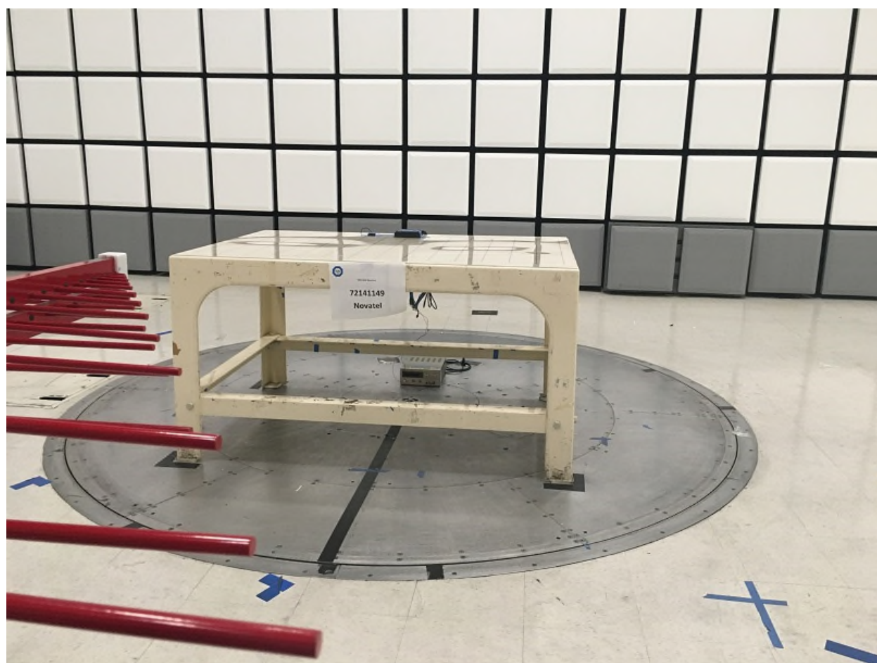
FCC Part 15B Radiated Emissions Test Setup (below 1GHz)
