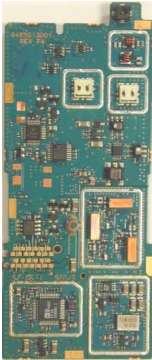
RF BOARD , less shields (TOP VIEW)
