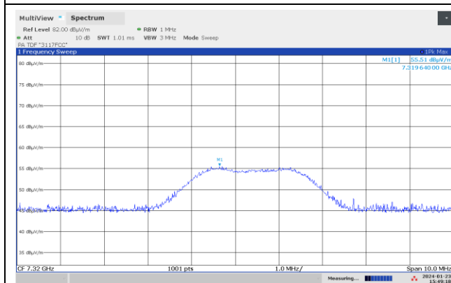
Spurious 7320 MHz, 2440, EUT H, Max: HP, Peak
