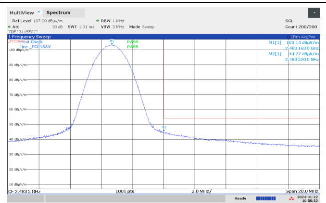
Upper Band Edge, 2480 MHz, 1Mb, Average
