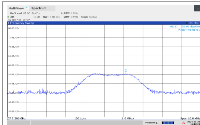
Spurious 7206 MHz, 2402, EUT H, Max: HP, Peak
