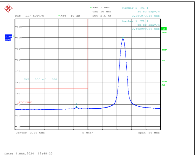
Lower Band Edge, 2402 MHz, 1Mb, Average
