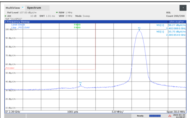
Lower Band Edge, 2402 MHz, 1Mb, Average
