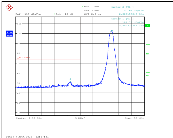
Lower Band Edge, 2402 MHz, 1Mb, Peak
