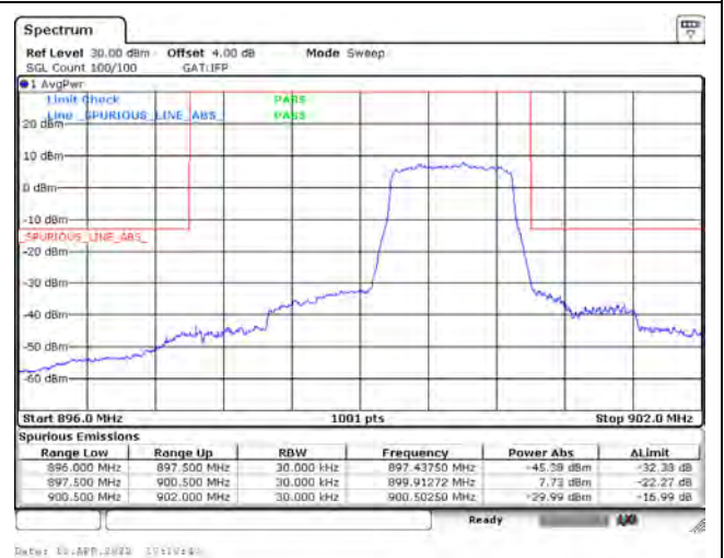
3 MHz / QPSK - Low / CH21640 / 6RB0
