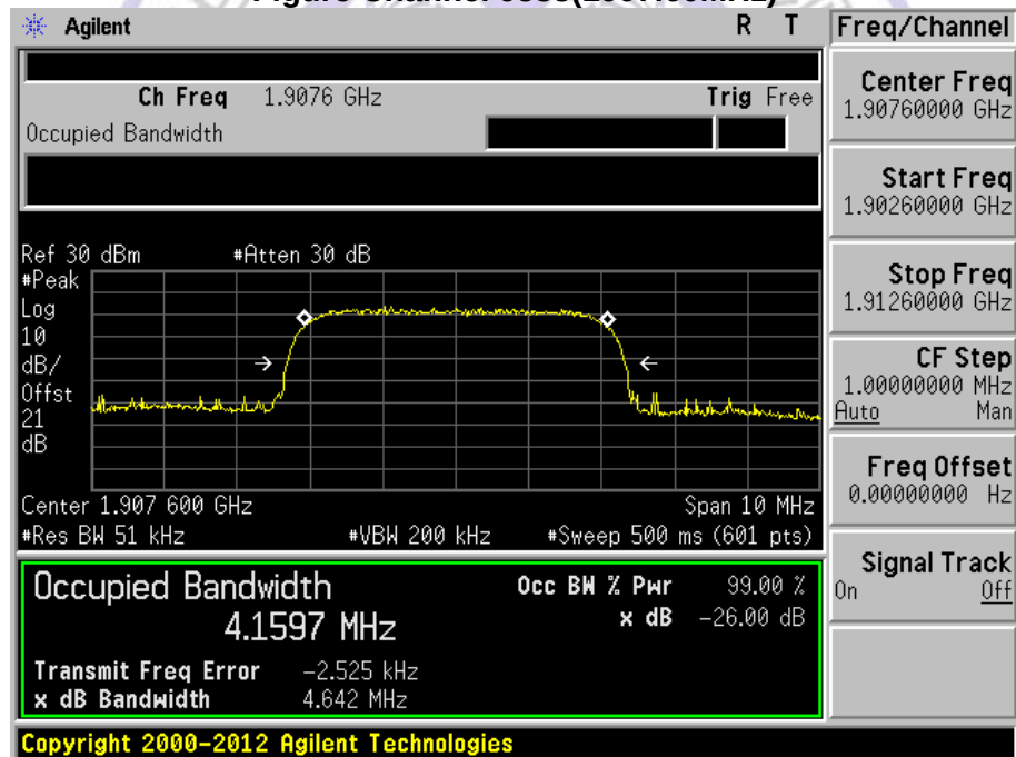
Figure Channel 9538(1907.60MHz)
