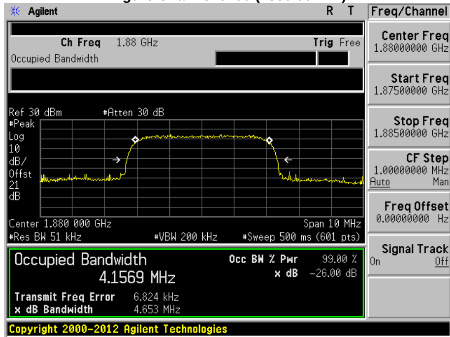
Figure Channel 9400 (1880.00MHz)
