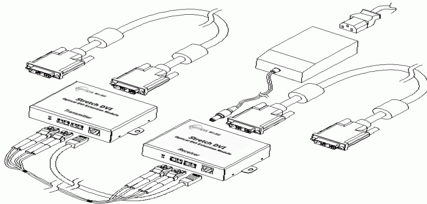
Figure 1 – Overall Optical DVI Module
