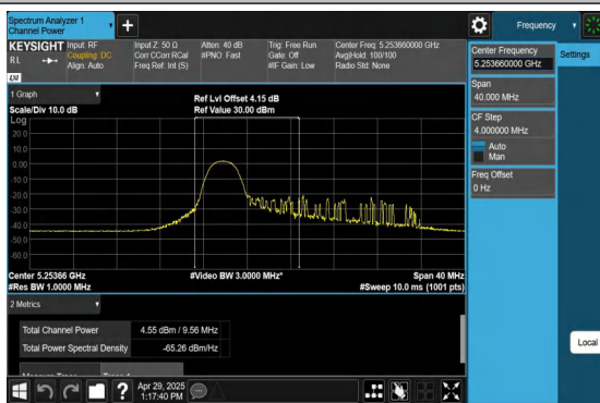
11AX20MIMO-Ant1-5260-TPC_H-52Tone-RU37-PASS
