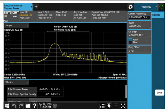
11AX20MIMO-Ant2-5260-TPC_H-52Tone-RU37-PASS
