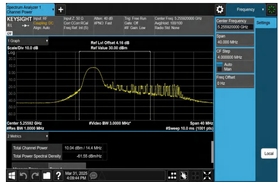
11AX20MIMO-Ant2-5260-TPC_L-26Tone-RU0-PASS
