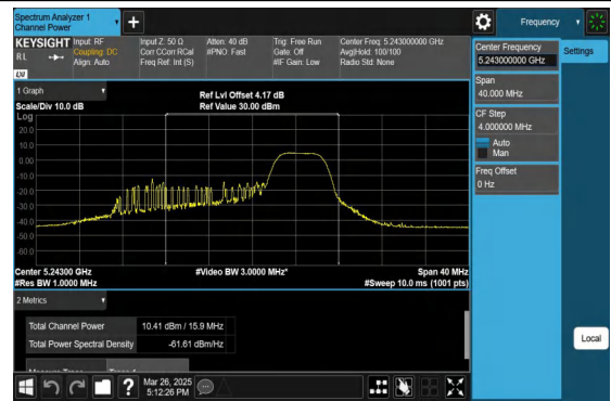
11AX20MIMO-Ant2-5240-106Tone-RU54-PASS
