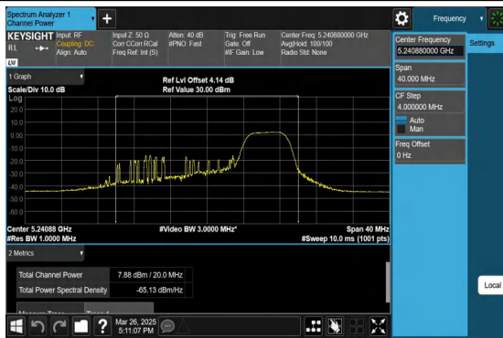
11AX20MIMO-Ant1-5240-106Tone-RU54-PASS
