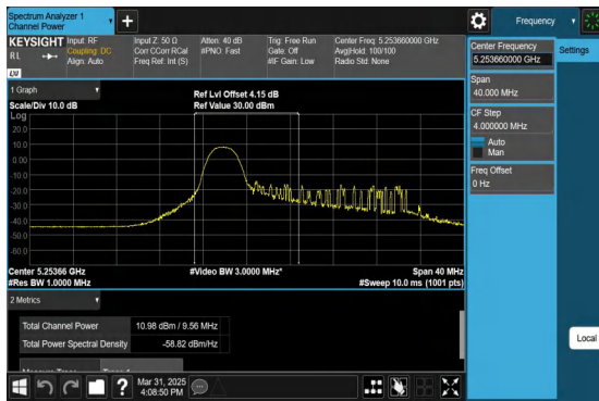
11AX20MIMO-Ant1-5260-TPC_L-26Tone-RU0-PASS
