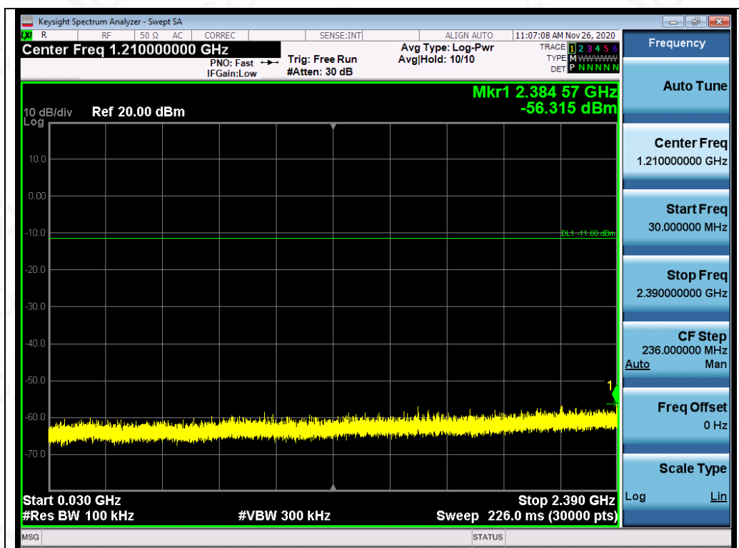
Test_Graph_EDR_2402_2Mbps_Lower Band Emissions
