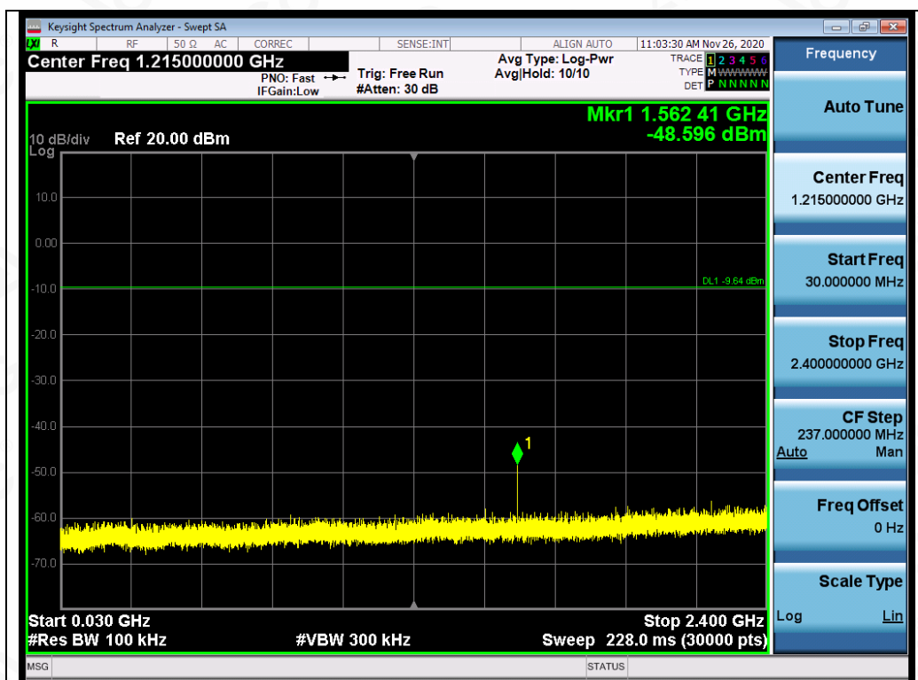
Test_Graph_BR_2441_1Mbps_Lower Band Emissions
