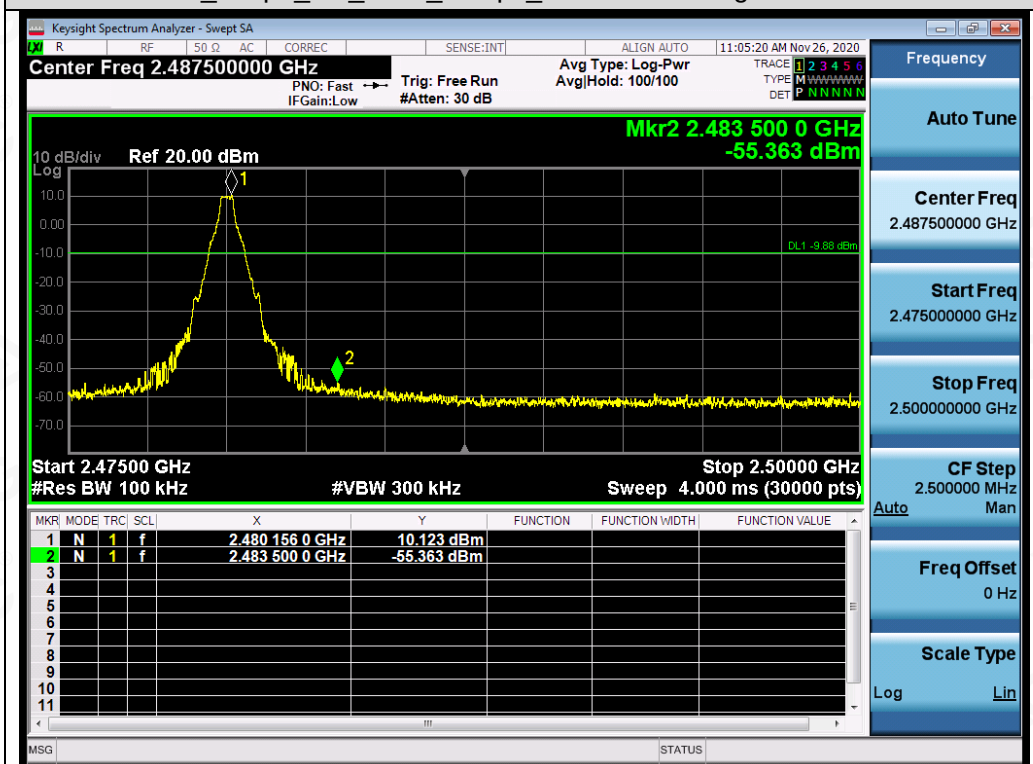
Test_Graph_BR_2480_1Mbps_Higher Band Edge Emissions
