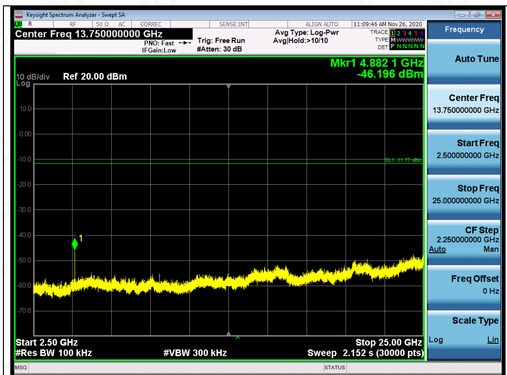
Test_Graph_EDR_2441_2Mbps_Higher Band Emissions
