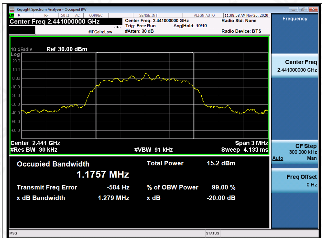
Test_Graph_EDR_2441_2Mbps_OBW
