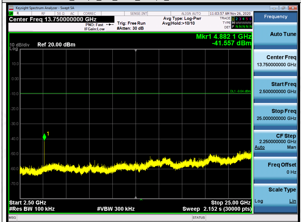
Test_Graph_BR_2441_1Mbps_Higher Band Emissions
