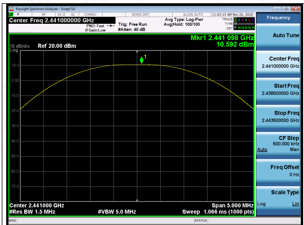
Test_Graph_BR_2441_1Mbps_Peak Power
