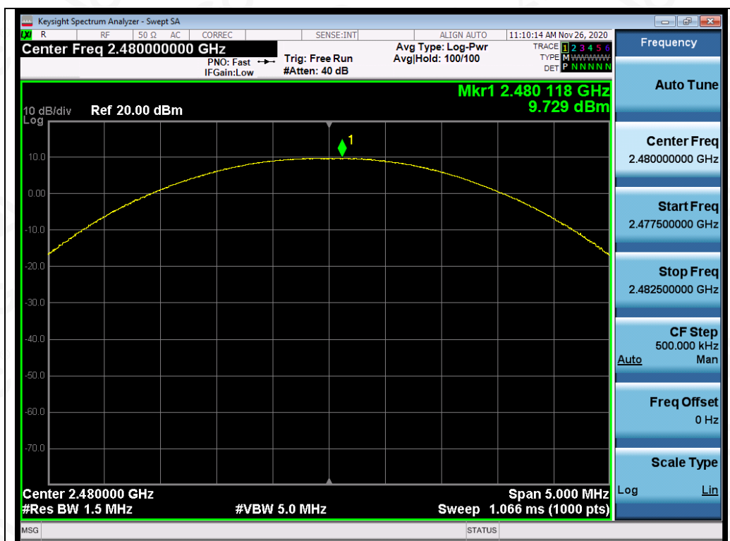
Test_Graph_EDR_2480_2Mbps_Peak Power
