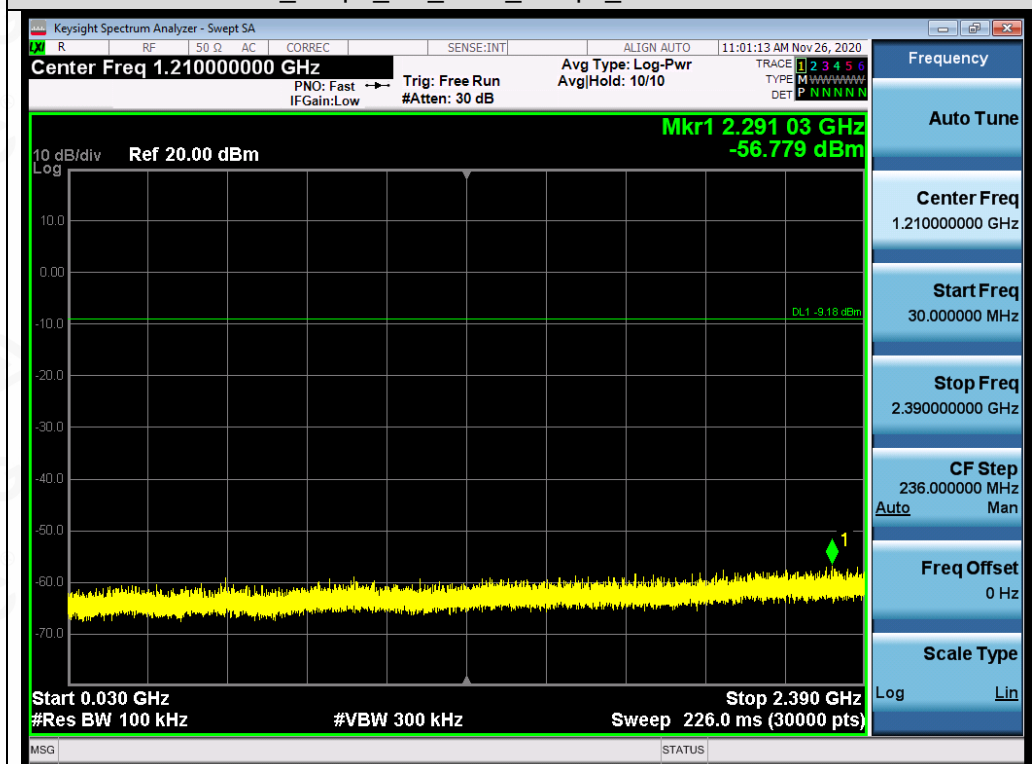
Test_Graph_BR_2402_1Mbps_Lower Band Emissions
