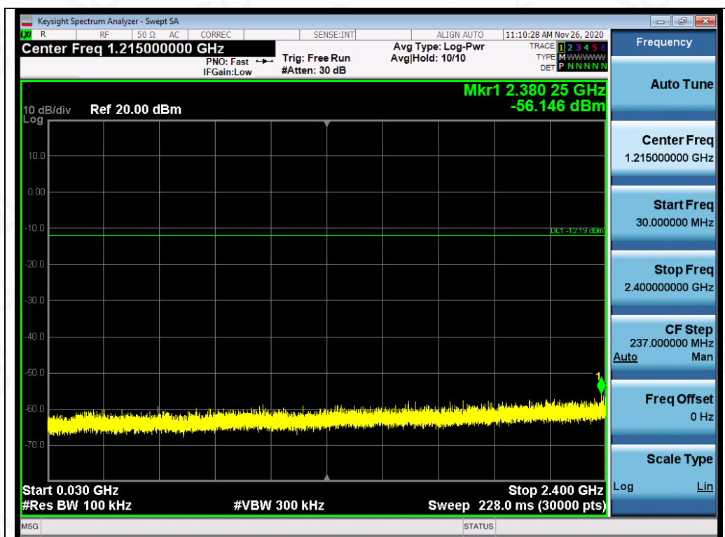
Test_Graph_EDR_2480_2Mbps_Lower Band Emissions
