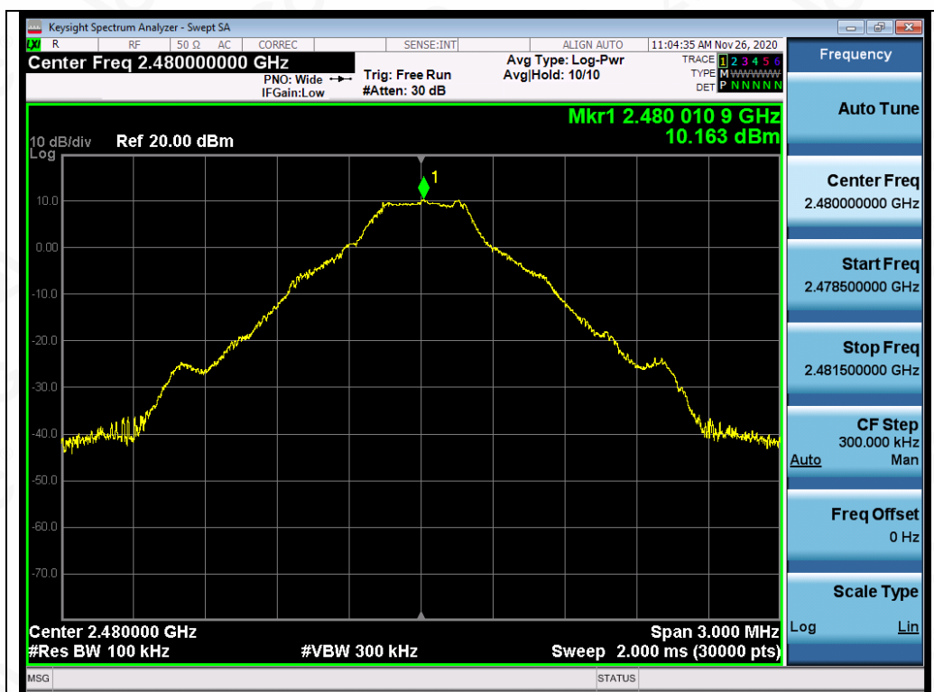
Test_Graph_BR_2480_1Mbps_Reference Level
