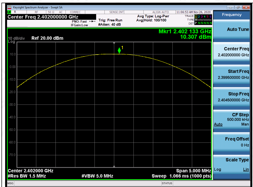
Test_Graph_EDR_2402_2Mbps_Peak Power
