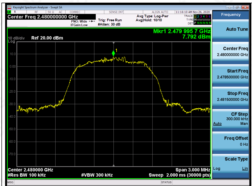
Test_Graph_EDR_2480_3Mbps_Reference Level
