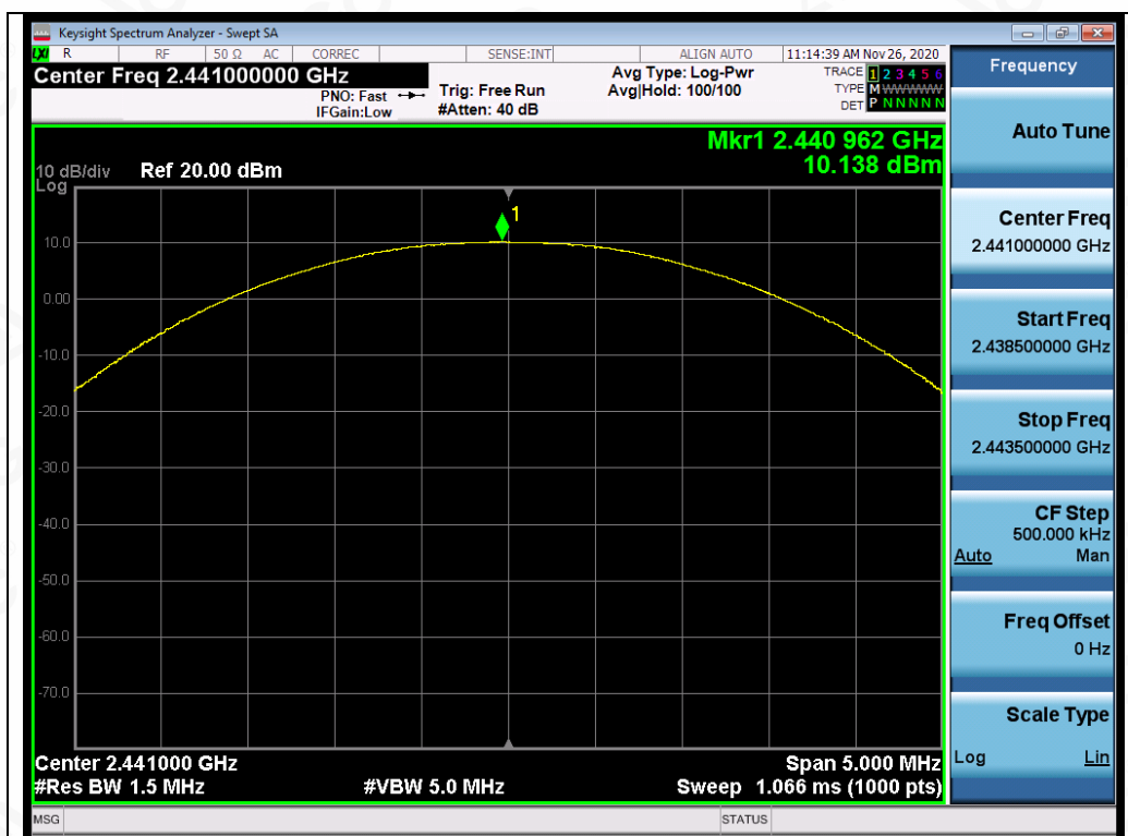
Test_Graph_EDR_2441_3Mbps_Peak Power
