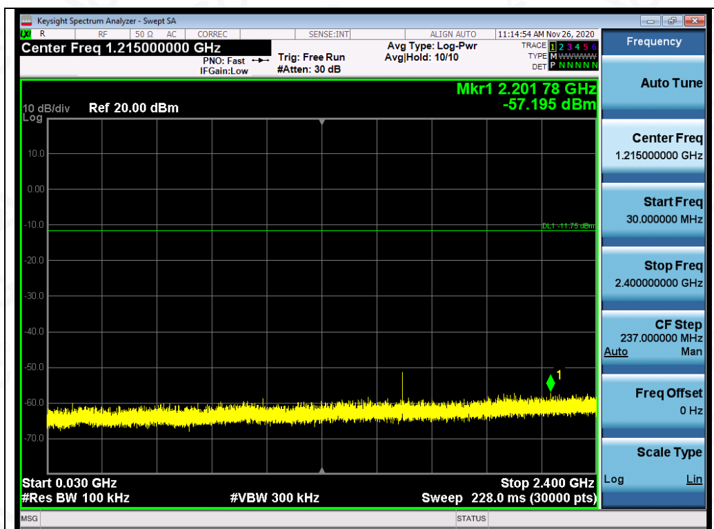
Test_Graph_EDR_2441_3Mbps_Lower Band Emissions
