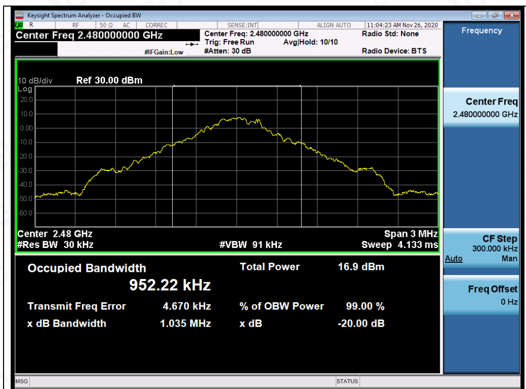
Test_Graph_BR_2480_1Mbps_OBW
