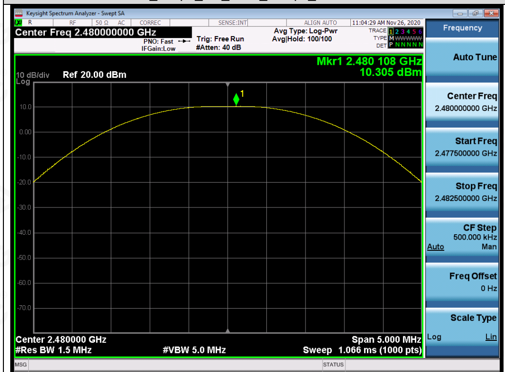
Test_Graph_BR_2480_1Mbps_Peak Power
