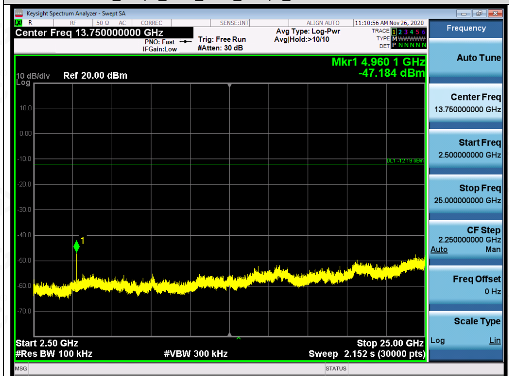
Test_Graph_EDR_2480_2Mbps_Higher Band Emissions
