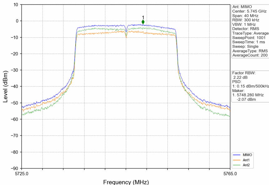
802.11ax(HEW20)_LCH_5745MHz_RU242_Left_MIMO_NTNV
