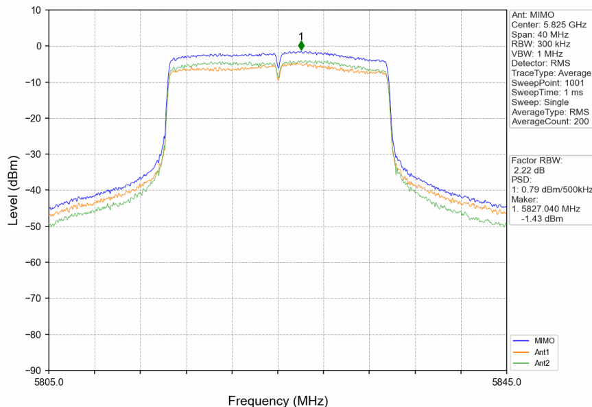
802.11ax(HEW20)_HCH_5825MHz_RU242_Left_MIMO_NTNV
