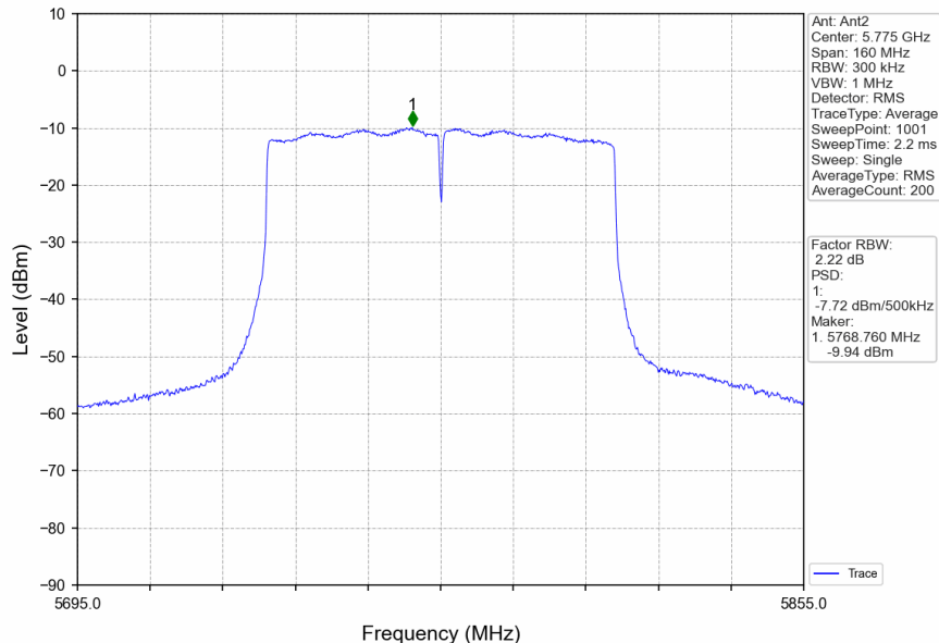
802.11ac(VHT80)_MCH_5775MHz_Ant2_NTNV
