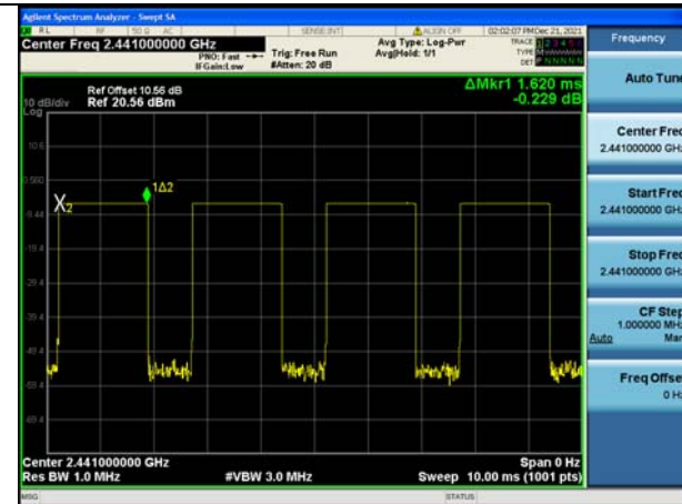
Test Mode:GFSK(DH5) 2441MHz
