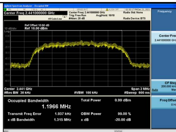
Test Mode:8DPSK(3DH5) MHz
