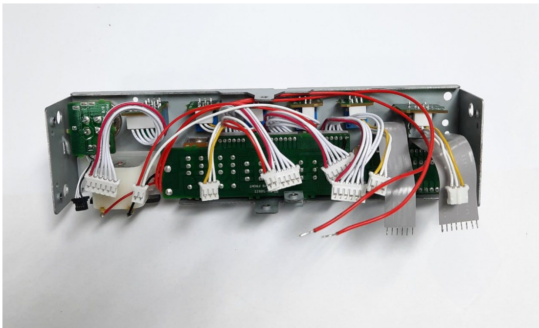
Front Assembly 1
