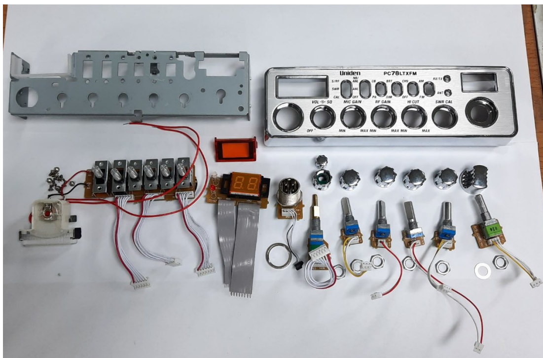
Front Assembly 3
