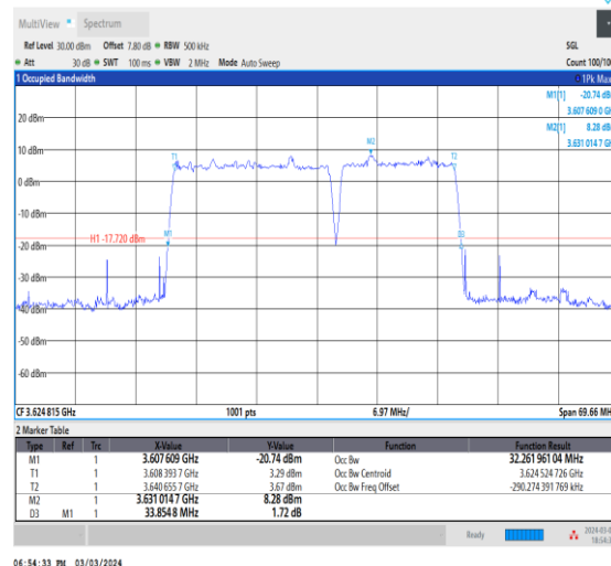
NTNV_CA_n48B_PC3_30+30_20+15_M+M_Ant0_TID3_1_#1
