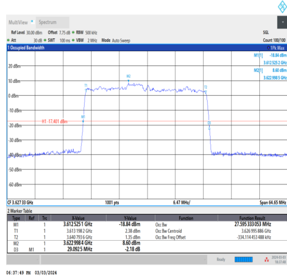
NTNV_CA_n48B_PC3_30+30_15+20_M+M_Ant0_TID3_1_#1
