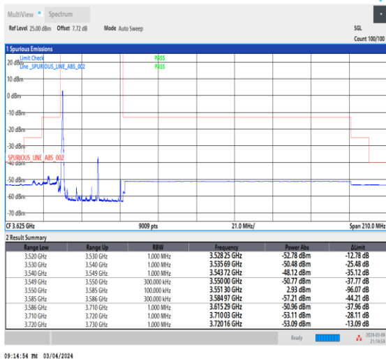
NTNV_CA_n48B_PC3_30+30_20+15_L+L_TID4_1_#1
