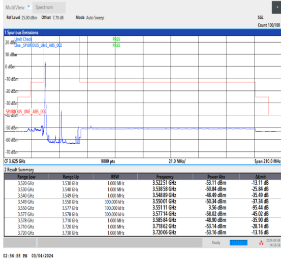
NTNV_CA_n48B_PC3_30+30_15+15_L+L_TID1_1_#1
