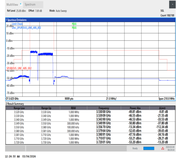
NTNV_CA_n48B_PC3_30+30_10+20_L+L_TID3_1_#1
