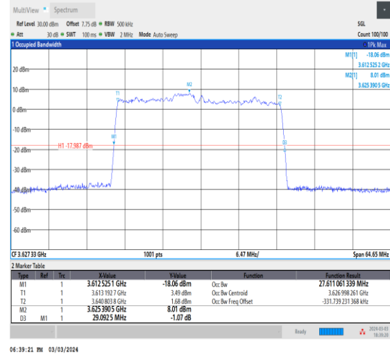
NTNV_CA_n48B_PC3_30+30_15+20_M+M_Ant0_TID9_1_#1
