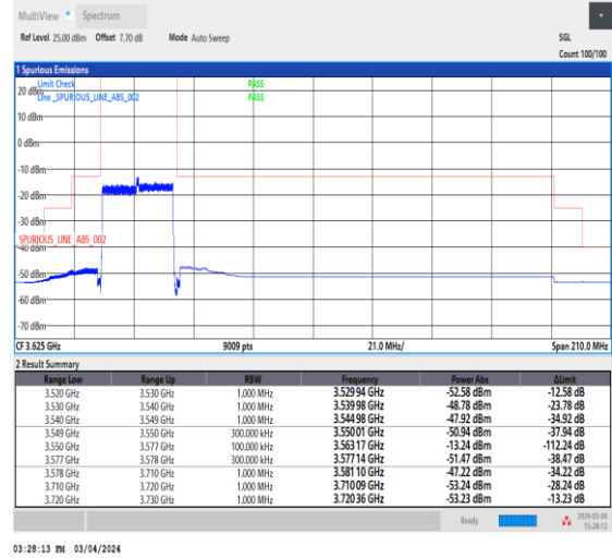
NTNV_CA_n48B_PC3_30+30_15+15_L+L_TID3_1_#1
