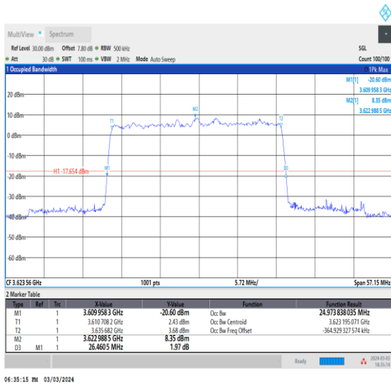
NTNV_CA_n48B_PC3_30+30_15+15_M+M_Ant0_TID9_1_#1
