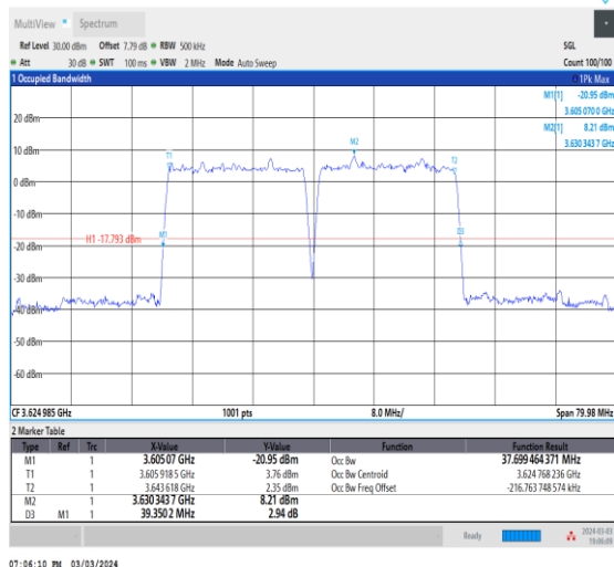
NTNV_CA_n48B_PC3_30+30_20+20_M+M_Ant0_TID5_1_#1
