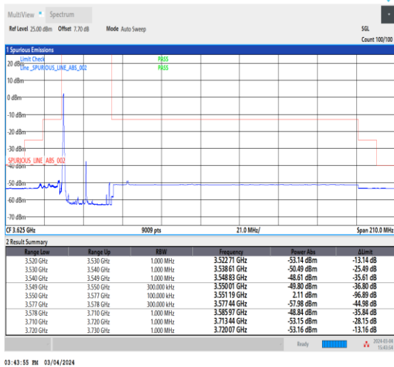
NTNV_CA_n48B_PC3_30+30_15+15_L+L_TID4_1_#1
