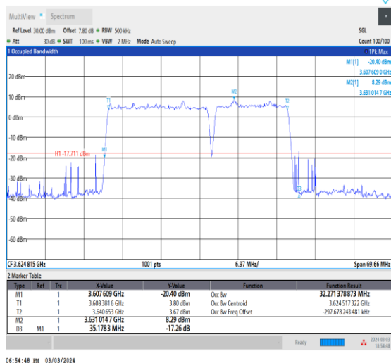
NTNV_CA_n48B_PC3_30+30_20+15_M+M_Ant0_TID4_1_#1
