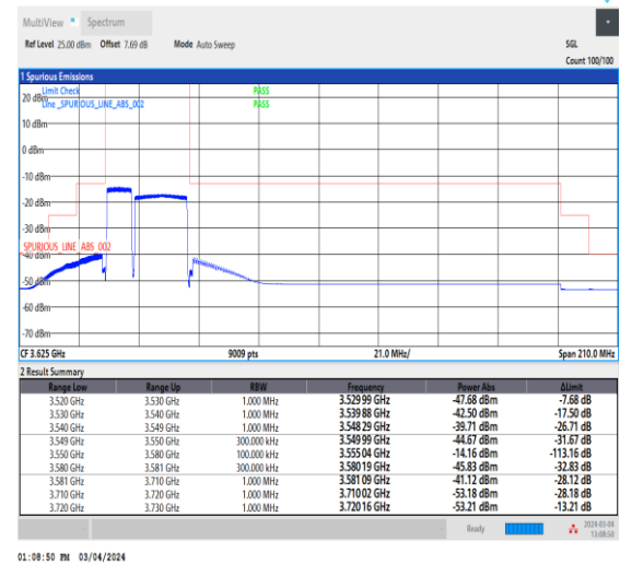
NTNV_CA_n48B_PC3_30+30_10+20_L+L_TID6_1_#1
