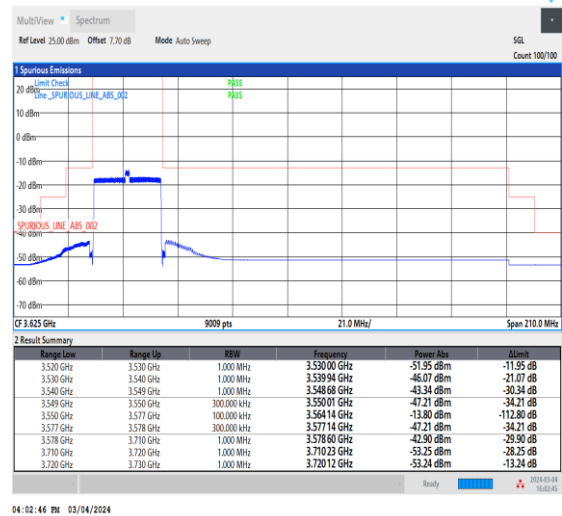
NTNV_CA_n48B_PC3_30+30_15+15_L+L_TID6_1_#1
