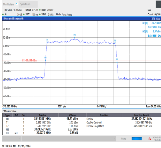
NTNV_CA_n48B_PC3_30+30_15+20_M+M_Ant0_TID8_1_#1
