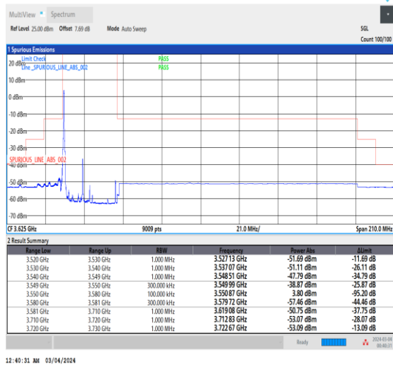
NTNV_CA_n48B_PC3_30+30_10+20_L+L_TID4_1_#1
