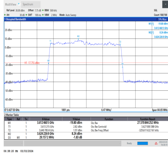
NTVN_CA_n48B_PC3_30+30_15+20_M+M_Ant0_TID5_1_#1
