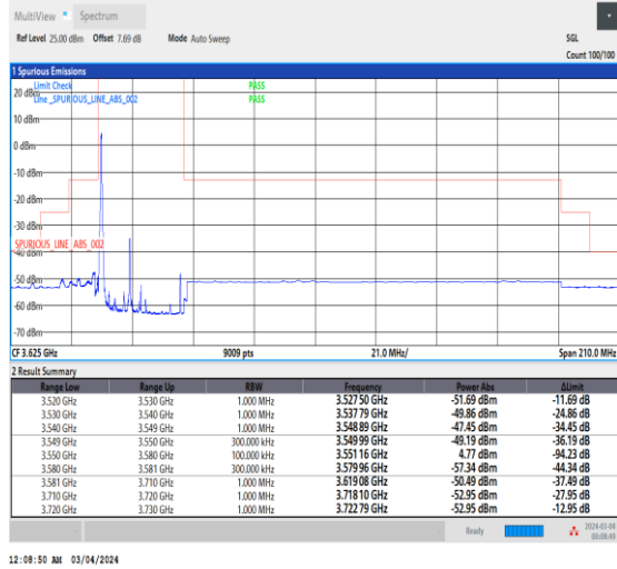
NTNV_CA_n48B_PC3_30+30_10+20_L+L_TID1_1_#1
