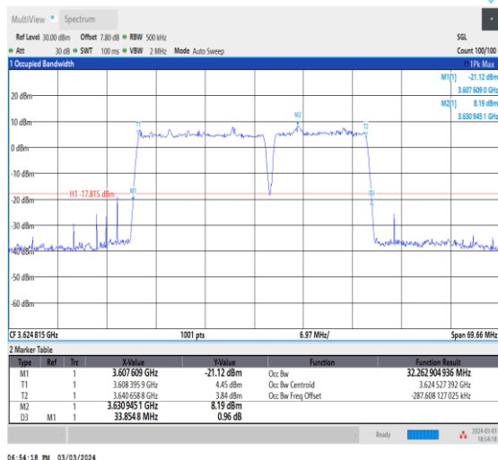
NTNV_CA_n48B_PC3_30+30_20+15_M+M_Ant0_TID2_1_#1
