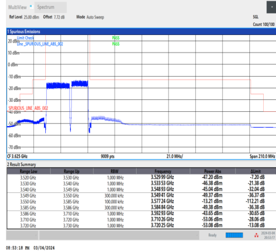
NTNV_CA_n48B_PC3_30+30_20+15_L+L_TID3_1_#1
