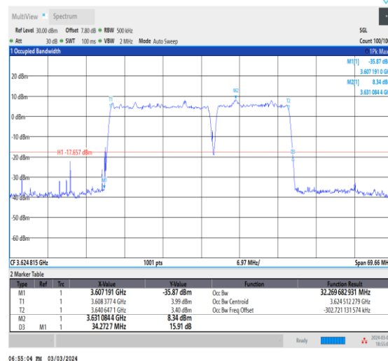
NTNV_CA_n48B_PC3_30+30_20+15_M+M_Ant0_TID5_1_#1
