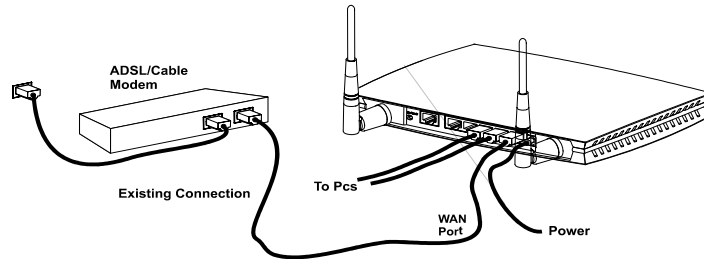
Figure 4: Installation Diagram
