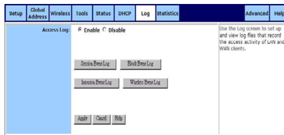
Figure 31: Log Screen
