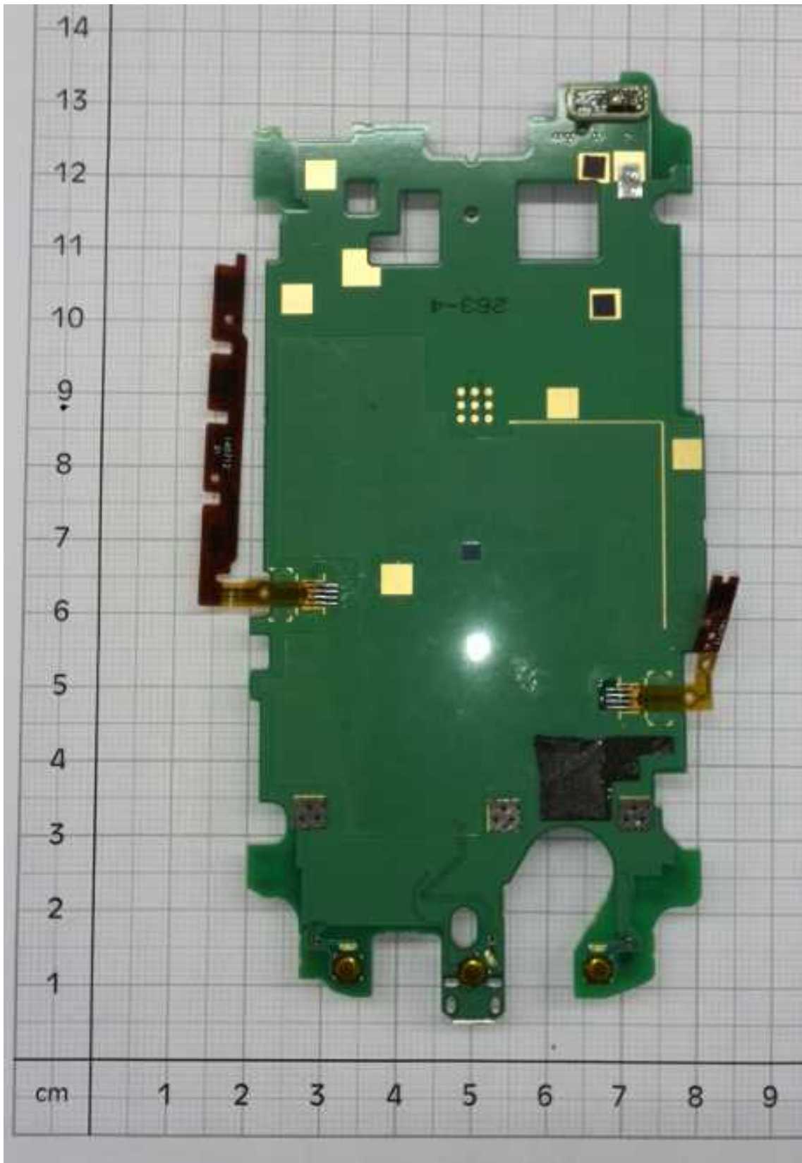
Main PCB rear
