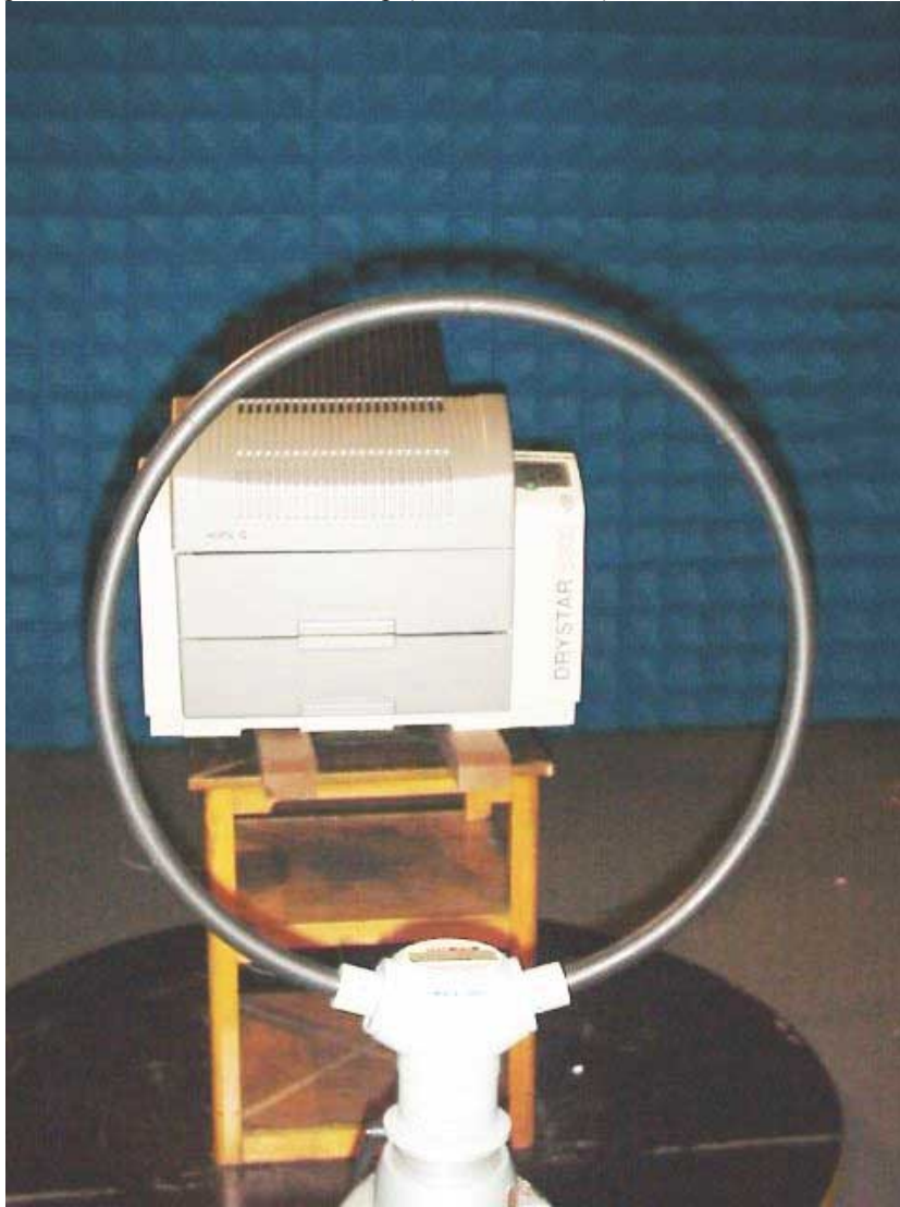
photo 6 : radiated emission set-up (band 13.56MHz)
