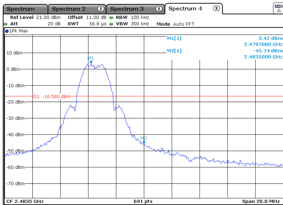
Channel 16: 2.480 GHz
